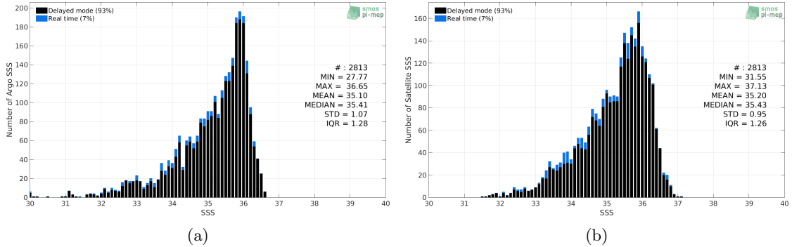
Figure 2: Histograms of SSS from Argo (a) and SMAP SSS L4 OI v1 - 7 Days (IPRC) (b) considering all match-up pairs per bins of 0.1 over the Congo river plume Pi-MEP region and for the full satellite product period.
