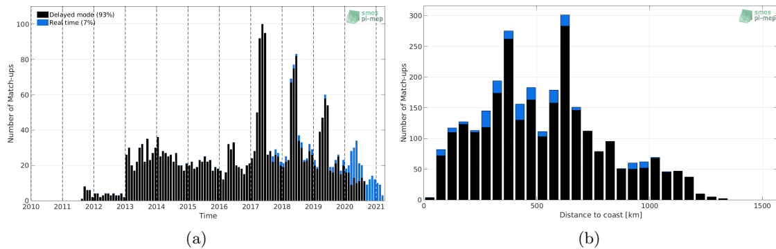
Figure 1: Number of match-ups between Argo and SMAP SSS L4 OI v1 - 7 Days (IPRC) SSS as a function of time (a) and as function of the distance to coast (b) over the Congo river plume Pi-MEP region and for the full satellite product period.
