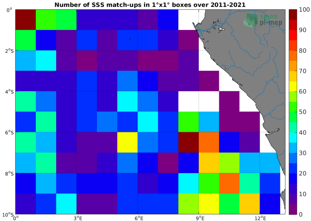
Figure 4: Number of SSS match-ups between Argo SSS and the SMAP SSS L4 OI v1 - 7 Days (IPRC) SSS product for the Congo river plume Pi-MEP region over 1^\circ \times 1^\circ boxes and for the full satellite product period.
