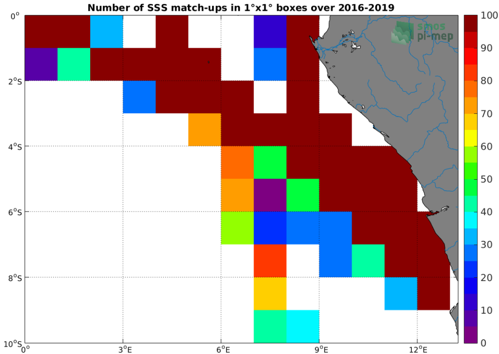
Figure 4: Number of SSS match-ups between TSG (LEGOS-DM) SSS and the SMAP SSS L4 OI v1 - Monthly (IPRC) SSS product for the Congo river plume Pi-MEP region over 1^{\circ} \times 1^{\circ} boxes and for the full satellite product period.
