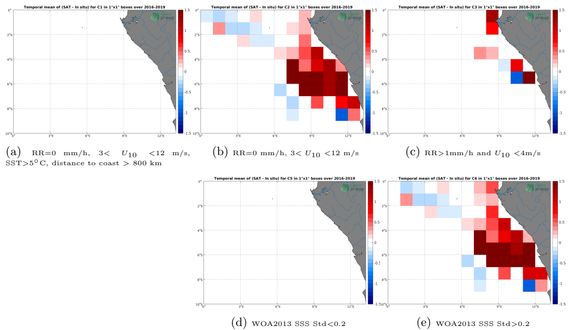
Figure 12: Temporal mean gridded over spatial boxes of size 1^\circ \times 1^\circ of \Delta SSS (SMAP SSS L4 OI v1 - Monthly (IPRC) - TSG (LEGOS-DM)) for 5 different subdatasets corresponding to:RR=0 mm/h, 3 < U_{10} < 12 m/s, SST >5^\circ\text{C} , distance to coast > 800 km (a), RR=0 mm/h, 3 < U_{10} < 12 m/s (b), RR >1 mm/h and U_{10} < 4 m/s (c), WOA2013 SSS Std <0.2 (d), WOA2013 SSS Std >0.2 (e).
