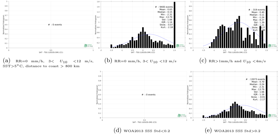
Figure 13: Normalized histogram of \Delta\text{SSS} (SMAP SSS L4 OI v1 - Monthly (IPRC) - TSG (LEGOS-DM)) for 5 different subdatasets corresponding to: RR=0 mm/h, 3 < U_{10} < 12 m/s, SST > 5^\circ\text{C} , distance to coast > 800 km (a), RR=0 mm/h, 3 < U_{10} < 12 m/s (b), RR > 1 mm/h and U_{10} < 4 m/s (c), WOA2013 SSS Std <0.2 (d), WOA2013 SSS Std >0.2 (e).
