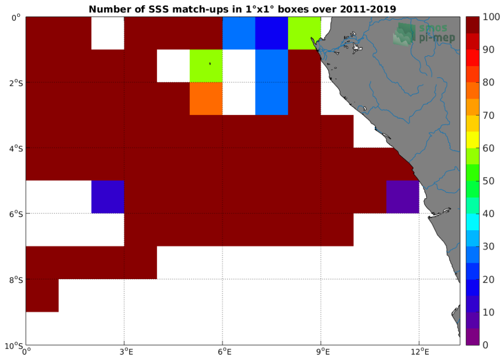
Figure 4: Number of SSS match-ups between TSG (GOSUD-Research-vessel) SSS and the SMAP SSS L4 OI v1 - Monthly (IPRC) SSS product for the Congo river plume Pi-MEP region over 1^\circ \times 1^\circ boxes and for the full satellite product period.
