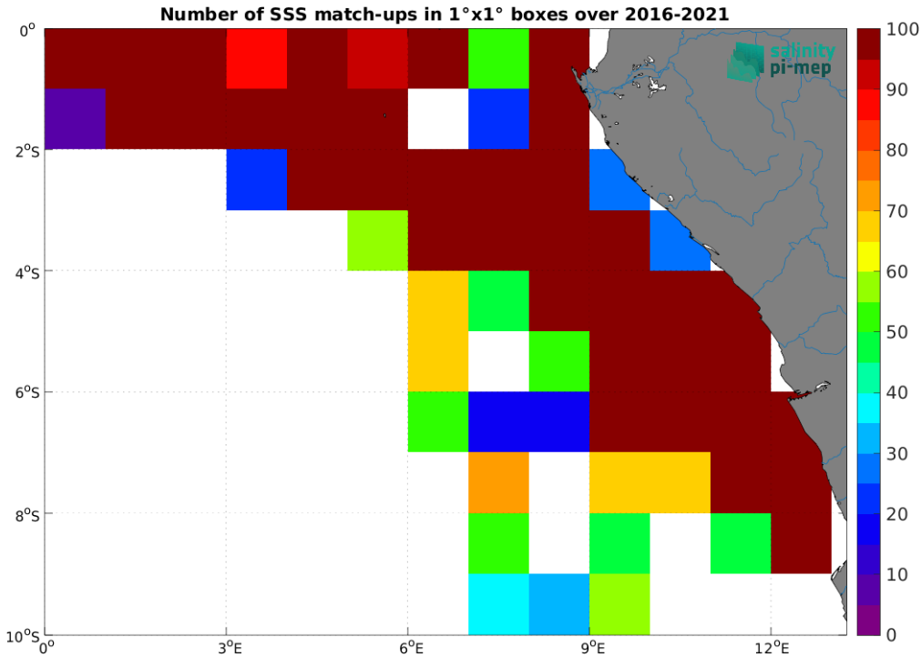
Figure 5: Number of SSS match-ups between TSG (LEGOS-DM) SSS and the SMAP SSS L4 OI v3 - Monthly (ESR) SSS product for the Congo river plume Pi-MEP region over 1^{\circ} \times 1^{\circ} boxes and for the full satellite product period.
