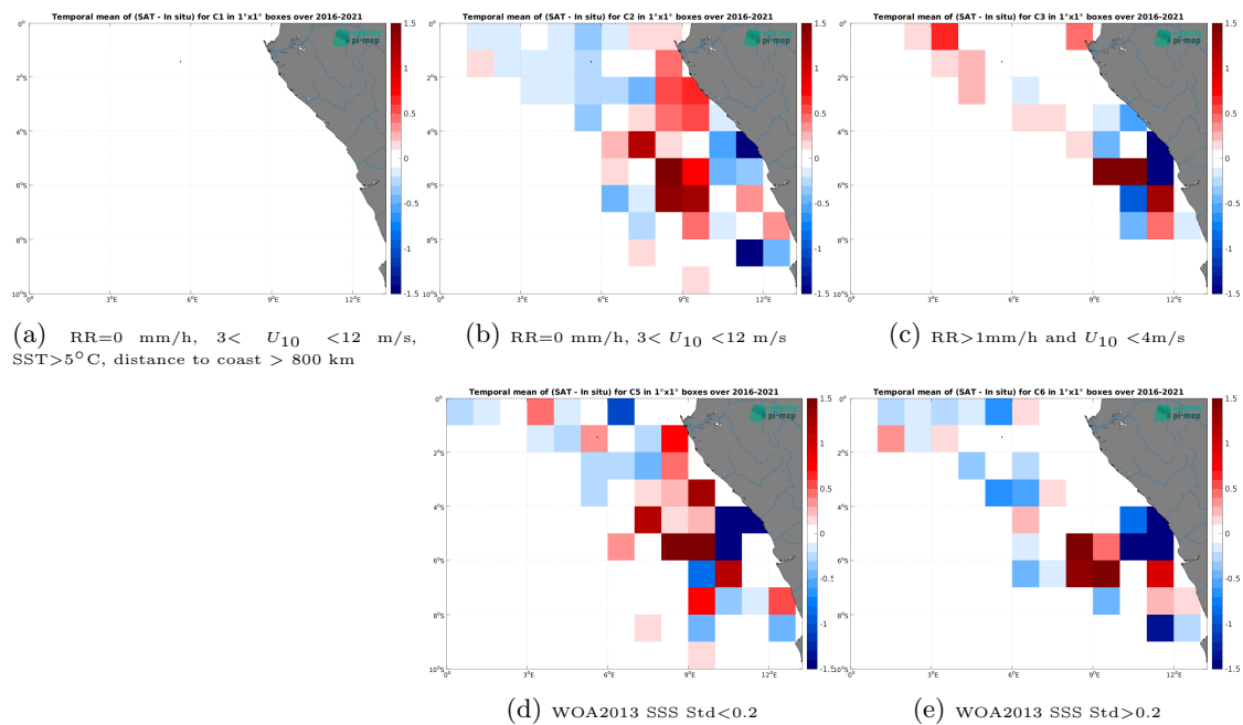
Figure 14: Temporal mean gridded over spatial boxes of size 1^\circ \times 1^\circ of \Delta SSS (SMAP SSS L4 OI v3 - Monthly (ESR) - TSG (LEGOS-DM)) for 5 different subdatasets corresponding to:RR=0 mm/h, 3 < U_{10} < 12 m/s, SST >5^\circ C, distance to coast > 800 km (a), RR=0 mm/h, 3 < U_{10} < 12 m/s (b), RR >1 mm/h and U_{10} < 4 m/s (c), WOA2013 SSS Std <0.2 (d), WOA2013 SSS Std >0.2 (e).
