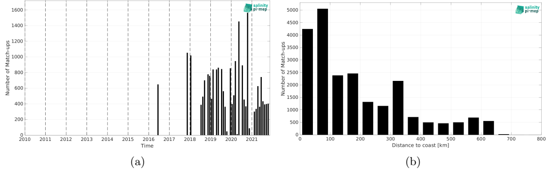
Figure 2: Number of match-ups between TSG (LEGOS-DM) and SMAP SSS L4 OI v3 - Monthly (ESR) SSS as a function of time (a) and as function of the distance to coast (b) over the Congo river plume Pi-MEP region and for the full satellite product period.
