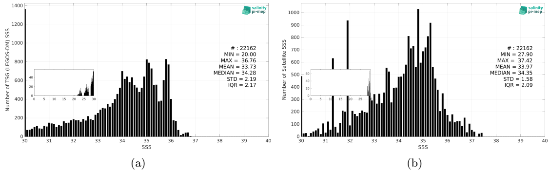
Figure 3: Histograms of SSS from TSG (LEGOS-DM) (a) and SMAP SSS L4 OI v3 - Monthly (ESR) (b) considering all match-up pairs per bins of 0.1 over the Congo river plume Pi-MEP region and for the full satellite product period.
