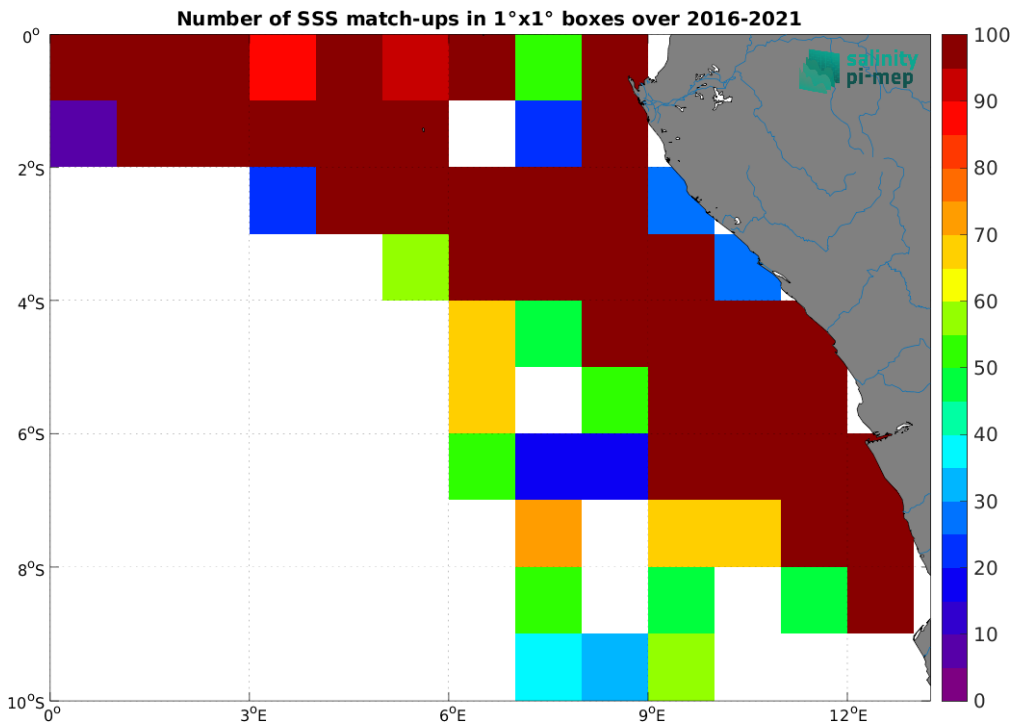
Figure 5: Number of SSS match-ups between TSG (LEGOS-DM) SSS and the SMAP SSS L4 OI v3 - Monthly (ESR) SSS product for the Congo river plume Pi-MEP region over 1^\circ \times 1^\circ boxes and for the full satellite product period.
