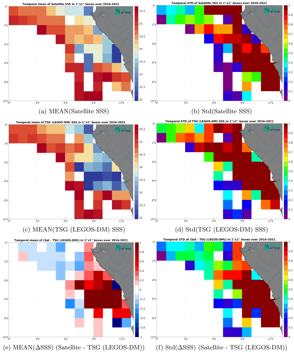
Figure 7: Temporal mean (left) and Std (right) of SSS from SMAP SSS L4 OI v3 - Monthly (ESR) (top), TSG (LEGOS-DM) (middle), and of \Delta SSS (Satellite - TSG (LEGOS-DM)). Only match-up pairs are used to generate these maps.
