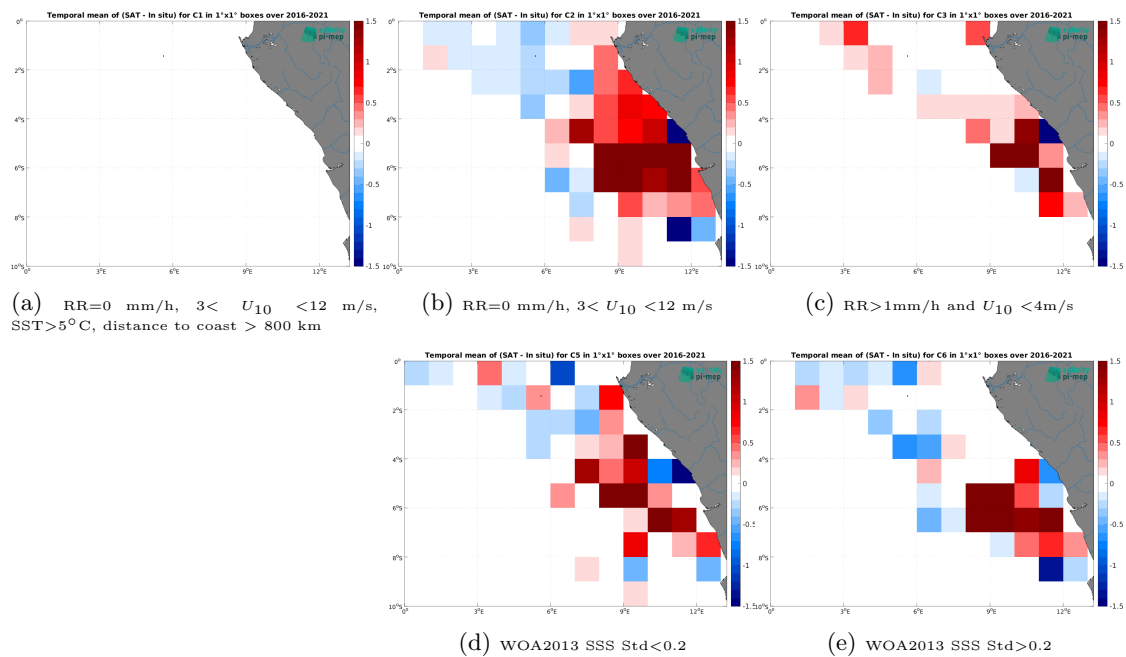
Figure 14: Temporal mean gridded over spatial boxes of size 1^\circ \times 1^\circ of \Delta\text{SSS} (SMAP SSS L4 OI v3 - Monthly (ESR) - TSG (LEGOS-DM)) for 5 different subdatasets corresponding to: RR=0 mm/h, 3 < U_{10} < 12 m/s, SST > 5°C, distance to coast > 800 km (a), RR=0 mm/h, 3 < U_{10} < 12 m/s (b), RR > 1mm/h and U_{10} < 4 m/s (c), WOA2013 SSS Std < 0.2 (d), WOA2013 SSS Std > 0.2 (e).
