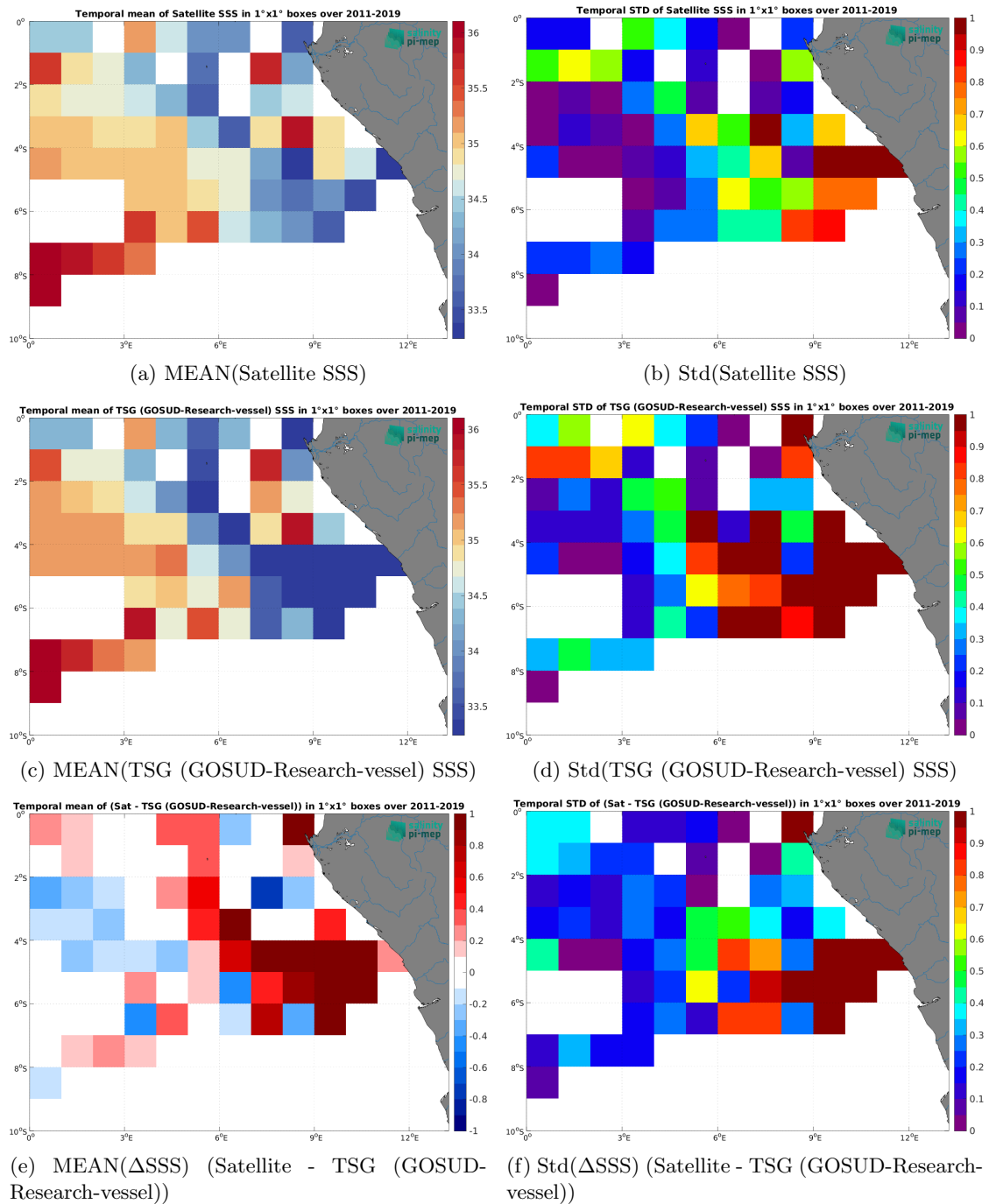
Figure 7: Temporal mean (left) and Std (right) of SSS from SMAP SSS L4 OI v3 - Monthly (ESR) (top), TSG (GOSUD-Research-vessel) (middle), and of \Delta SSS (Satellite - TSG (GOSUD-Research-vessel)). Only match-up pairs are used to generate these maps.
