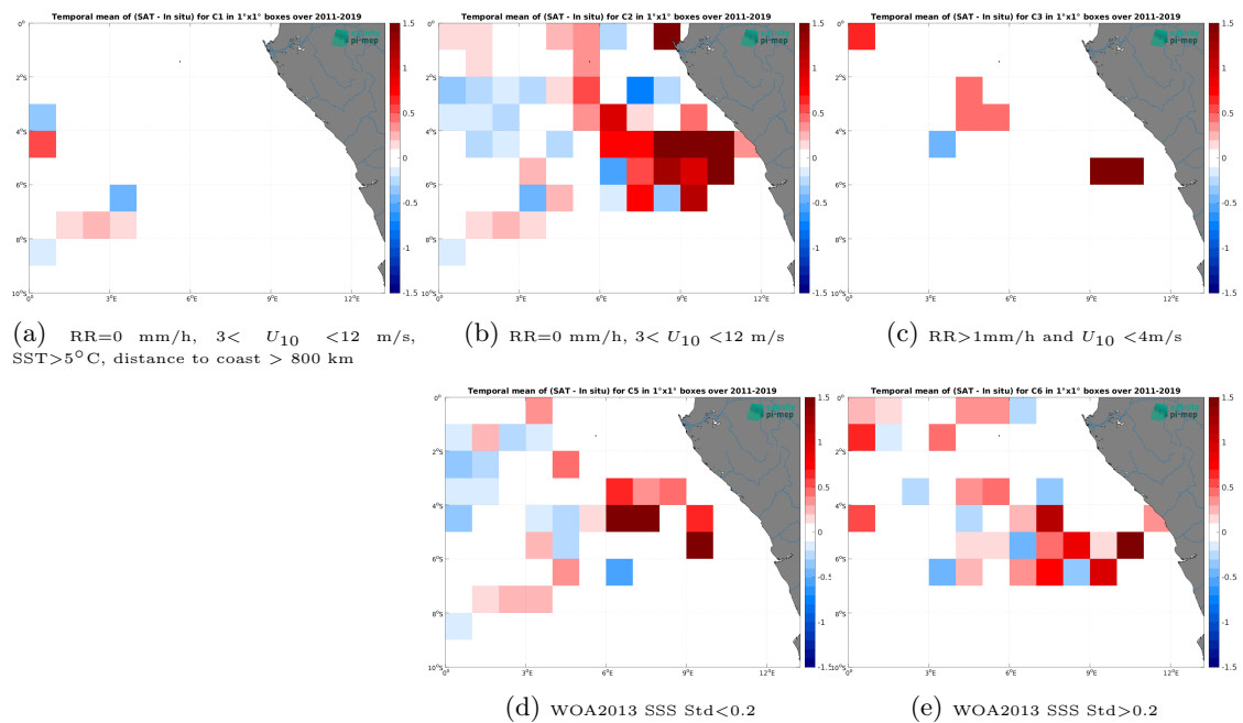
Figure 14: Temporal mean gridded over spatial boxes of size 1^\circ \times 1^\circ of \Delta SSS (SMAP SSS L4 OI v3 - Monthly (ESR) - TSG (GOSUD-Research-vessel)) for 5 different subdatasets corresponding to:RR=0 mm/h, 3 < U_{10} < 12 m/s, SST>5°C, distance to coast > 800 km (a), RR=0 mm/h, 3 < U_{10} < 12 m/s (b), RR>1mm/h and U_{10} < 4 m/s (c), WOA2013 SSS Std<0.2 (d), WOA2013 SSS Std>0.2 (e).
