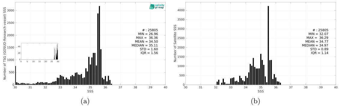
Figure 3: Histograms of SSS from TSG (GOSUD-Research-vessel) (a) and SMAP SSS L4 OI v3 - Monthly (ESR) (b) considering all match-up pairs per bins of 0.1 over the Congo river plume Pi-MEP region and for the full satellite product period.
