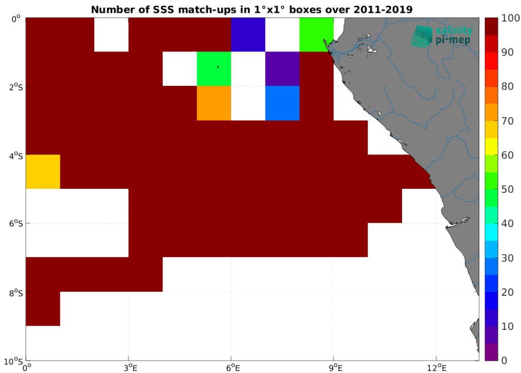
Figure 5: Number of SSS match-ups between TSG (GOSUD-Research-vessel) SSS and the SMAP SSS L4 OI v3 - Monthly (ESR) SSS product for the Congo river plume Pi-MEP region over 1^\circ \times 1^\circ boxes and for the full satellite product period.
