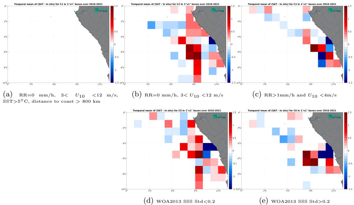
Figure 14: Temporal mean gridded over spatial boxes of size 1^\circ \times 1^\circ of \Delta SSS (SMAP SSS L4 OI v3 - Daily (ESR) - TSG (LEGOS-DM)) for 5 different subdatasets corresponding to: RR=0 mm/h, 3 < U_{10} < 12 m/s, SST > 5°C, distance to coast > 800 km (a), RR=0 mm/h, 3 < U_{10} < 12 m/s (b), RR > 1 mm/h and U_{10} < 4 m/s (c), WOA2013 SSS Std < 0.2 (d), WOA2013 SSS Std > 0.2 (e).
