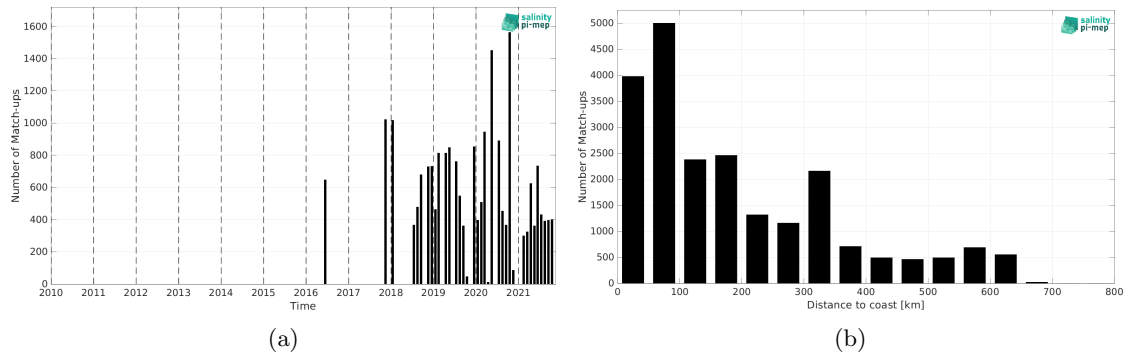
Figure 2: Number of match-ups between TSG (LEGOS-DM) and SMAP SSS L4 OI v3 - Daily (ESR) SSS as a function of time (a) and as function of the distance to coast (b) over the Congo river plume Pi-MEP region and for the full satellite product period.
