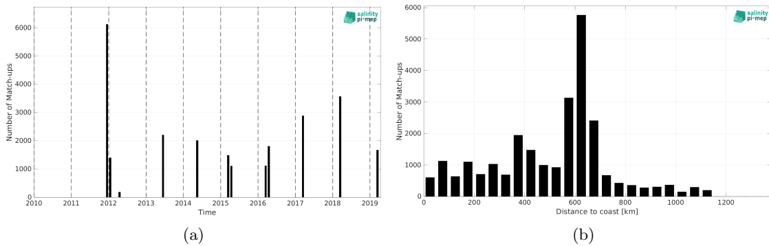
Figure 2: Number of match-ups between TSG (GOSUD-Research-vessel) and SMAP SSS L4 OI v3 - Daily (ESR) SSS as a function of time (a) and as function of the distance to coast (b) over the Congo river plume Pi-MEP region and for the full satellite product period.
