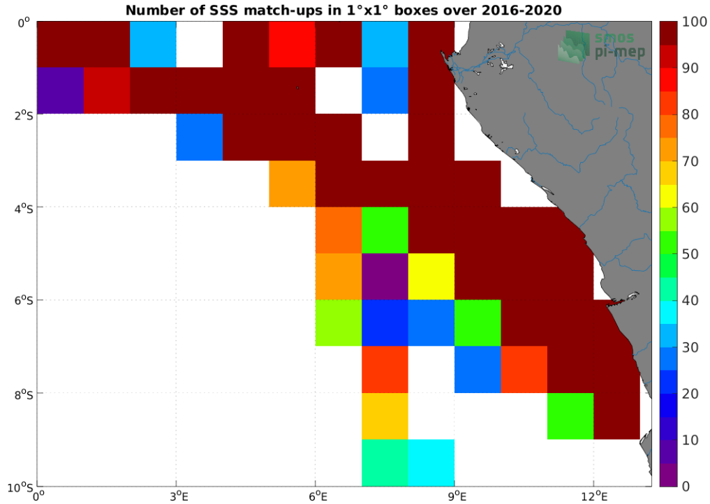
Figure 4: Number of SSS match-ups between TSG (LEGOS-DM) SSS and the SMAP SSS L4 OI v2 - Monthly (IPRC) SSS product for the Congo river plume Pi-MEP region over 1^\circ \times 1^\circ boxes and for the full satellite product period.
