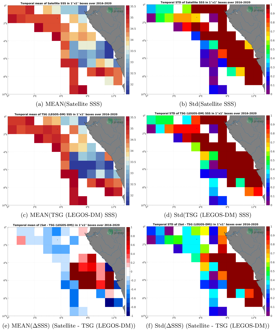
Figure 6: Temporal mean (left) and Std (right) of SSS from SMAP SSS L4 OI v2 - Monthly (IPRC) (top), TSG (LEGOS-DM) (middle), and of \Delta SSS (Satellite - TSG (LEGOS-DM)). Only match-up pairs are used to generate these maps.
