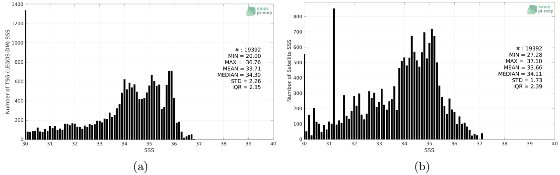
Figure 2: Histograms of SSS from TSG (LEGOS-DM) (a) and SMAP SSS L4 OI v2 - Monthly (IPRC) (b) considering all match-up pairs per bins of 0.1 over the Congo river plume Pi-MEP region and for the full satellite product period.
