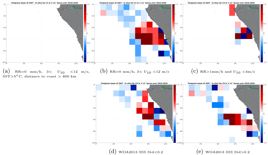
Figure 12: Temporal mean gridded over spatial boxes of size 1^\circ \times 1^\circ of \Delta SSS (SMAP SSS L4 OI v2 - Monthly (IPRC) - TSG (LEGOS-DM)) for 5 different subdatasets corresponding to:RR=0 mm/h, 3 < U_{10} < 12 m/s, SST >5^\circ C, distance to coast > 800 km (a), RR=0 mm/h, 3 < U_{10} < 12 m/s (b), RR >1 mm/h and U_{10} < 4 m/s (c), WOA2013 SSS Std <0.2 (d), WOA2013 SSS Std >0.2 (e).
