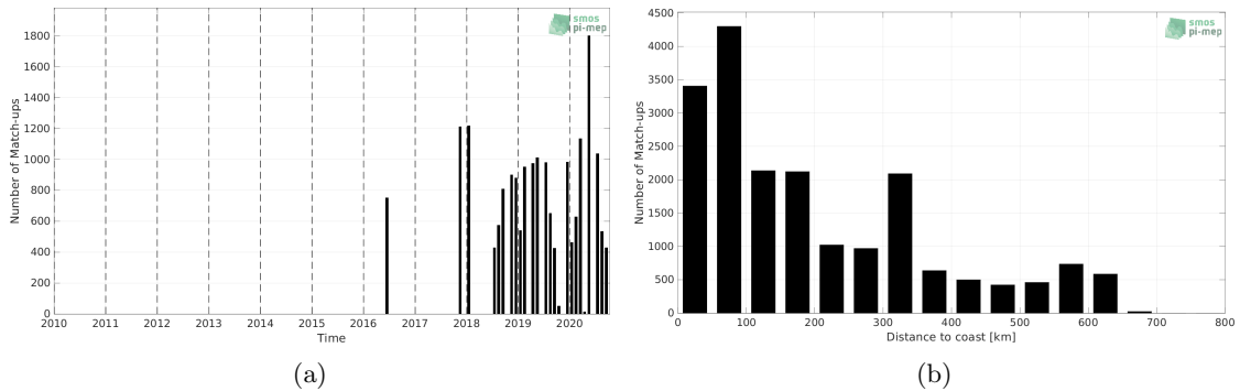
Figure 1: Number of match-ups between TSG (LEGOS-DM) and SMAP SSS L4 OI v2 - Monthly (IPRC) SSS as a function of time (a) and as function of the distance to coast (b) over the Congo river plume Pi-MEP region and for the full satellite product period.
