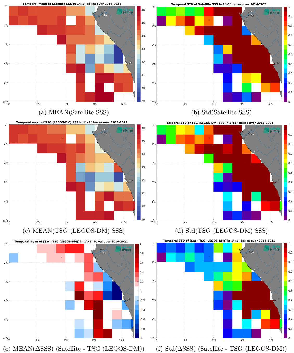
Figure 7: Temporal mean (left) and Std (right) of SSS from SMAP SSS L3 v6 - 8-Day running (RSS) (top), TSG (LEGOS-DM) (middle), and of \Delta SSS (Satellite - TSG (LEGOS-DM)). Only match-up pairs are used to generate these maps.
