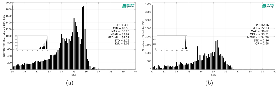
Figure 3: Histograms of SSS from TSG (LEGOS-DM) (a) and SMAP SSS L3 v6 - 8-Day running (RSS) (b) considering all match-up pairs per bins of 0.1 over the Congo river plume Pi-MEP region and for the full satellite product period.
