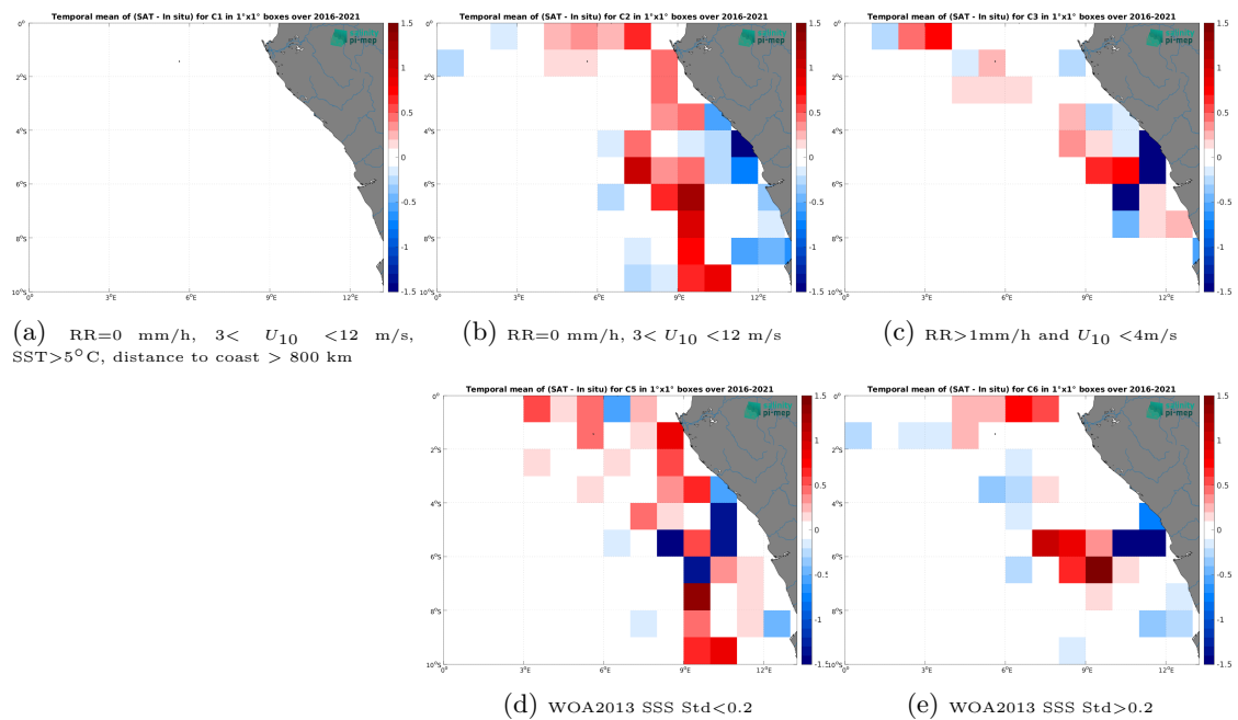
Figure 14: Temporal mean gridded over spatial boxes of size 1^\circ \times 1^\circ of \Delta SSS (SMAP SSS L3 v6 - 8-Day running (RSS) - TSG (LEGOS-DM)) for 5 different subdatasets corresponding to: RR=0 mm/h, 3 < U_{10} < 12 m/s, SST > 5°C, distance to coast > 800 km (a), RR=0 mm/h, 3 < U_{10} < 12 m/s (b), RR > 1mm/h and U_{10} < 4 m/s (c), WOA2013 SSS Std < 0.2 (d), WOA2013 SSS Std > 0.2 (e).
