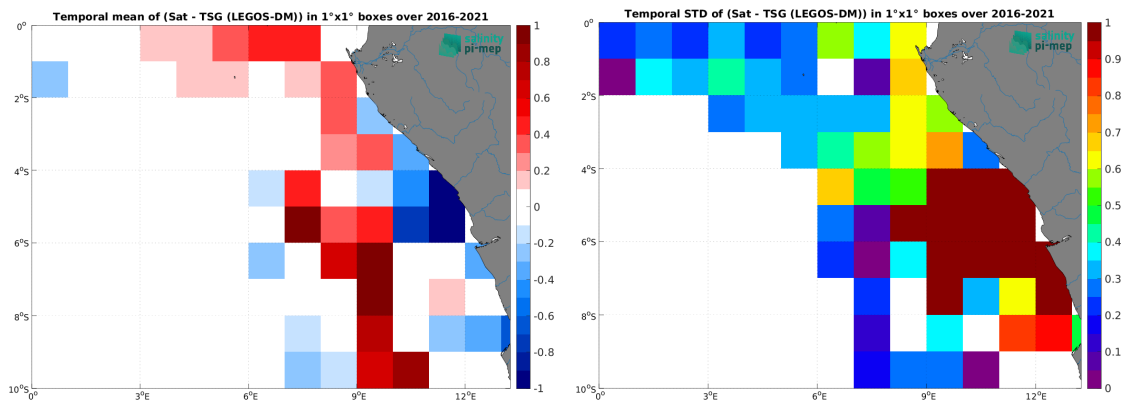
(e) MEAN( \Delta SSS) (Satellite - TSG (LEGOS-DM)) (f) Std( \Delta SSS) (Satellite - TSG (LEGOS-DM))
