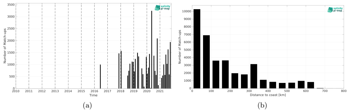
Figure 2: Number of match-ups between TSG (LEGOS-DM) and SMAP SSS L3 v6 - 8-Day running (RSS) SSS as a function of time (a) and as function of the distance to coast (b) over the Congo river plume Pi-MEP region and for the full satellite product period.
