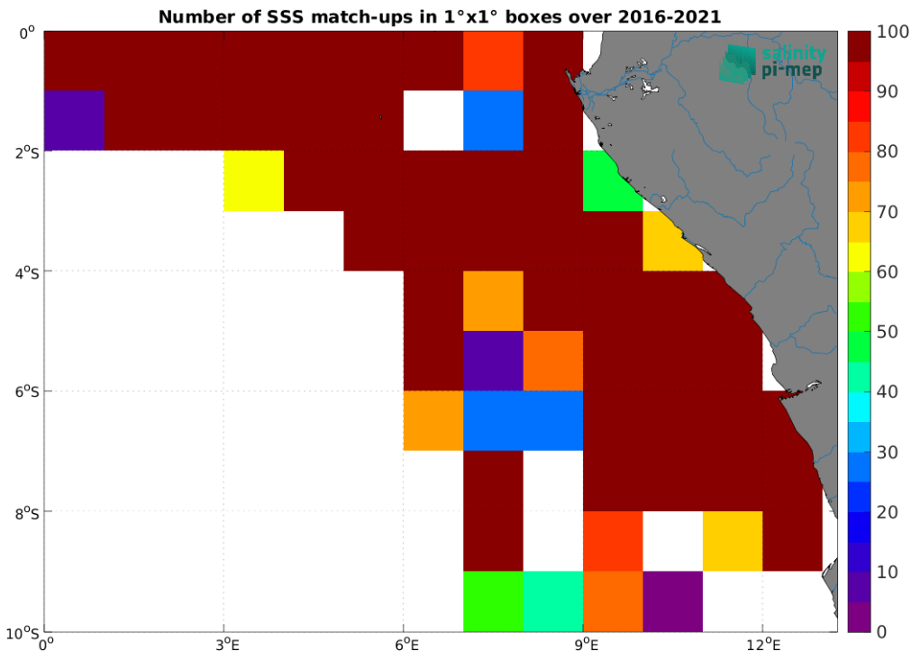
Figure 5: Number of SSS match-ups between TSG (LEGOS-DM) SSS and the SMAP SSS L3 v6 - 8-Day running (RSS) SSS product for the Congo river plume Pi-MEP region over 1^\circ \times 1^\circ boxes and for the full satellite product period.
