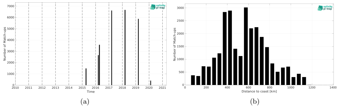
Figure 2: Number of match-ups between TSG (GOSUD-Research-vessel) and SMAP SSS L3 v6 - 8-Day running (RSS) SSS as a function of time (a) and as function of the distance to coast (b) over the Congo river plume Pi-MEP region and for the full satellite product period.
