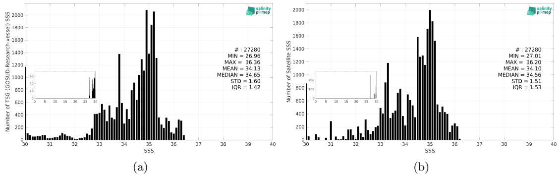
Figure 3: Histograms of SSS from TSG (GOSUD-Research-vessel) (a) and SMAP SSS L3 v6 - 8-Day running (RSS) (b) considering all match-up pairs per bins of 0.1 over the Congo river plume Pi-MEP region and for the full satellite product period.
