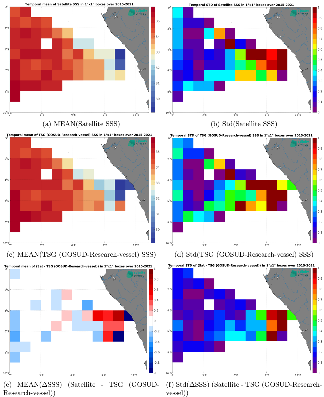
Figure 7: Temporal mean (left) and Std (right) of SSS from SMAP SSS L3 v6 - 8-Day running (RSS) (top), TSG (GOSUD-Research-vessel) (middle), and of \Delta SSS (Satellite - TSG (GOSUD-Research-vessel)). Only match-up pairs are used to generate these maps.
