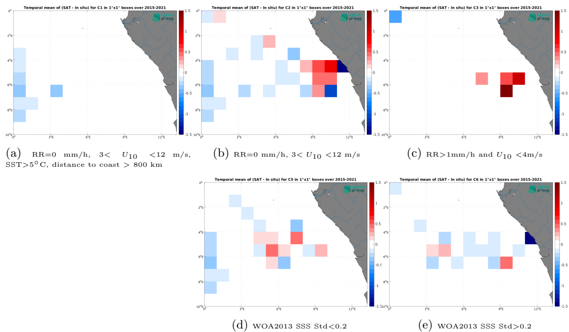
Figure 14: Temporal mean gridded over spatial boxes of size 1^\circ \times 1^\circ of \Delta\text{SSS} (SMAP SSS L3 v6 - 8-Day running (RSS) - TSG (GOSUD-Research-vessel)) for 5 different subdatasets corresponding to:RR=0 mm/h, 3 < U_{10} < 12 m/s, SST >5^\circ\text{C} , distance to coast > 800 km (a), RR=0 mm/h, 3 < U_{10} < 12 m/s (b), RR >1 mm/h and U_{10} < 4 m/s (c), WOA2013 SSS Std <0.2 (d), WOA2013 SSS Std >0.2 (e).
