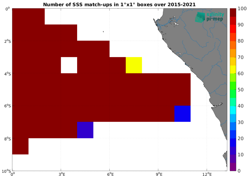
Figure 5: Number of SSS match-ups between TSG (GOSUD-Research-vessel) SSS and the SMAP SSS L3 v6 - 8-Day running (RSS) SSS product for the Congo river plume Pi-MEP region over 1^\circ \times 1^\circ boxes and for the full satellite product period.
