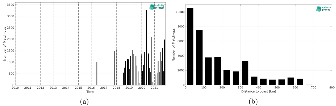
Figure 2: Number of match-ups between TSG (LEGOS-DM) and SMAP SSS L3 v6 - Monthly (RSS) SSS as a function of time (a) and as function of the distance to coast (b) over the Congo river plume Pi-MEP region and for the full satellite product period.
