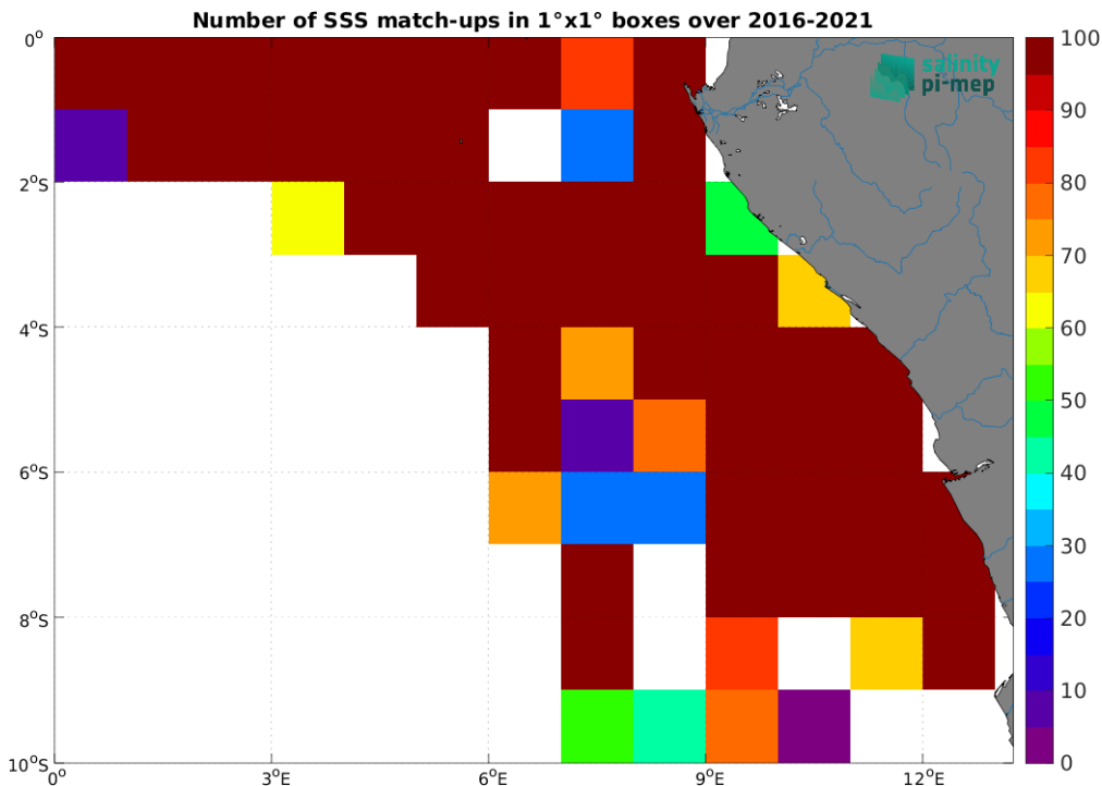
Figure 5: Number of SSS match-ups between TSG (LEGOS-DM) SSS and the SMAP SSS L3 v6 - Monthly (RSS) SSS product for the Congo river plume Pi-MEP region over 1^\circ \times 1^\circ boxes and for the full satellite product period.
