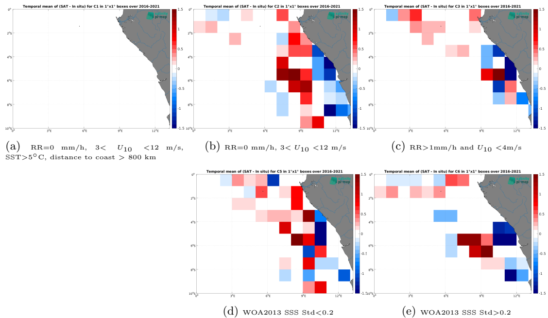
Figure 14: Temporal mean gridded over spatial boxes of size 1^\circ \times 1^\circ of \Delta SSS (SMAP SSS L3 v6 - Monthly (RSS) - TSG (LEGOS-DM)) for 5 different subdatasets corresponding to:RR=0 mm/h, 3 < U_{10} < 12 m/s, SST>5°C, distance to coast > 800 km (a), RR=0 mm/h, 3 < U_{10} < 12 m/s (b), RR>1mm/h and U_{10} < 4 m/s (c), WOA2013 SSS Std<0.2 (d), WOA2013 SSS Std>0.2 (e).
