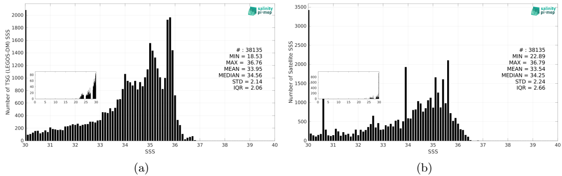
Figure 3: Histograms of SSS from TSG (LEGOS-DM) (a) and SMAP SSS L3 v6 - Monthly (RSS) (b) considering all match-up pairs per bins of 0.1 over the Congo river plume Pi-MEP region and for the full satellite product period.
