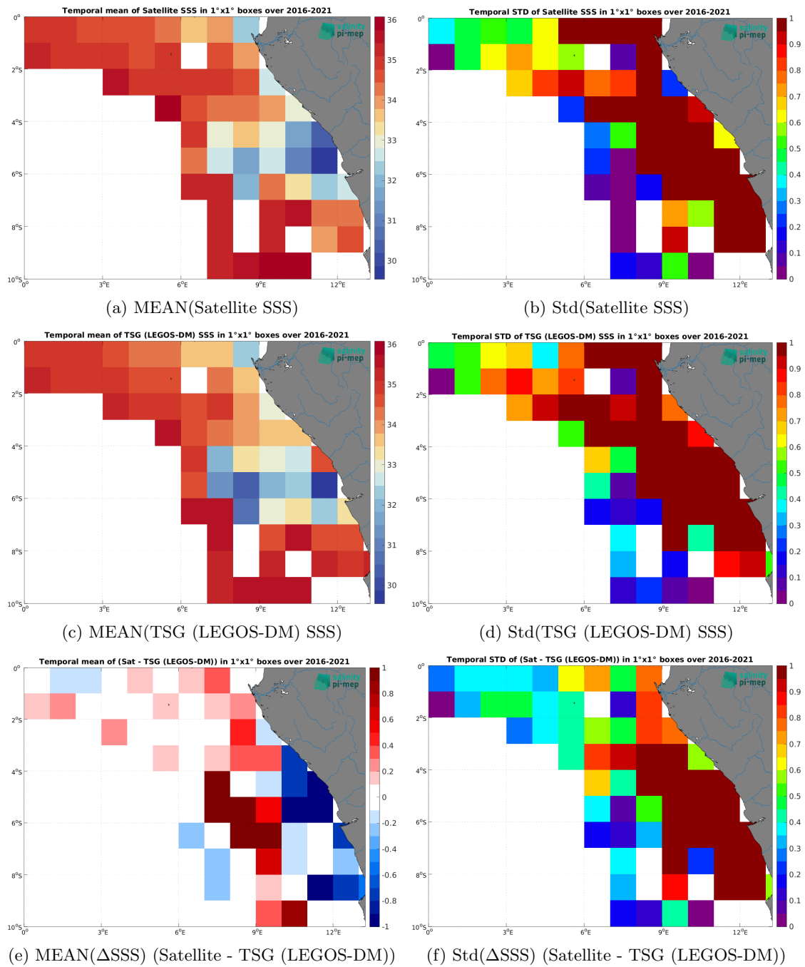
Figure 7: Temporal mean (left) and Std (right) of SSS from SMAP SSS L3 v6 - Monthly (RSS) (top), TSG (LEGOS-DM) (middle), and of \Delta SSS (Satellite - TSG (LEGOS-DM)). Only match-pairs are used to generate these maps.
