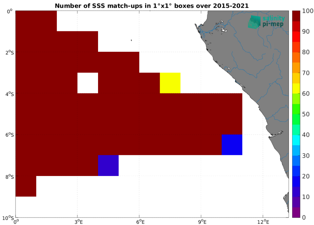
Figure 5: Number of SSS match-ups between TSG (GOSUD-Research-vessel) SSS and the SMAP SSS L3 v6 - Monthly (RSS) SSS product for the Congo river plume Pi-MEP region over 1^\circ \times 1^\circ boxes and for the full satellite product period.
