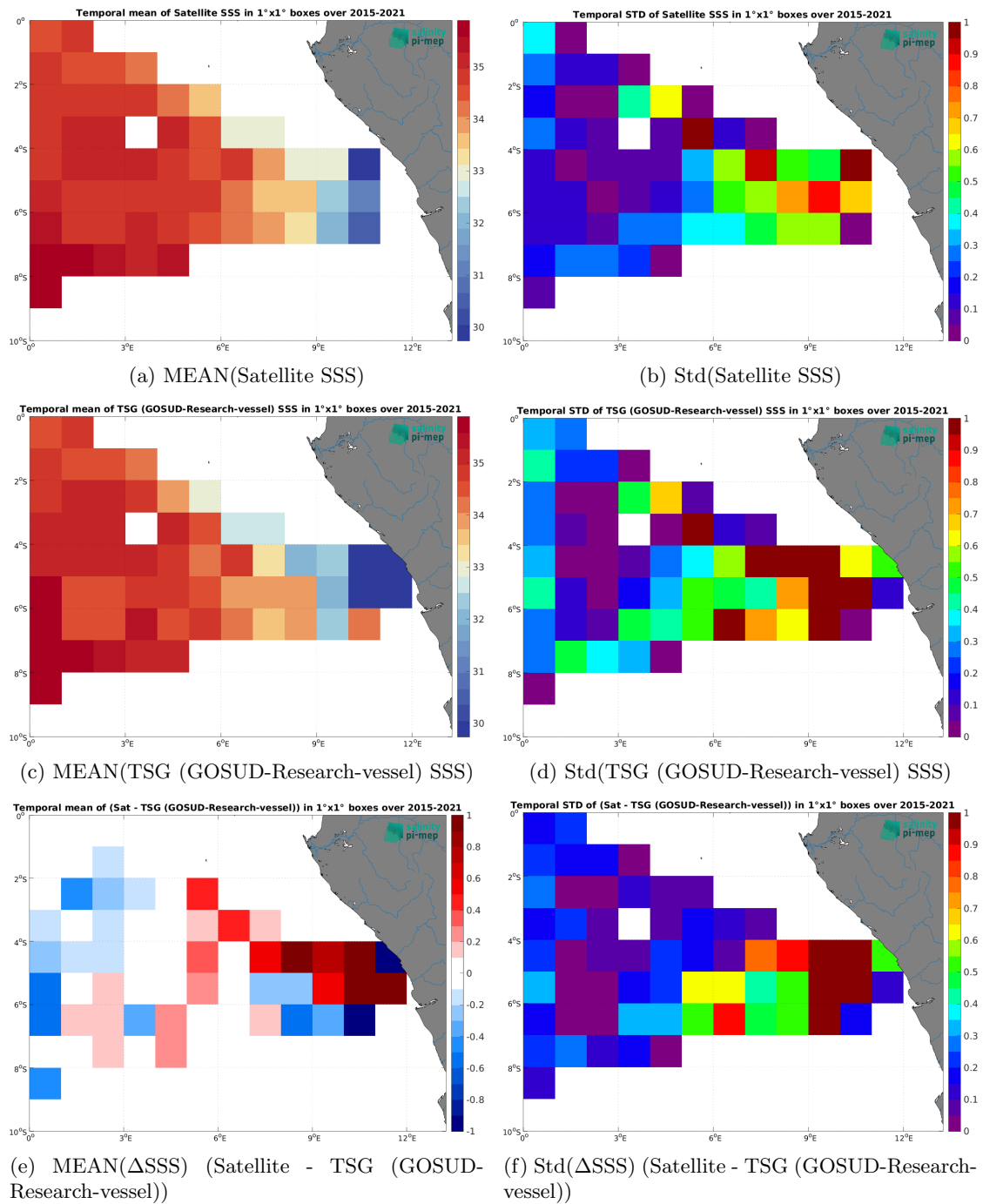
Figure 7: Temporal mean (left) and Std (right) of SSS from SMAP SSS L3 v6 - Monthly (RSS) (top), TSG (GOSUD-Research-vessel) (middle), and of \Delta SSS (Satellite - TSG (GOSUD-Research-vessel)). Only match-up pairs are used to generate these maps.
