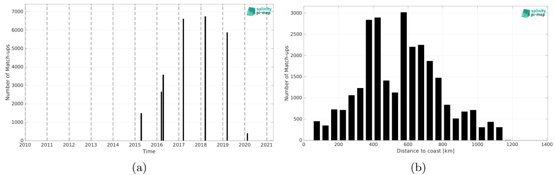
Figure 2: Number of match-ups between TSG (GOSUD-Research-vessel) and SMAP SSS L3 v6 - Monthly (RSS) SSS as a function of time (a) and as function of the distance to coast (b) over the Congo river plume Pi-MEP region and for the full satellite product period.
