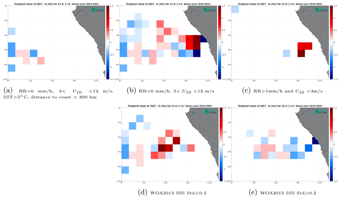
Figure 14: Temporal mean gridded over spatial boxes of size 1^\circ \times 1^\circ of \Delta\text{SSS} (SMAP SSS L3 v6 - Monthly (RSS) - TSG (GOSUD-Research-vessel)) for 5 different subdatasets corresponding to:RR=0 mm/h, 3 < U_{10} < 12 m/s, SST > 5^\circ\text{C} , distance to coast > 800 km (a), RR=0 mm/h, 3 < U_{10} < 12 m/s (b), RR > 1 mm/h and U_{10} < 4 m/s (c), WOA2013 SSS Std < 0.2 (d), WOA2013 SSS Std > 0.2 (e).
