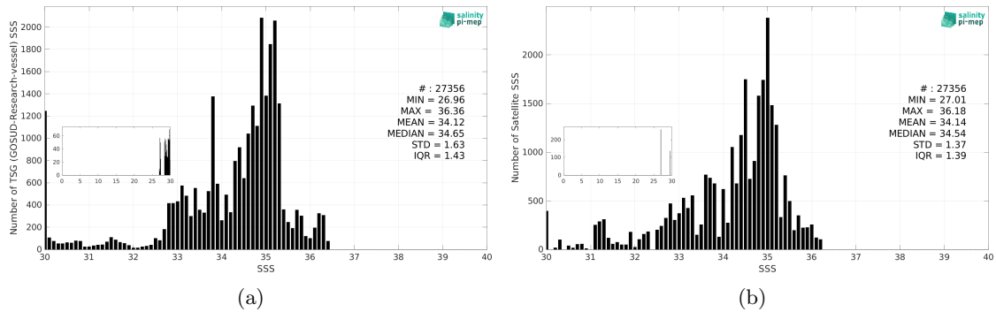
Figure 3: Histograms of SSS from TSG (GOSUD-Research-vessel) (a) and SMAP SSS L3 v6 - Monthly (RSS) (b) considering all match-up pairs per bins of 0.1 over the Congo river plume Pi-MEP region and for the full satellite product period.
