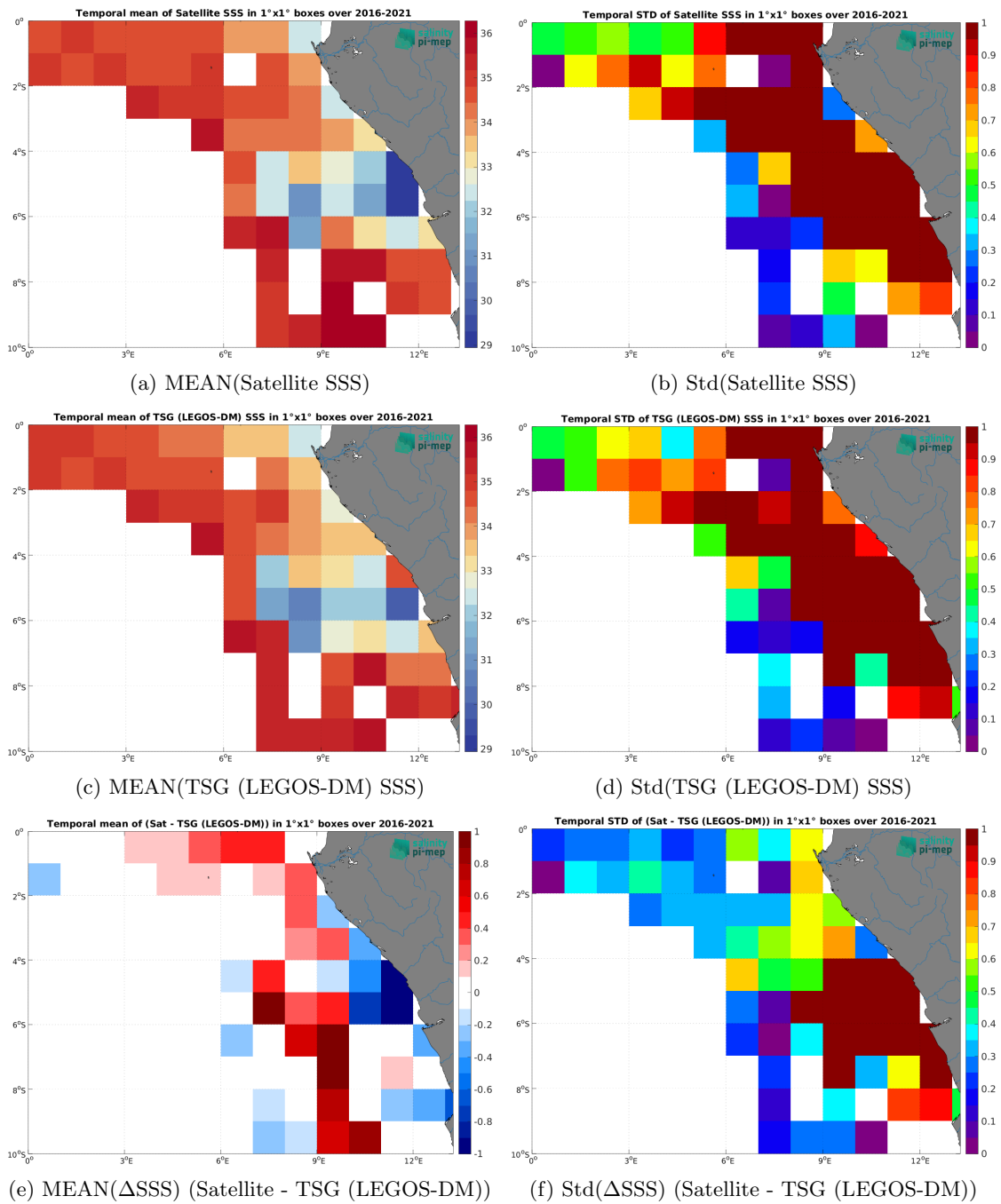
Figure 7: Temporal mean (left) and Std (right) of SSS from SMAP SSS L3 v5.3 - 8-Day running (RSS) (top), TSG (LEGOS-DM) (middle), and of \Delta SSS (Satellite - TSG (LEGOS-DM)). Only match-up pairs are used to generate these maps.
