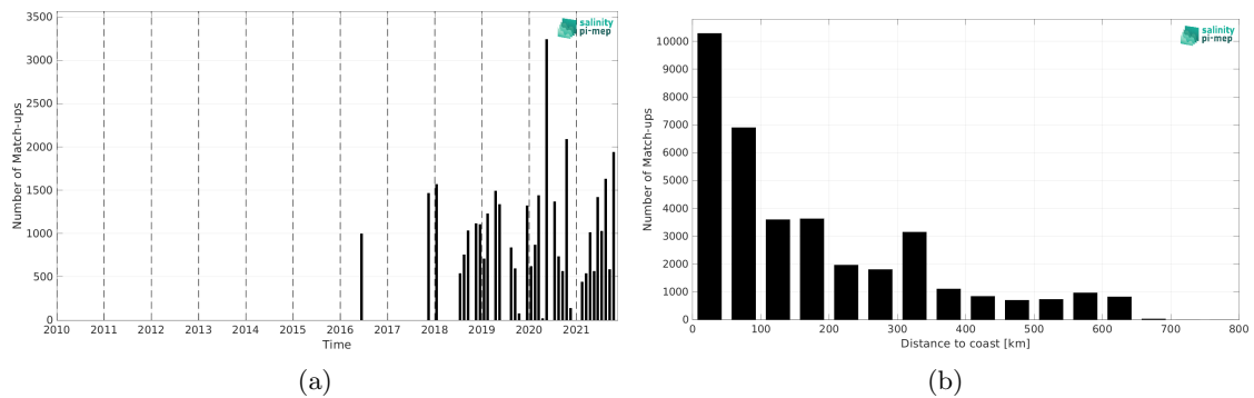
Figure 2: Number of match-ups between TSG (LEGOS-DM) and SMAP SSS L3 v5.3 - 8-Day running (RSS) SSS as a function of time (a) and as function of the distance to coast (b) over the Congo river plume Pi-MEP region and for the full satellite product period.
