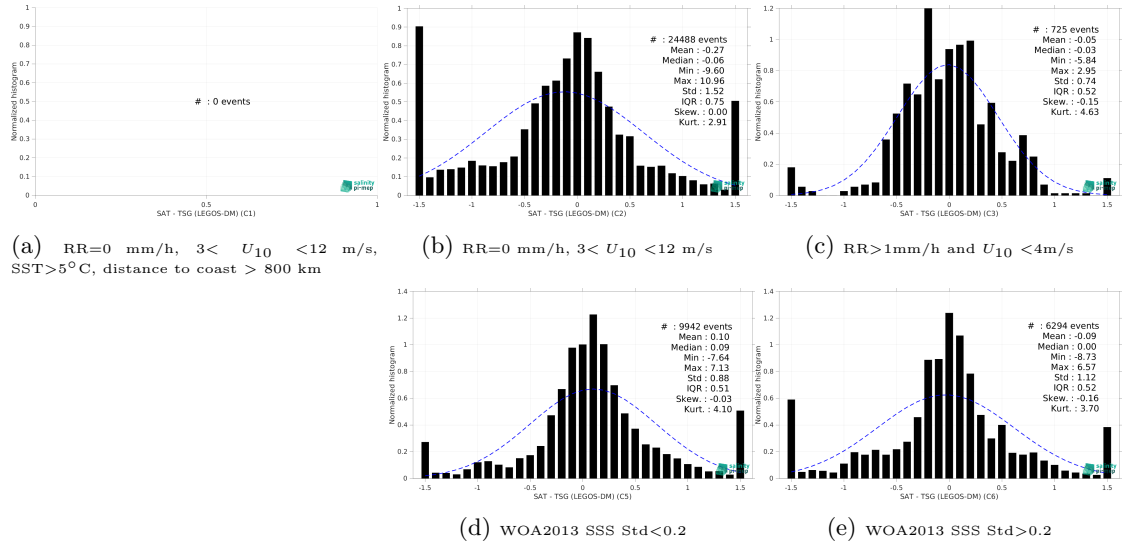
Figure 15: Normalized histogram of \Delta SSS (SMAP SSS L3 v5.3 - 8-Day running (RSS) - TSG (LEGOS-DM)) for 5 different subdatasets corresponding to: RR=0 mm/h, 3 < U_{10} < 12 m/s, SST > 5°C, distance to coast > 800 km (a), RR=0 mm/h, 3 < U_{10} < 12 m/s (b), RR > 1mm/h and U_{10} < 4 m/s (c), WOA2013 SSS Std < 0.2 (d), WOA2013 SSS Std > 0.2 (e).
