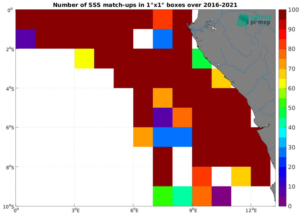
Figure 5: Number of SSS match-ups between TSG (LEGOS-DM) SSS and the SMAP SSS L3 v5.3 - 8-Day running (RSS) SSS product for the Congo river plume Pi-MEP region over 1^\circ \times 1^\circ boxes and for the full satellite product period.
