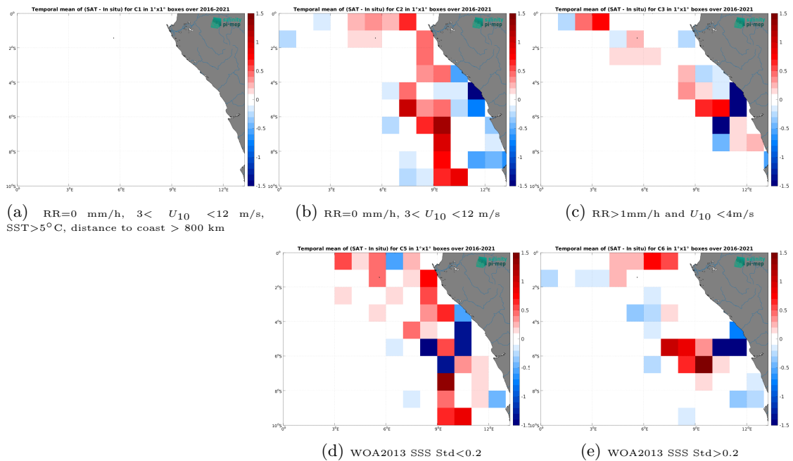
Figure 14: Temporal mean gridded over spatial boxes of size 1^\circ \times 1^\circ of \Delta SSS (SMAP SSS L3 v5.3 - 8-Day running (RSS) - TSG (LEGOS-DM)) for 5 different subdatasets corresponding to: RR=0 mm/h, 3 < U_{10} < 12 m/s, SST > 5°C, distance to coast > 800 km (a), RR=0 mm/h, 3 < U_{10} < 12 m/s (b), RR > 1mm/h and U_{10} < 4 m/s (c), WOA2013 SSS Std < 0.2 (d), WOA2013 SSS Std > 0.2 (e).
