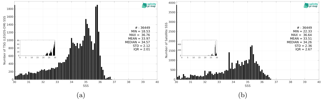
Figure 3: Histograms of SSS from TSG (LEGOS-DM) (a) and SMAP SSS L3 v5.3 - 8-Day running (RSS) (b) considering all match-up pairs per bins of 0.1 over the Congo river plume Pi-MEP region and for the full satellite product period.
