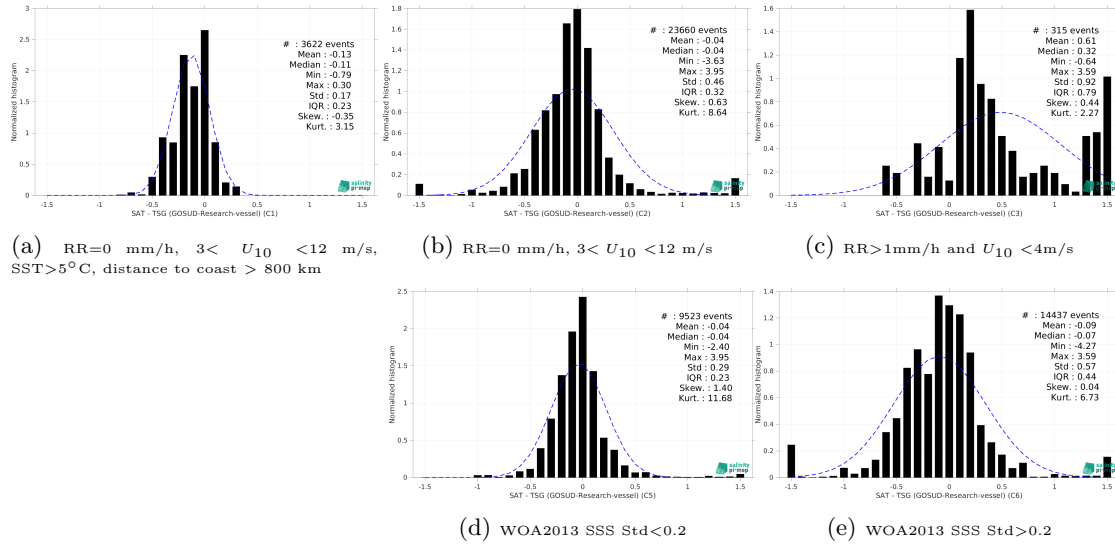
Figure 15: Normalized histogram of \Delta SSS (SMAP SSS L3 v5.3 - 8-Day running (RSS) - TSG (GOSUD-Research-vessel)) for 5 different subdatasets corresponding to: RR=0 mm/h, 3 < U_{10} < 12 m/s, SST > 5°C, distance to coast > 800 km (a), RR=0 mm/h, 3 < U_{10} < 12 m/s (b), RR > 1mm/h and U_{10} < 4 m/s (c), WOA2013 SSS Std < 0.2 (d), WOA2013 SSS Std > 0.2 (e).
