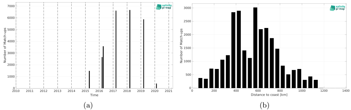
Figure 2: Number of match-ups between TSG (GOSUD-Research-vessel) and SMAP SSS L3 v5.3 - 8-Day running (RSS) SSS as a function of time (a) and as function of the distance to coast (b) over the Congo river plume Pi-MEP region and for the full satellite product period.
