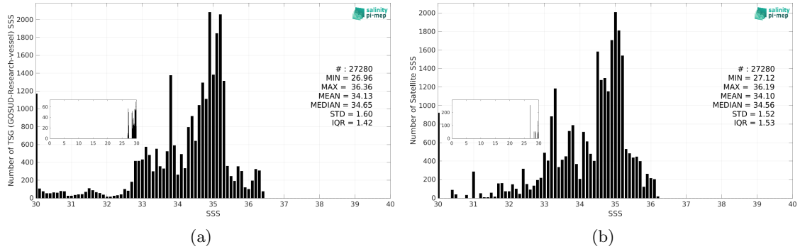
Figure 3: Histograms of SSS from TSG (GOSUD-Research-vessel) (a) and SMAP SSS L3 v5.3 - 8-Day running (RSS) (b) considering all match-up pairs per bins of 0.1 over the Congo river plume Pi-MEP region and for the full satellite product period.
