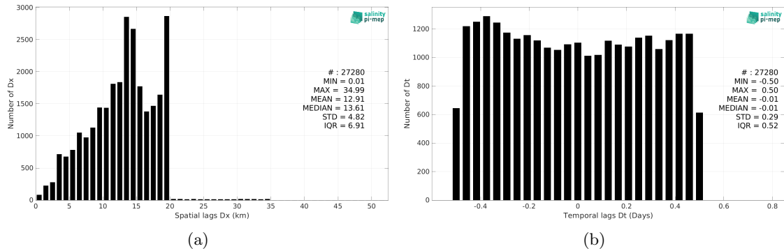
Figure 6: Histograms of the spatial (a) and temporal (b) lags between the location/time of the TSG (GOSUD-Research-vessel) measurement and the date of the corresponding SMAP SSS L3 v5.3 - 8-Day running (RSS) SSS pixel.
