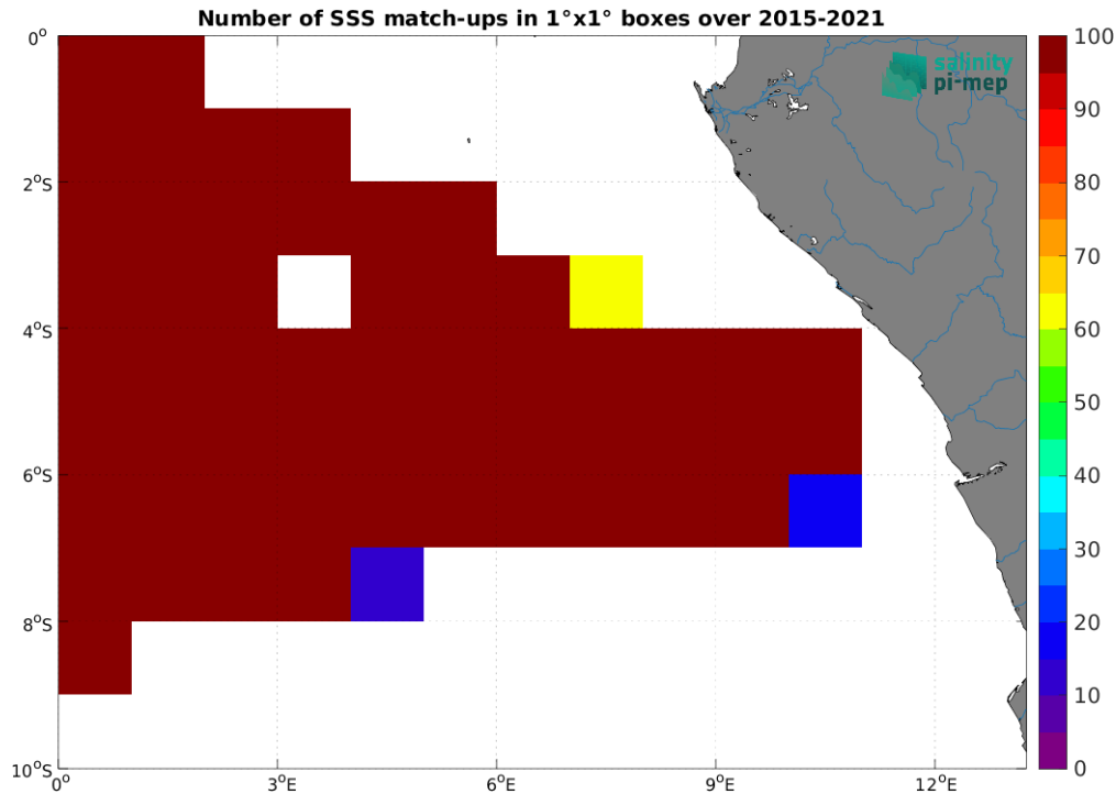
Figure 5: Number of SSS match-ups between TSG (GOSUD-Research-vessel) SSS and the SMAP SSS L3 v5.3 - 8-Day running (RSS) SSS product for the Congo river plume Pi-MEP region over 1^\circ \times 1^\circ boxes and for the full satellite product period.
