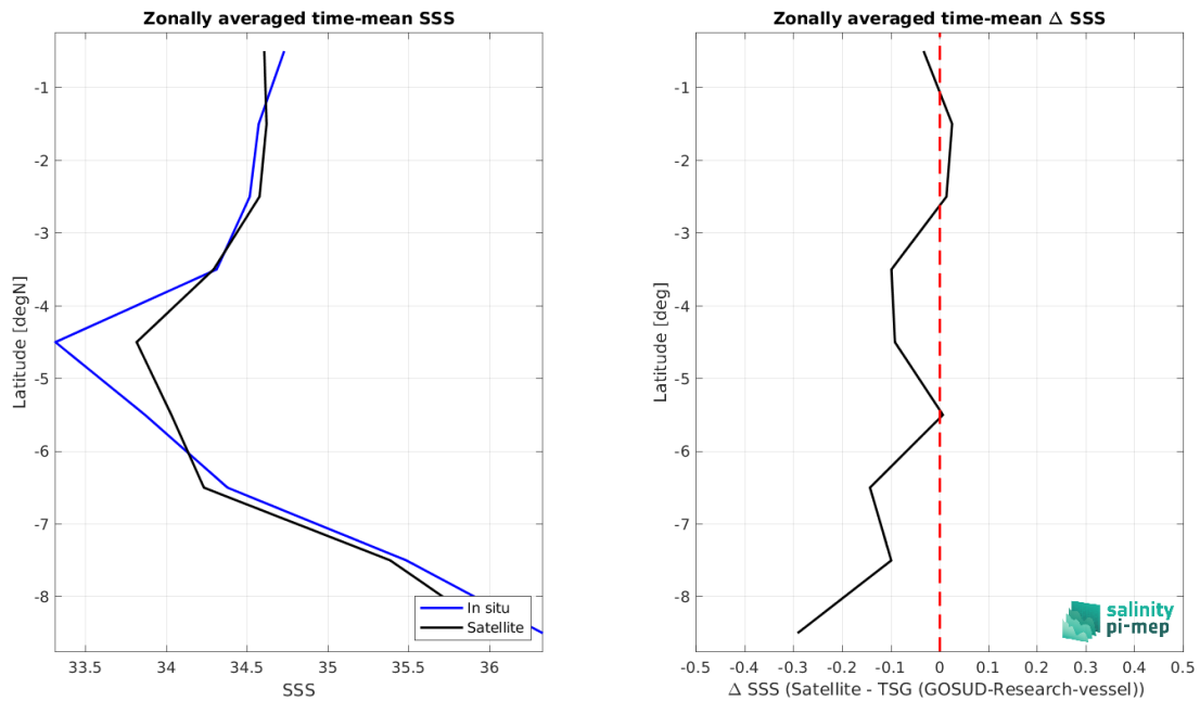
Figure 9: Left panel: Zonal mean SSS from SMAP SSS L3 v5.3 - 8-Day running (RSS) satellite product (black) and from TSG (GOSUD-Research-vessel) (blue). Right panel: Zonal mean of \Delta SSS (Satellite - TSG (GOSUD-Research-vessel)) for all the collected Pi-MEP match-up pairs estimated over the full satellite product period.
