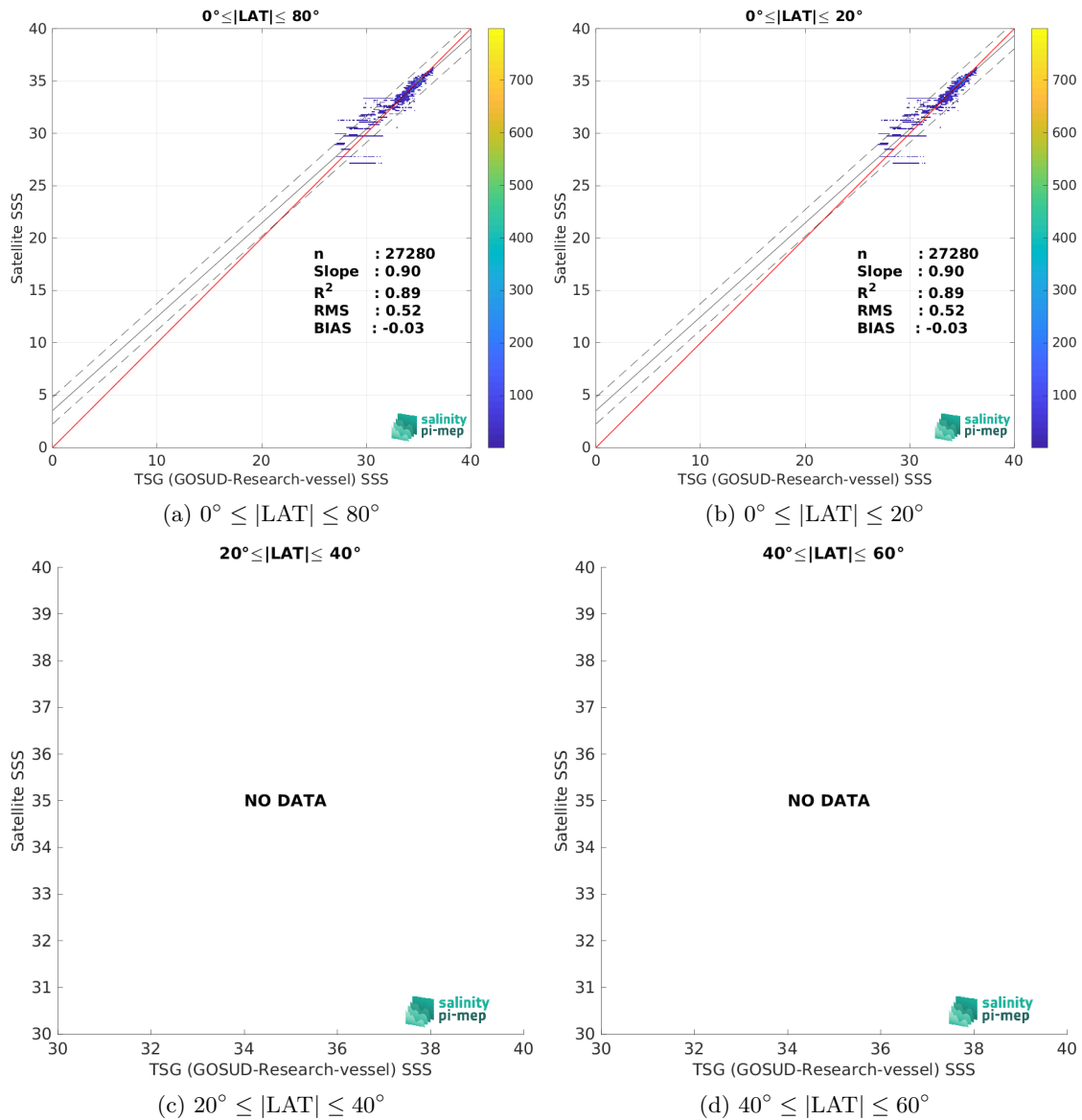
Figure 10: Contour maps of the concentration of SMAP SSS L3 v5.3 - 8-Day running (RSS) SSS (y-axis) versus TSG (GOSUD-Research-vessel) SSS (x-axis) at match-up pairs for different latitude bands. For each plot, the red line shows x=y . The black thin and dashed lines indicate a linear fit through the data cloud and the \pm 95\% confidence levels, respectively. The number match-up pairs n , the slope and R^2 coefficient of the linear fit, the root mean square (RMS) and the mean bias between satellite and in situ data are indicated for each latitude band in each plots.
