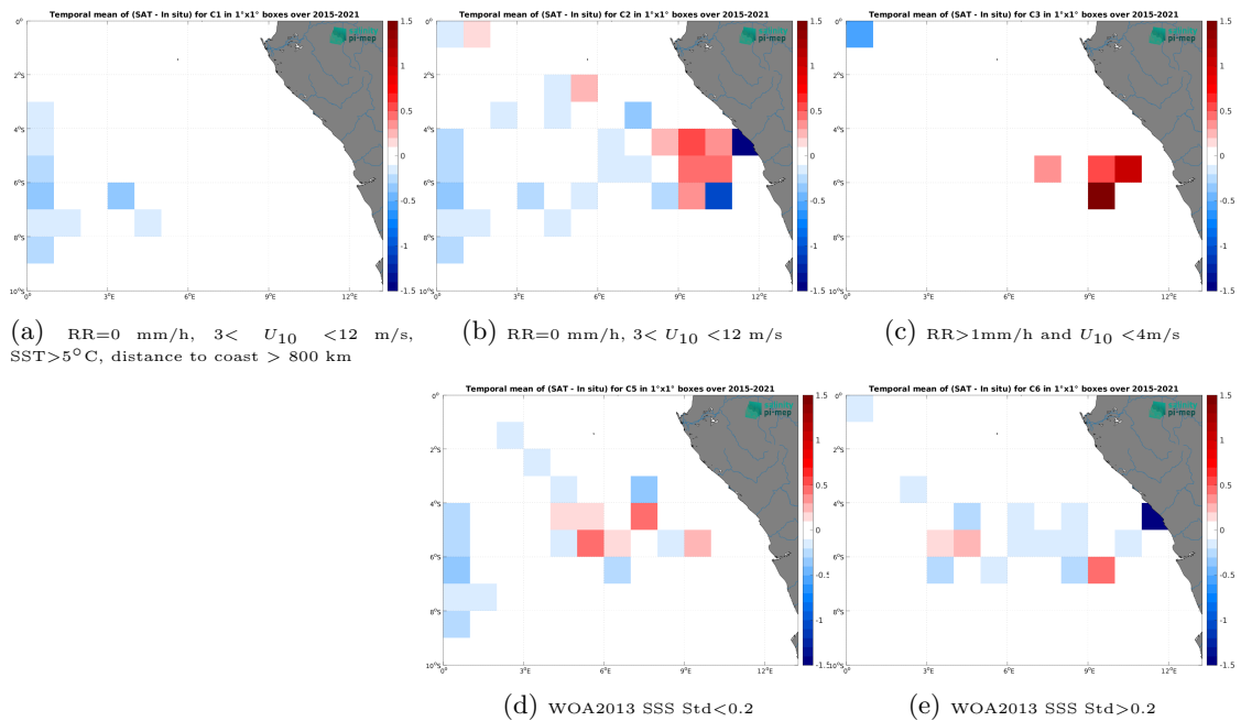
Figure 14: Temporal mean gridded over spatial boxes of size 1^\circ \times 1^\circ of \Delta SSS (SMAP SSS L3 v5.3 - 8-Day running (RSS) - TSG (GOSUD-Research-vessel)) for 5 different subdatasets corresponding to:RR=0 mm/h, 3 < U_{10} < 12 m/s, SST>5°C, distance to coast > 800 km (a), RR=0 mm/h, 3 < U_{10} < 12 m/s (b), RR>1mm/h and U_{10} < 4 m/s (c), WOA2013 SSS Std<0.2 (d), WOA2013 SSS Std>0.2 (e).
