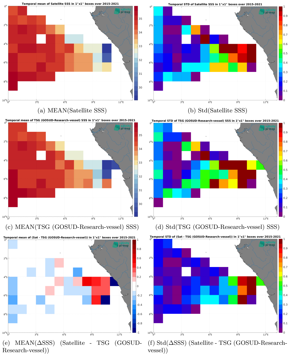
Figure 7: Temporal mean (left) and Std (right) of SSS from SMAP SSS L3 v5.3 - 8-Day running (RSS) (top), TSG (GOSUD-Research-vessel) (middle), and of \Delta SSS (Satellite - TSG (GOSUD-Research-vessel)). Only match-up pairs are used to generate these maps.
