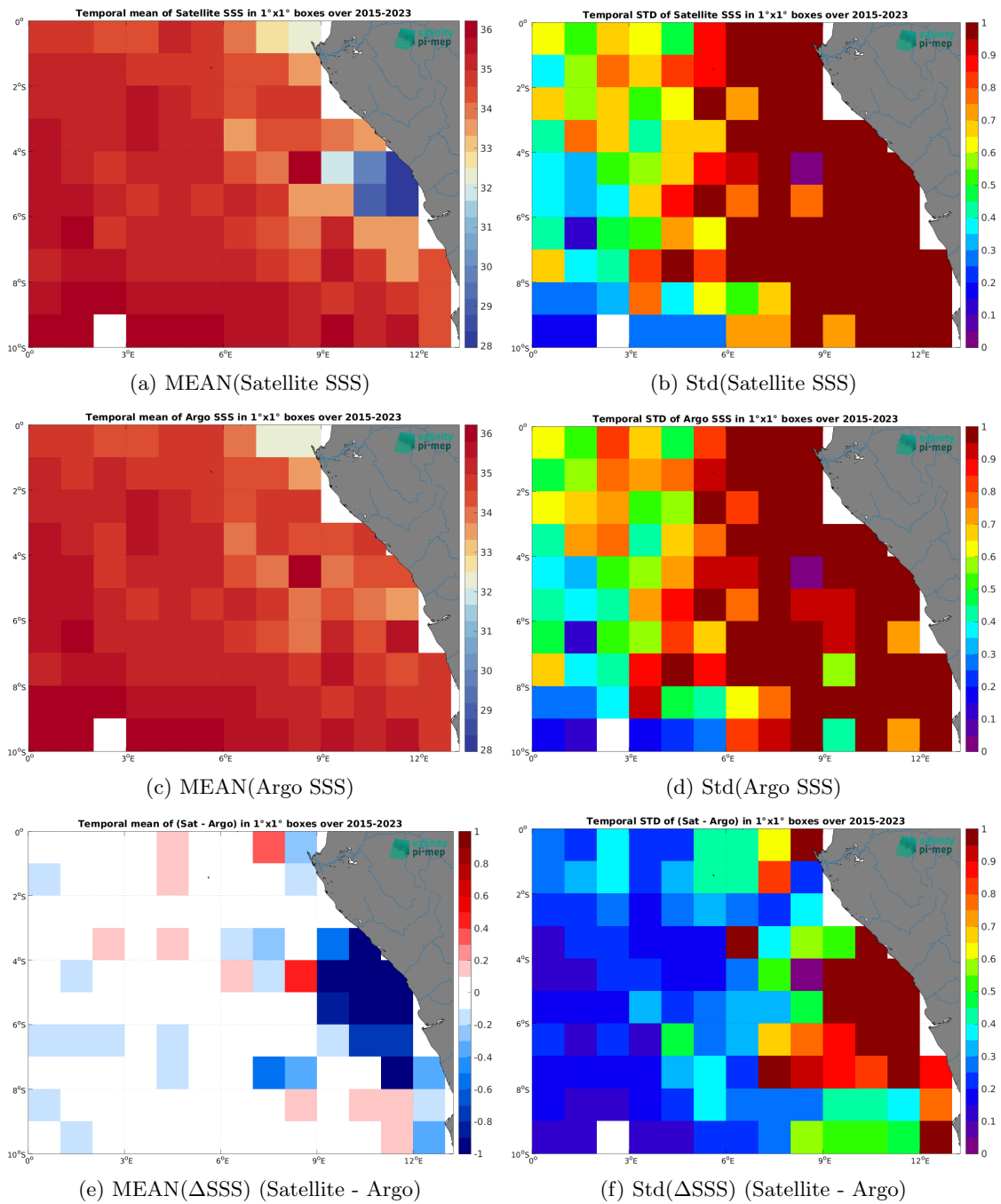
Figure 7: Temporal mean (left) and Std (right) of SSS from SMAP SSS L3 v5.3 - 8-Day running (RSS) (top), Argo (middle), and of \Delta SSS (Satellite - Argo). Only match-up pairs are used to generate these maps.
