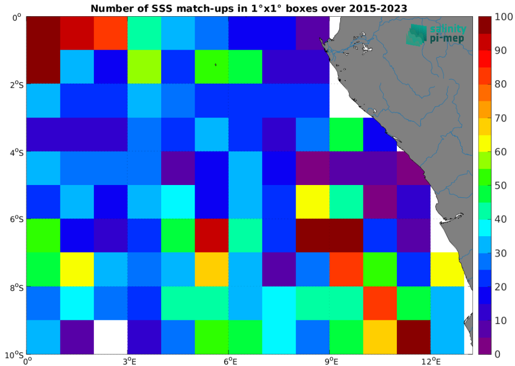
Figure 5: Number of SSS match-ups between Argo SSS and the SMAP SSS L3 v5.3 - 8-Day running (RSS) SSS product for the Congo river plume Pi-MEP region over 1^\circ \times 1^\circ boxes and for the full satellite product period.
