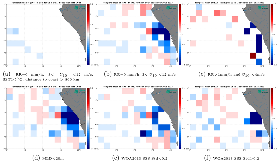
Figure 14: Temporal mean gridded over spatial boxes of size 1^\circ \times 1^\circ of \Delta SSS (SMAP SSS L3 v5.3 - 8-Day running (RSS) - Argo) for 6 different subdatasets corresponding to:RR=0 mm/h, 3 < U_{10} < 12 m/s, SST >5^\circ C, distance to coast > 800 km (a), RR=0 mm/h, 3 < U_{10} < 12 m/s (b), RR >1 mm/h and U_{10} < 4 m/s (c),MLD <20 m (d),WOA2013 SSS Std <0.2 (e),WOA2013 SSS Std >0.2 (f).
