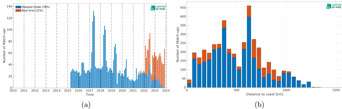
Figure 2: Number of match-ups between Argo and SMAP SSS L3 v5.3 - 8-Day running (RSS) SSS as a function of time (a) and as function of the distance to coast (b) over the Congo river plume Pi-MEP region and for the full satellite product period.
