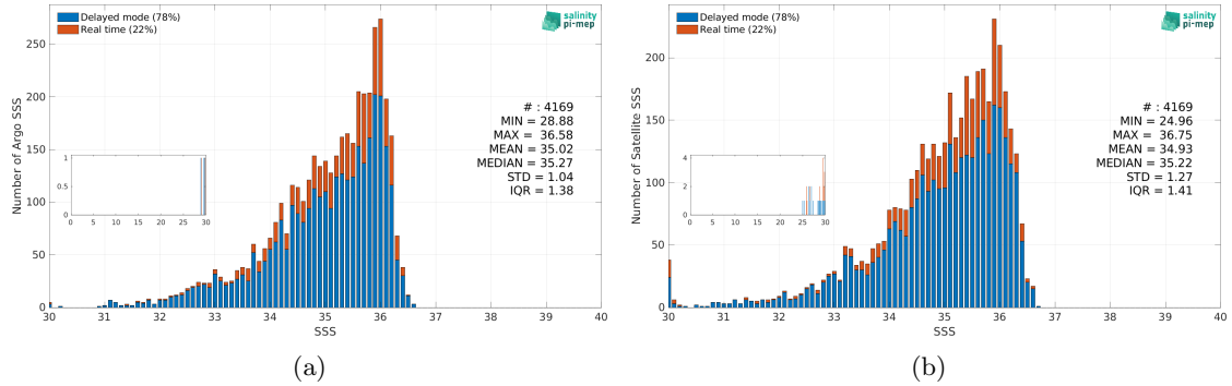
Figure 3: Histograms of SSS from Argo (a) and SMAP SSS L3 v5.3 - 8-Day running (RSS) (b) considering all match-up pairs per bins of 0.1 over the Congo river plume Pi-MEP region and for the full satellite product period.
