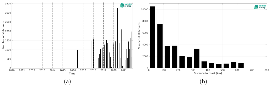
Figure 2: Number of match-ups between TSG (LEGOS-DM) and SMAP SSS L3 v5.3 - Monthly (RSS) SSS as a function of time (a) and as function of the distance to coast (b) over the Congo river plume Pi-MEP region and for the full satellite product period.
