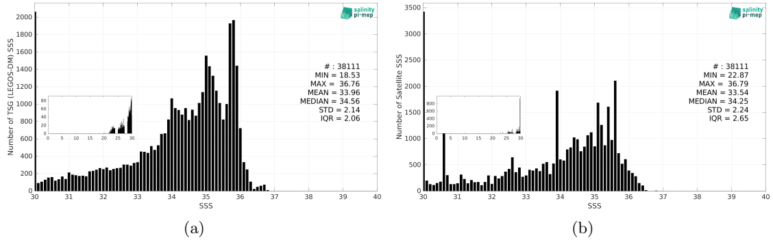
Figure 3: Histograms of SSS from TSG (LEGOS-DM) (a) and SMAP SSS L3 v5.3 - Monthly (RSS) (b) considering all match-up pairs per bins of 0.1 over the Congo river plume Pi-MEP region and for the full satellite product period.
