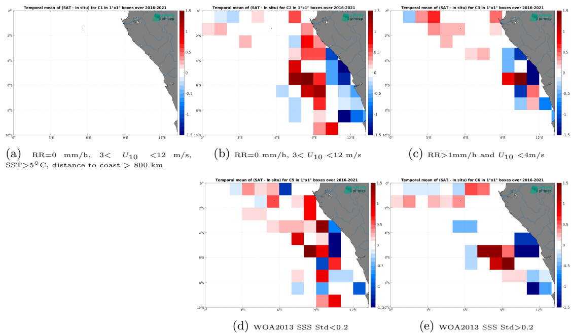
Figure 14: Temporal mean gridded over spatial boxes of size 1^\circ \times 1^\circ of \Delta SSS (SMAP SSS L3 v5.3 - Monthly (RSS) - TSG (LEGOS-DM)) for 5 different subdatasets corresponding to:RR=0 mm/h, 3 < U_{10} < 12 m/s, SST > 5^\circ\text{C} , distance to coast > 800 km (a), RR=0 mm/h, 3 < U_{10} < 12 m/s (b), RR > 1 mm/h and U_{10} < 4 m/s (c), WOA2013 SSS Std < 0.2 (d), WOA2013 SSS Std > 0.2 (e).
