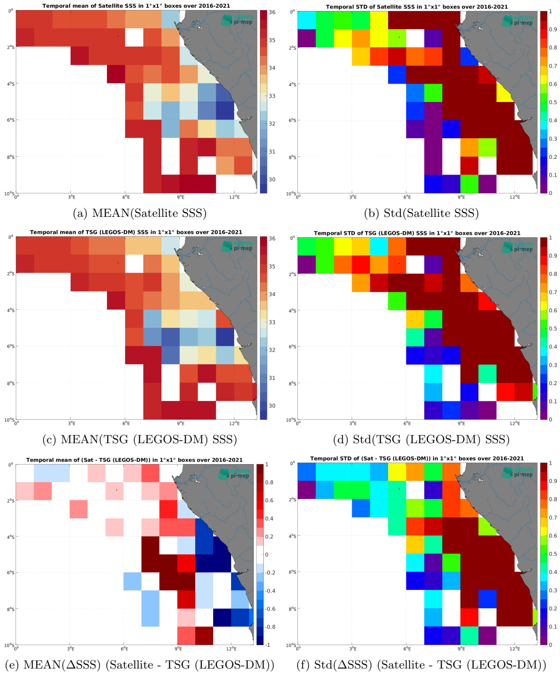
Figure 7: Temporal mean (left) and Std (right) of SSS from SMAP SSS L3 v5.3 - Monthly (RSS) (top), TSG (LEGOS-DM) (middle), and of \Delta SSS (Satellite - TSG (LEGOS-DM)). Only match-up pairs are used to generate these maps.
