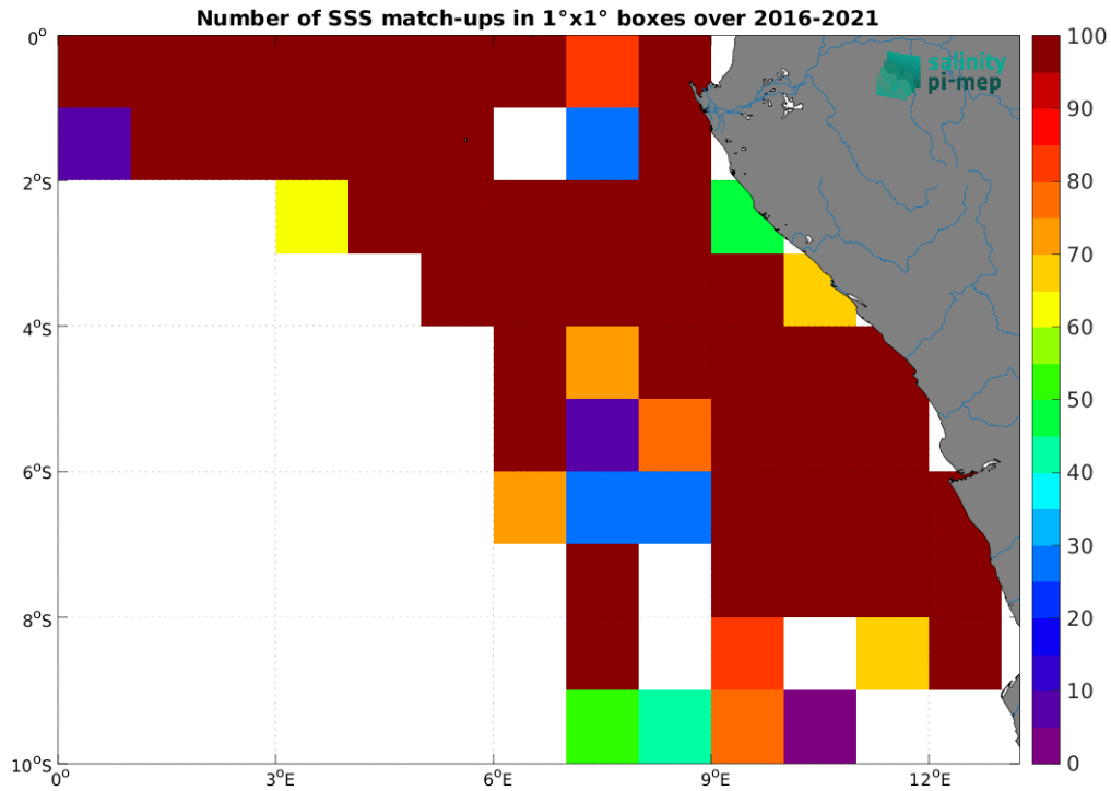
Figure 5: Number of SSS match-ups between TSG (LEGOS-DM) SSS and the SMAP SSS L3 v5.3 - Monthly (RSS) SSS product for the Congo river plume Pi-MEP region over 1^\circ \times 1^\circ boxes and for the full satellite product period.
