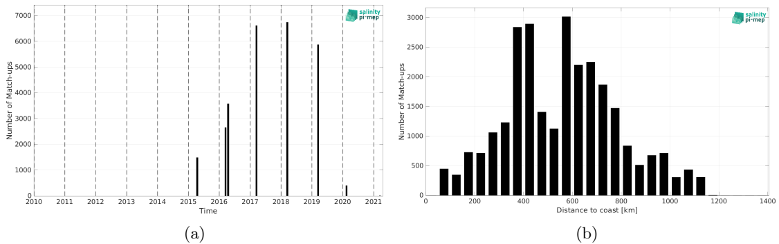
Figure 2: Number of match-ups between TSG (GOSUD-Research-vessel) and SMAP SSS L3 v5.3 - Monthly (RSS) SSS as a function of time (a) and as function of the distance to coast (b) over the Congo river plume Pi-MEP region and for the full satellite product period.
