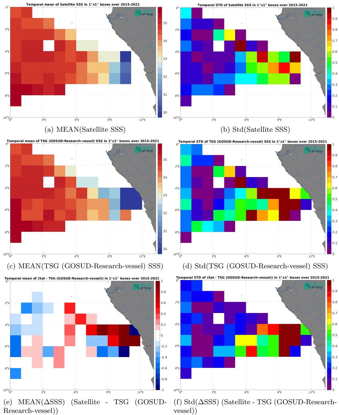
Figure 7: Temporal mean (left) and Std (right) of SSS from SMAP SSS L3 v5.3 - Monthly (RSS) (top), TSG (GOSUD-Research-vessel) (middle), and of \Delta SSS (Satellite - TSG (GOSUD-Research-vessel)). Only match-up pairs are used to generate these maps.
