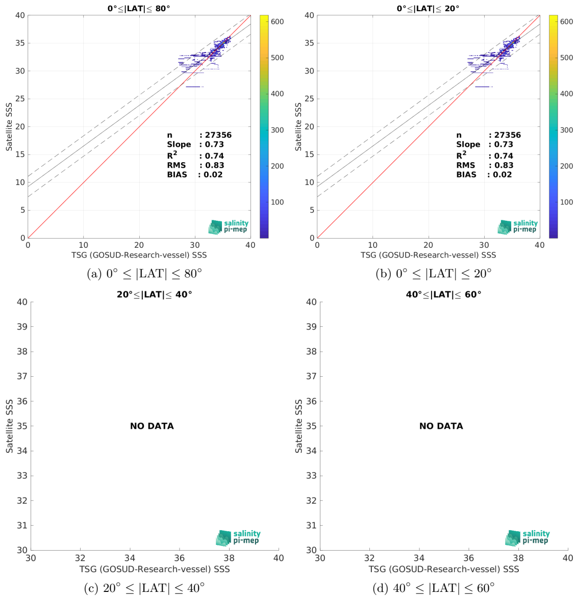
Figure 10: Contour maps of the concentration of SMAP SSS L3 v5.3 - Monthly (RSS) SSS (y-axis) versus TSG (GOSUD-Research-vessel) SSS (x-axis) at match-up pairs for different latitude bands. For each plot, the red line shows x=y . The black thin and dashed lines indicate a linear fit through the data cloud and the \pm 95\% confidence levels, respectively. The number match-up pairs n , the slope and R^2 coefficient of the linear fit, the root mean square (RMS) and the mean bias between satellite and in situ data are indicated for each latitude band in each plots.
