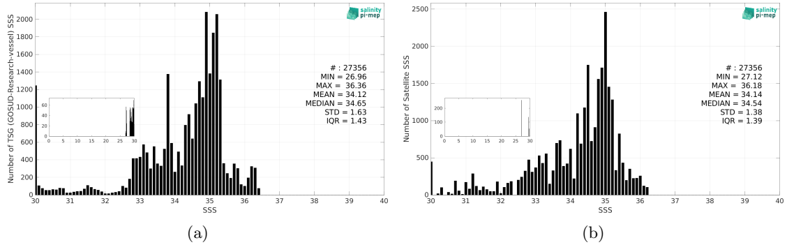
Figure 3: Histograms of SSS from TSG (GOSUD-Research-vessel) (a) and SMAP SSS L3 v5.3 - Monthly (RSS) (b) considering all match-up pairs per bins of 0.1 over the Congo river plume Pi-MEP region and for the full satellite product period.
