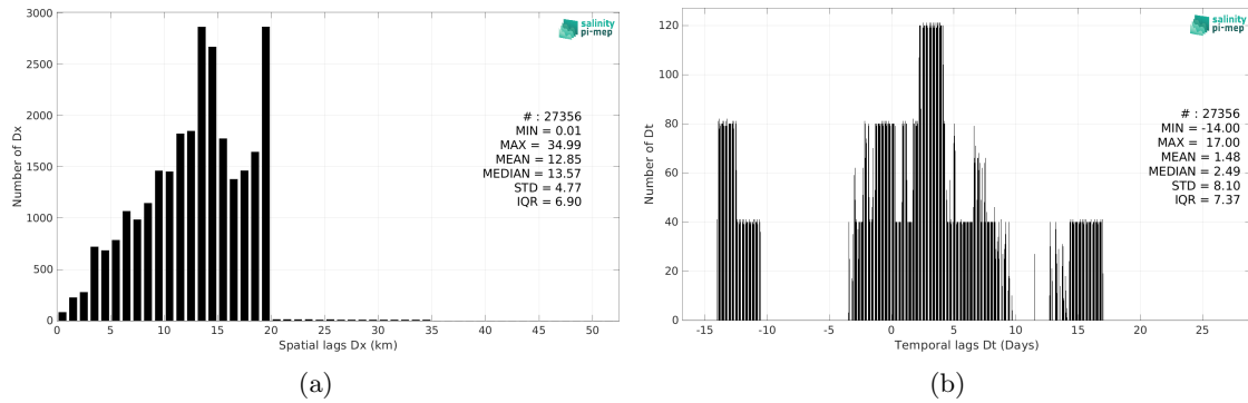
Figure 6: Histograms of the spatial (a) and temporal (b) lags between the location/time of the TSG (GOSUD-Research-vessel) measurement and the date of the corresponding SMAP SSS L3 v5.3 - Monthly (RSS) SSS pixel.
