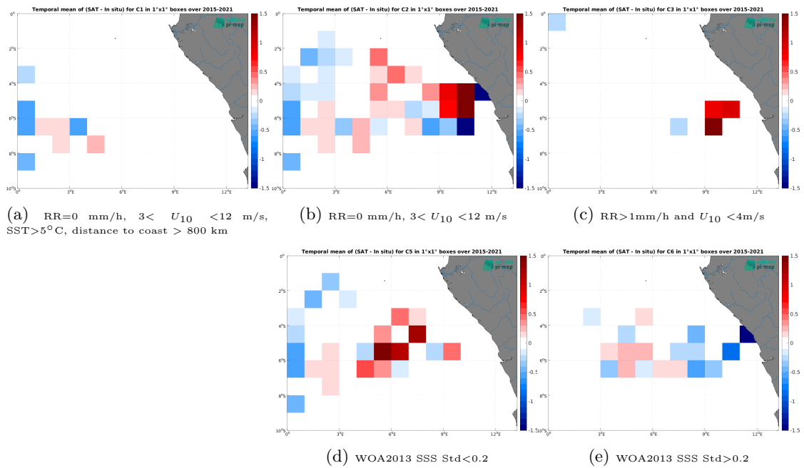
Figure 14: Temporal mean gridded over spatial boxes of size 1^\circ \times 1^\circ of \Delta SSS (SMAP SSS L3 v5.3 - Monthly (RSS) - TSG (GOSUD-Research-vessel)) for 5 different subdatasets corresponding to:RR=0 mm/h, 3 < U_{10} < 12 m/s, SST > 5°C, distance to coast > 800 km (a), RR=0 mm/h, 3 < U_{10} < 12 m/s (b), RR > 1mm/h and U_{10} < 4 m/s (c), WOA2013 SSS Std < 0.2 (d), WOA2013 SSS Std > 0.2 (e).
