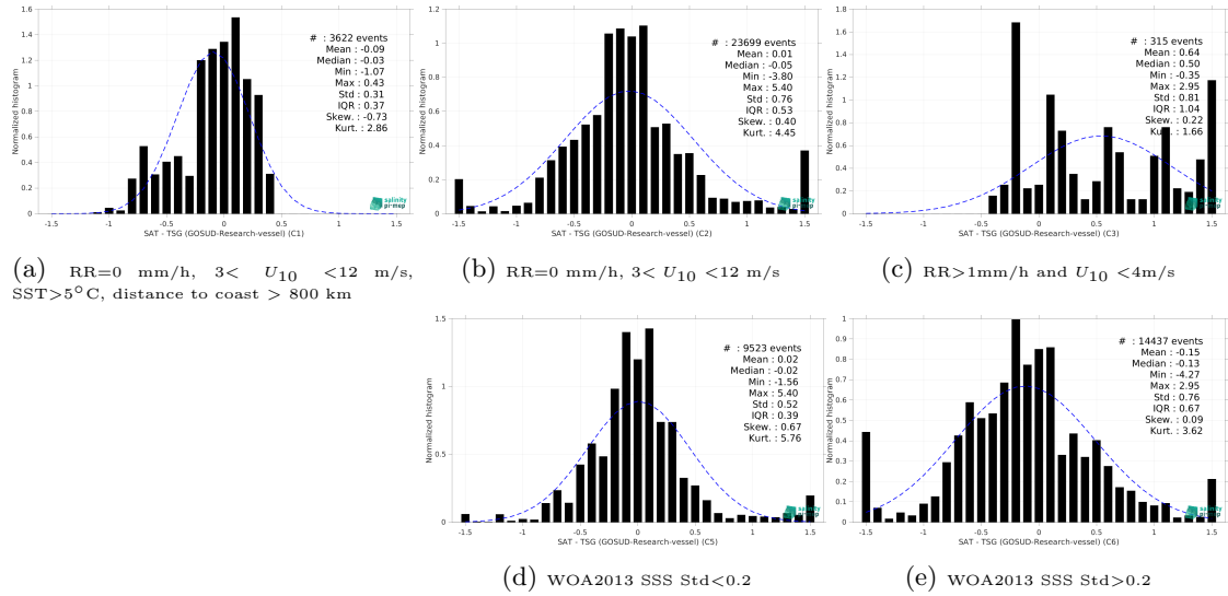
Figure 15: Normalized histogram of \Delta SSS (SMAP SSS L3 v5.3 - Monthly (RSS) - TSG (GOSUD-Research-vessel)) for 5 different subdatasets corresponding to: RR=0 mm/h, 3 < U_{10} < 12 m/s, SST>5°C, distance to coast > 800 km (a), RR=0 mm/h, 3 < U_{10} < 12 m/s (b), RR>1mm/h and U_{10} < 4 m/s (c), WOA2013 SSS Std<0.2 (d), WOA2013 SSS Std>0.2 (e).
