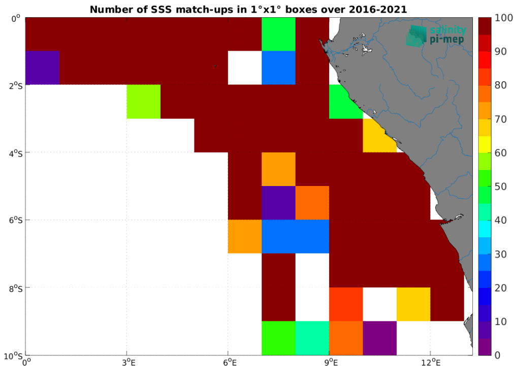
Figure 4: Number of SSS match-ups between TSG (LEGOS-DM) SSS and the SMAP SSS L3 v5 - 8-Day running (RSS) SSS product for the Congo river plume Pi-MEP region over 1^\circ \times 1^\circ boxes and for the full satellite product period.
