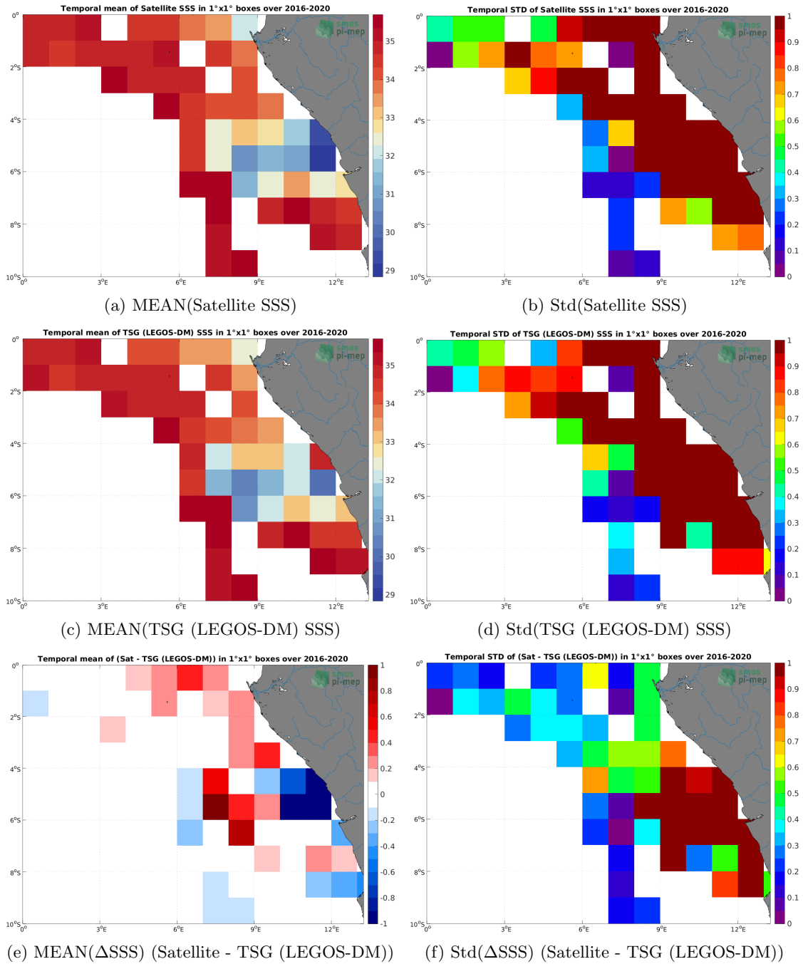
Figure 6: Temporal mean (left) and Std (right) of SSS from SMAP SSS L3 v5 - 8-Day running (RSS) (top), TSG (LEGOS-DM) (middle), and of \Delta SSS (Satellite - TSG (LEGOS-DM)). Only match-up pairs are used to generate these maps.
