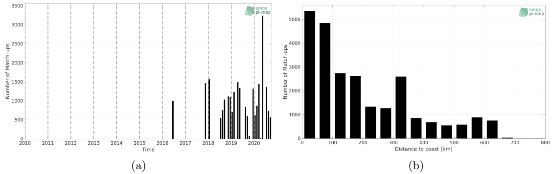
Figure 1: Number of match-ups between TSG (LEGOS-DM) and SMAP SSS L3 v5 - 8-Day running (RSS) SSS as a function of time (a) and as function of the distance to coast (b) over the Congo river plume Pi-MEP region and for the full satellite product period.
