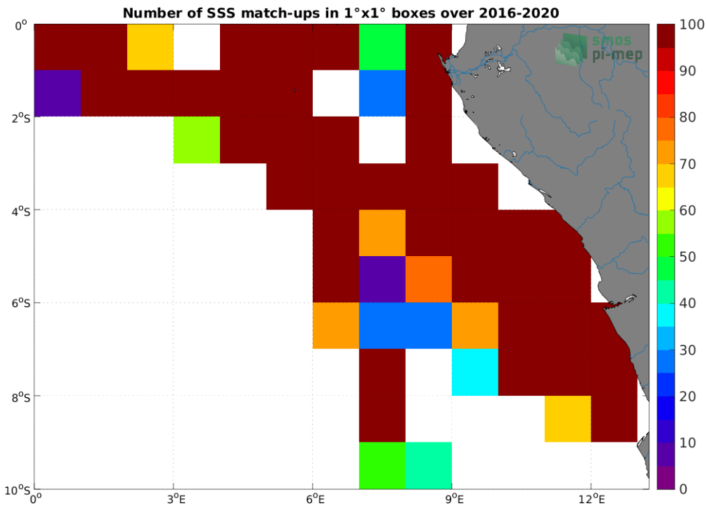
Figure 4: Number of SSS match-ups between TSG (LEGOS-DM) SSS and the SMAP SSS L3 v5 - 8-Day running (RSS) SSS product for the Congo river plume Pi-MEP region over 1^{\circ} \times 1^{\circ} boxes and for the full satellite product period.
