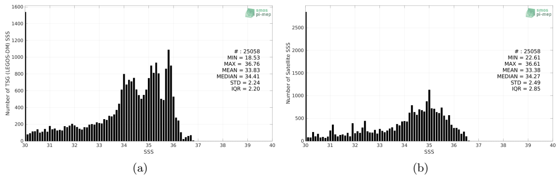
Figure 2: Histograms of SSS from TSG (LEGOS-DM) (a) and SMAP SSS L3 v5 - 8-Day running (RSS) (b) considering all match-up pairs per bins of 0.1 over the Congo river plume Pi-MEP region and for the full satellite product period.
