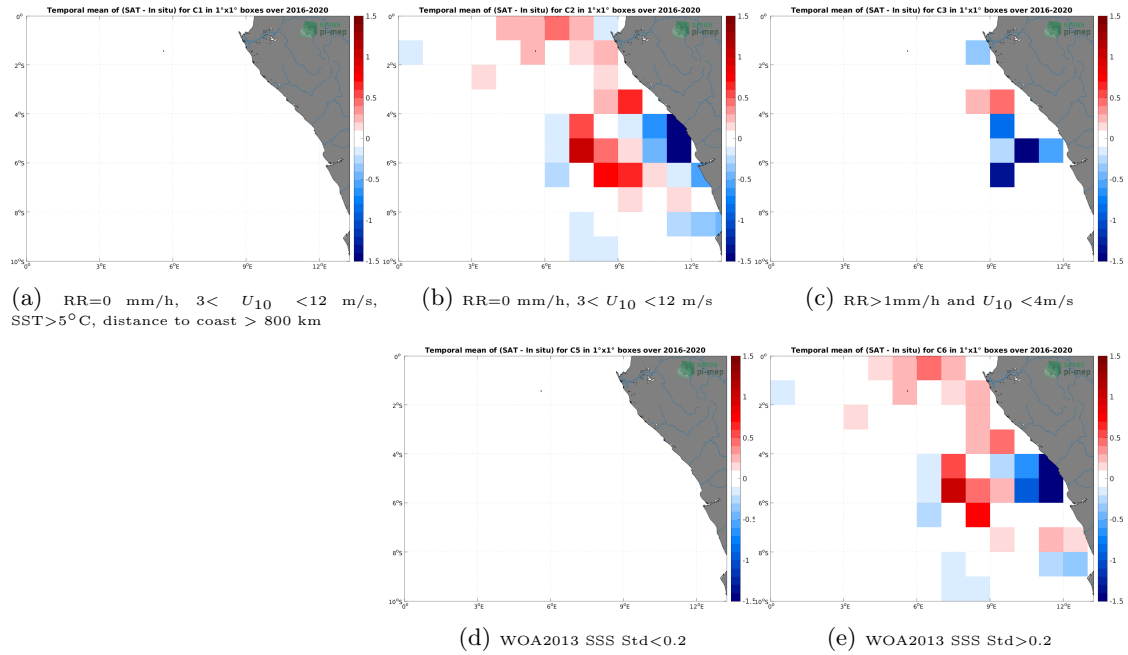
Figure 12: Temporal mean gridded over spatial boxes of size 1^\circ \times 1^\circ of \Delta SSS (SMAP SSS L3 v5 - 8-Day running (RSS) - TSG (LEGOS-DM)) for 5 different subdatasets corresponding to:RR=0 mm/h, 3 < U_{10} < 12 m/s, SST > 5^\circ C , distance to coast > 800 km (a), RR=0 mm/h, 3 < U_{10} < 12 m/s (b), RR >1 mm/h and U_{10} < 4 m/s (c), WOA2013 SSS Std <0.2 (d), WOA2013 SSS Std >0.2 (e).
