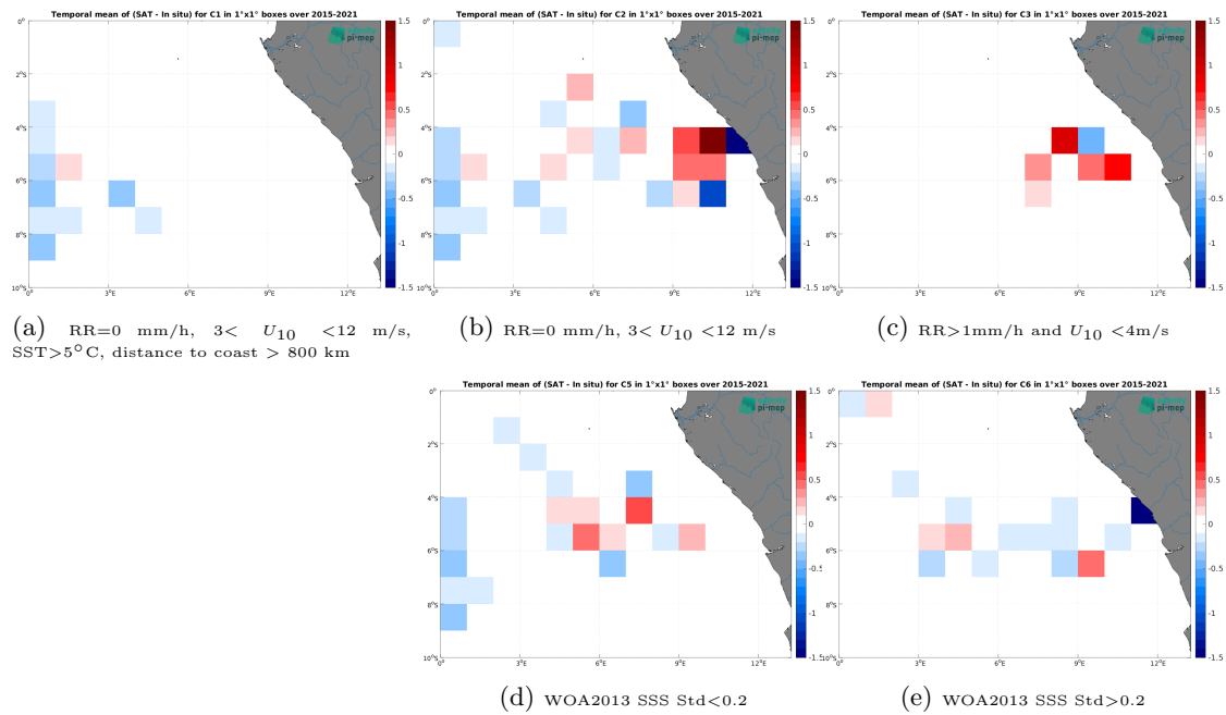
Figure 12: Temporal mean gridded over spatial boxes of size 1^\circ \times 1^\circ of \Delta SSS (SMAP SSS L3 v5 - 8-Day running (RSS) - TSG (GOSUD-Research-vessel)) for 5 different subdatasets corresponding to:RR=0 mm/h, 3 < U_{10} < 12 m/s, SST >5^\circ C, distance to coast > 800 km (a), RR=0 mm/h, 3 < U_{10} < 12 m/s (b), RR >1 mm/h and U_{10} < 4 m/s (c), WOA2013 SSS Std <0.2 (d), WOA2013 SSS Std >0.2 (e).
