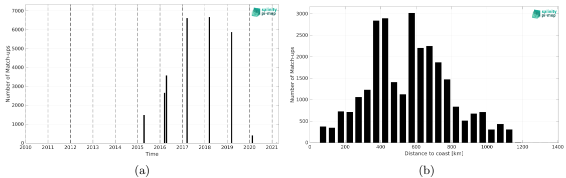
Figure 1: Number of match-ups between TSG (GOSUD-Research-vessel) and SMAP SSS L3 v5 - 8-Day running (RSS) SSS as a function of time (a) and as function of the distance to coast (b) over the Congo river plume Pi-MEP region and for the full satellite product period.
