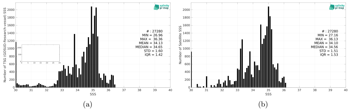
Figure 2: Histograms of SSS from TSG (GOSUD-Research-vessel) (a) and SMAP SSS L3 v5 - 8-Day running (RSS) (b) considering all match-up pairs per bins of 0.1 over the Congo river plume Pi-MEP region and for the full satellite product period.
