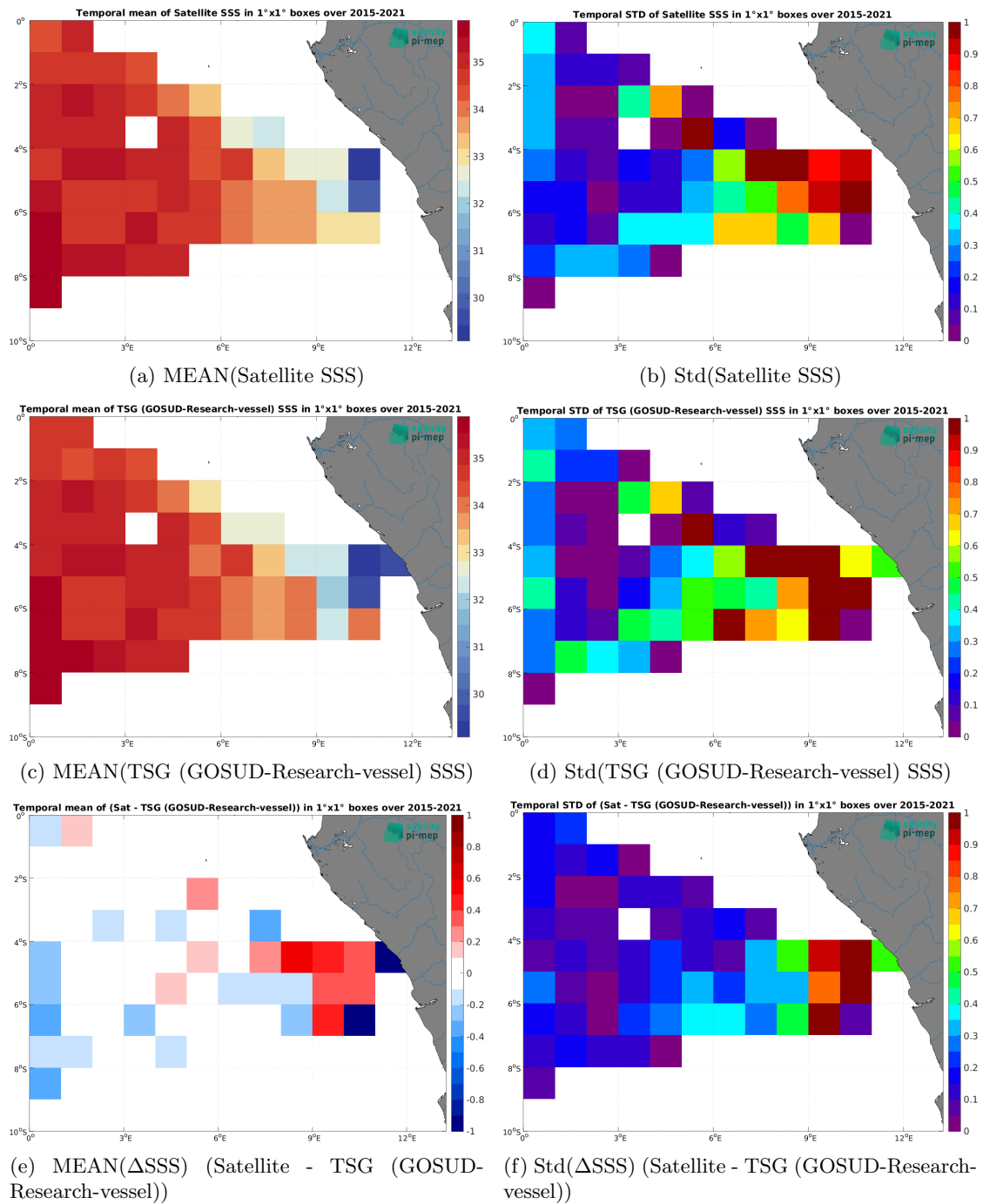
Figure 6: Temporal mean (left) and Std (right) of SSS from SMAP SSS L3 v5 - 8-Day running (RSS) (top), TSG (GOSUD-Research-vessel) (middle), and of \Delta SSS (Satellite - TSG (GOSUD-Research-vessel)). Only match-up pairs are used to generate these maps.
