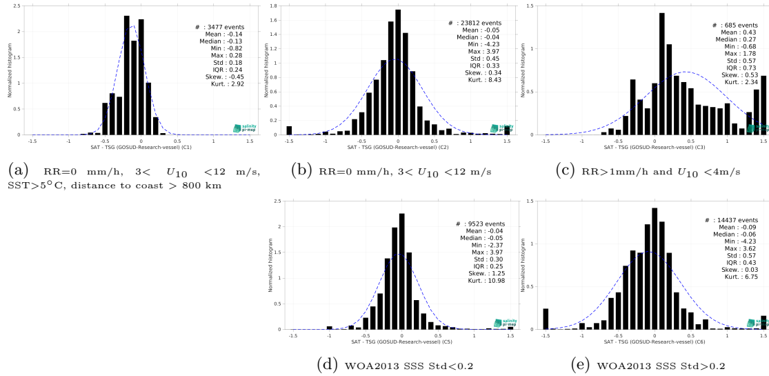
Figure 13: Normalized histogram of \Delta SSS (SMAP SSS L3 v5 - 8-Day running (RSS) - TSG (GOSUD-Research-vessel)) for 5 different subdatasets corresponding to: RR=0 mm/h, 3 < U_{10} < 12 m/s, SST > 5°C, distance to coast > 800 km (a), RR=0 mm/h, 3 < U_{10} < 12 m/s (b), RR > 1mm/h and U_{10} < 4 m/s (c), WOA2013 SSS Std < 0.2 (d), WOA2013 SSS Std > 0.2 (e).
