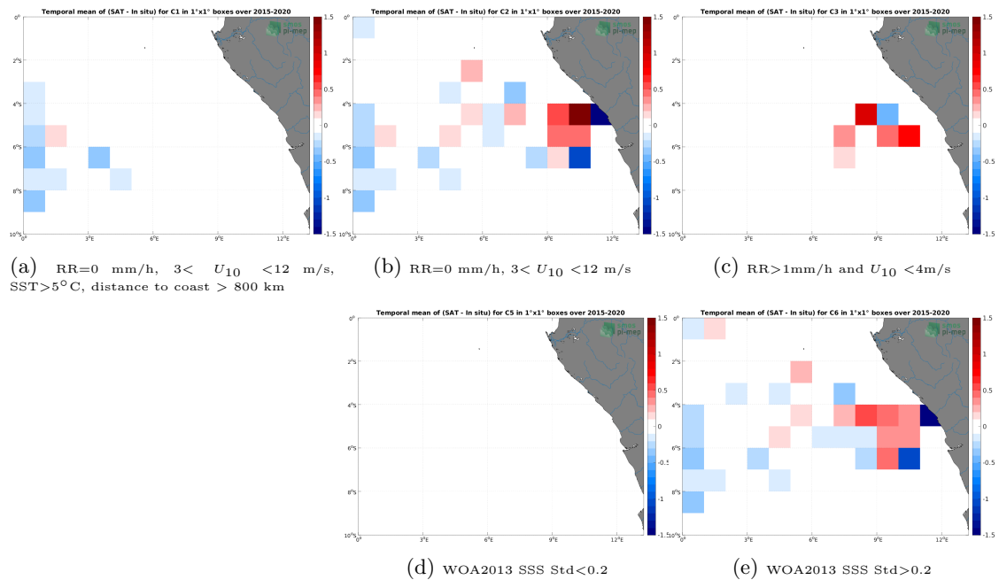
Figure 12: Temporal mean gridded over spatial boxes of size 1^\circ \times 1^\circ of \Delta\text{SSS} (SMAP SSS L3 v5 - 8-Day running (RSS) - TSG (GOSUD-Research-vessel)) for 5 different subdatasets corresponding to:RR=0 mm/h, 3 < U_{10} < 12 m/s, SST > 5^\circ\text{C} , distance to coast > 800 km (a), RR=0 mm/h, 3 < U_{10} < 12 m/s (b), RR > 1 mm/h and U_{10} < 4 m/s (c), WOA2013 SSS Std < 0.2 (d), WOA2013 SSS Std > 0.2 (e).
