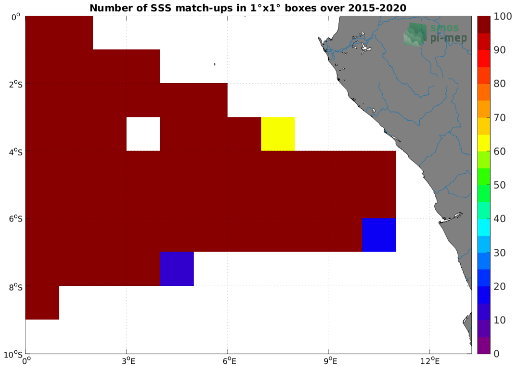
Figure 4: Number of SSS match-ups between TSG (GOSUD-Research-vessel) SSS and the SMAP SSS L3 v5 - 8-Day running (RSS) SSS product for the Congo river plume Pi-MEP region over 1^{\circ} \times 1^{\circ} boxes and for the full satellite product period.
