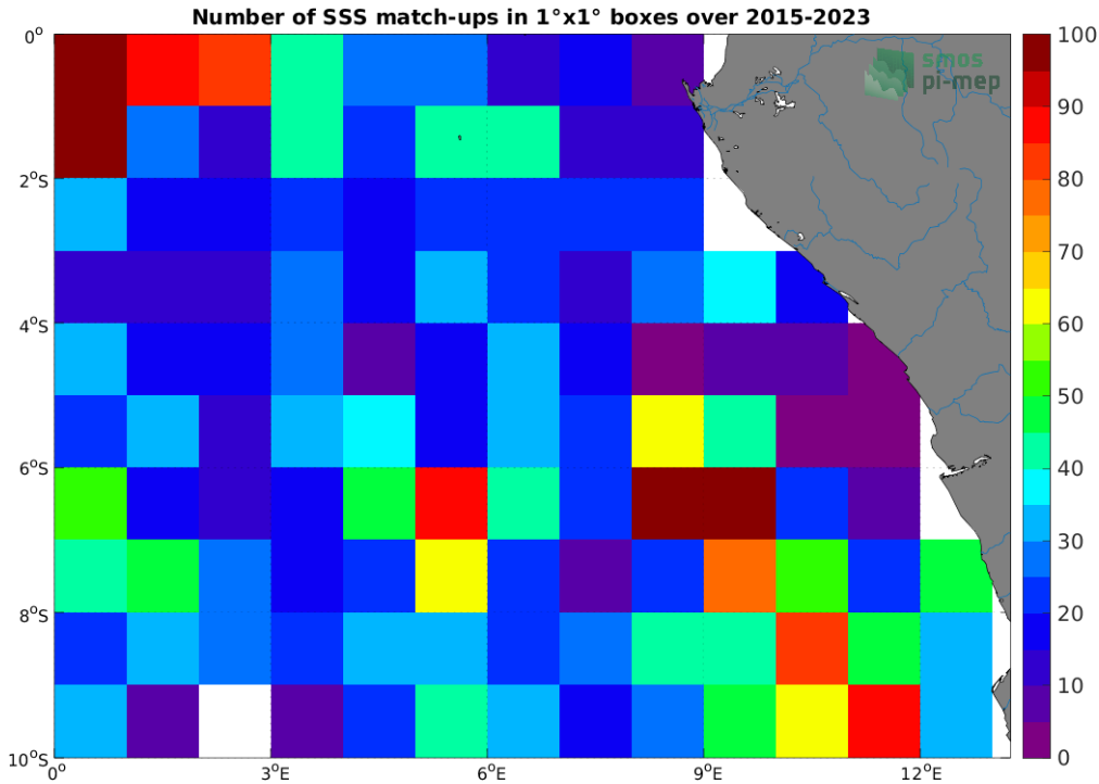
Figure 4: Number of SSS match-ups between Argo SSS and the SMAP SSS L3 v5 - 8-Day running (RSS) SSS product for the Congo river plume Pi-MEP region over 1°x1° boxes and for the full satellite product period.
