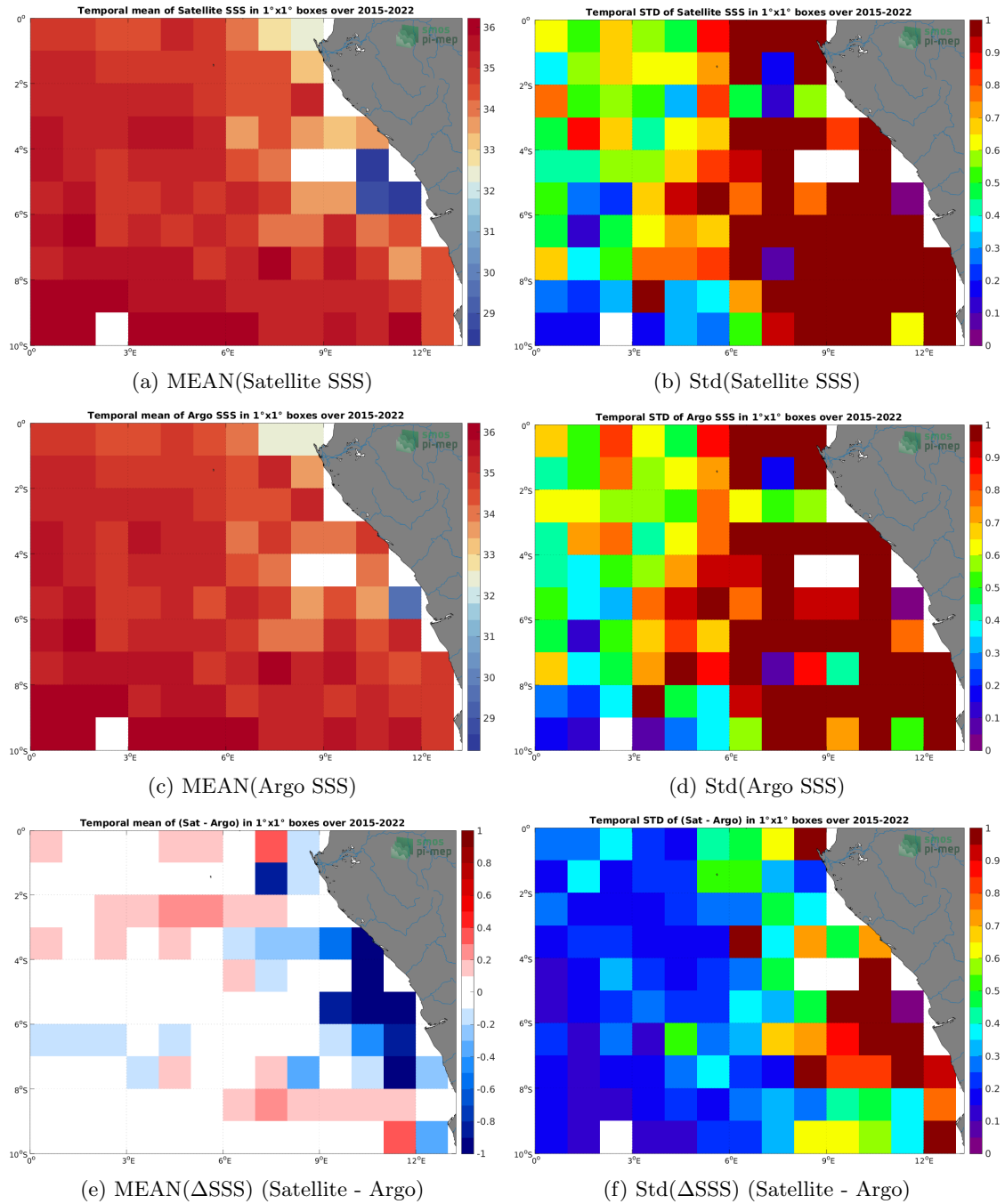
Figure 6: Temporal mean (left) and Std (right) of SSS from SMAP SSS L3 v5 - 8-Day running (RSS) (top), Argo (middle), and of \Delta SSS (Satellite - Argo). Only match-up pairs are used to generate these maps.
