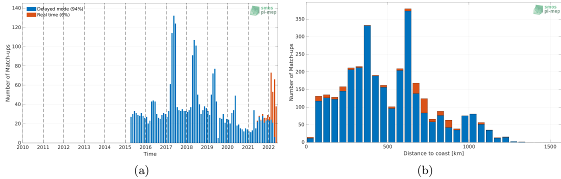
Figure 1: Number of match-ups between Argo and SMAP SSS L3 v5 - 8-Day running (RSS) SSS as a function of time (a) and as function of the distance to coast (b) over the Congo river plume Pi-MEP region and for the full satellite product period.
