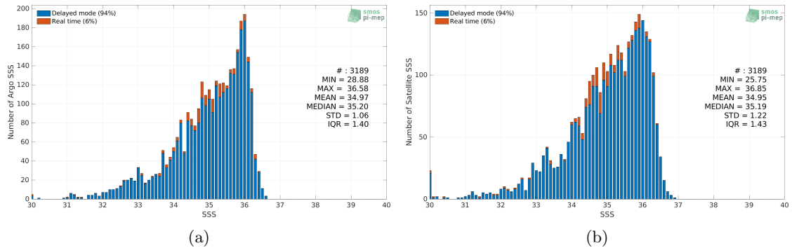
Figure 2: Histograms of SSS from Argo (a) and SMAP SSS L3 v5 - 8-Day running (RSS) (b) considering all match-up pairs per bins of 0.1 over the Congo river plume Pi-MEP region and for the full satellite product period.
