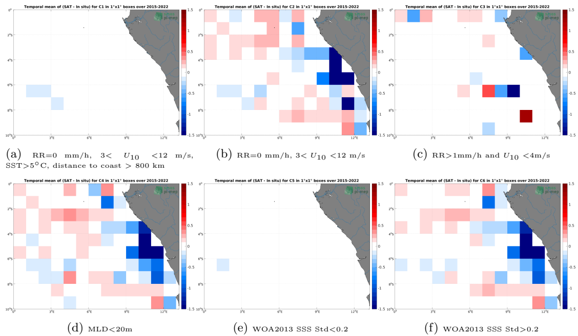
Figure 12: Temporal mean gridded over spatial boxes of size 1^\circ \times 1^\circ of \Delta SSS (SMAP SSS L3 v5 - 8-Day running (RSS) - Argo) for 6 different subdatasets corresponding to:RR=0 mm/h, 3 < U_{10} < 12 m/s, SST >5^\circ\text{C} , distance to coast > 800 km (a), RR=0 mm/h, 3 < U_{10} < 12 m/s (b), RR >1 mm/h and U_{10} < 4 m/s (c),MLD <20 m (d),WOA2013 SSS Std <0.2 (e),WOA2013 SSS Std >0.2 (f).
