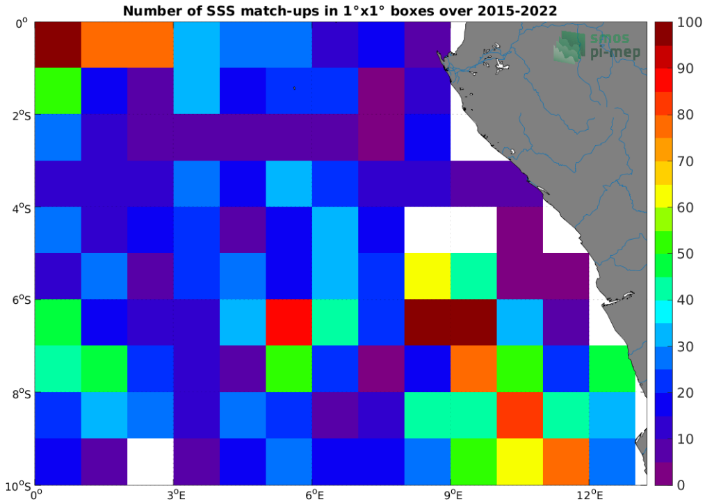
Figure 4: Number of SSS match-ups between Argo SSS and the SMAP SSS L3 v5 - 8-Day running (RSS) SSS product for the Congo river plume Pi-MEP region over 1^\circ \times 1^\circ boxes and for the full satellite product period.
