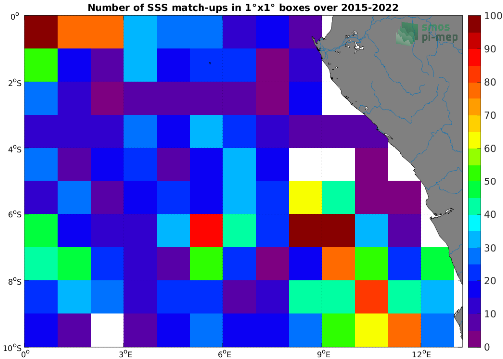
Figure 4: Number of SSS match-ups between Argo SSS and the SMAP SSS L3 v5 - 8-Day running (RSS) SSS product for the Congo river plume Pi-MEP region over 1^{\circ} \times 1^{\circ} boxes and for the full satellite product period.
