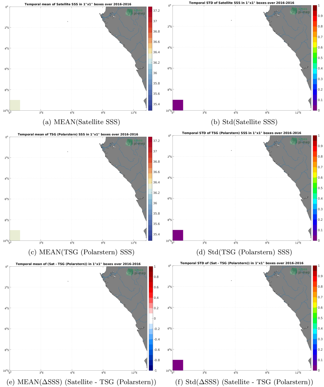
Figure 6: Temporal mean (left) and Std (right) of SSS from SMAP SSS L3 v5 - Monthly (RSS) (top), TSG (Polarstern) (middle), and of \Delta SSS (Satellite - TSG (Polarstern)). Only match-up pairs are used to generate these maps.
