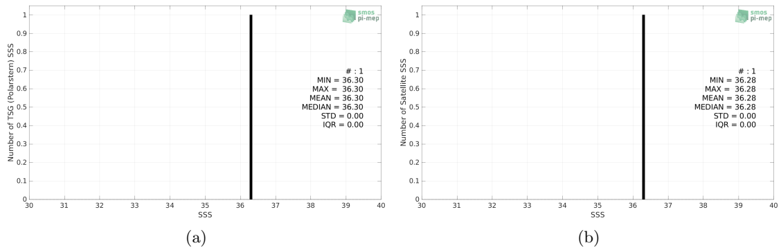
Figure 2: Histograms of SSS from TSG (Polarstern) (a) and SMAP SSS L3 v5 - Monthly (RSS) (b) considering all match-up pairs per bins of 0.1 over the Congo river plume Pi-MEP region and for the full satellite product period.
