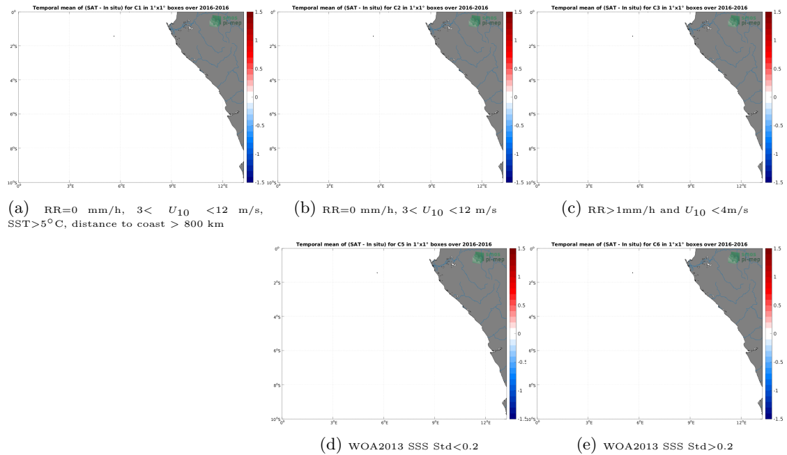
Figure 12: Temporal mean gridded over spatial boxes of size 1^{\circ}\times 1^{\circ} of \Delta\text{SSS} (SMAP SSS L3 v5 - Monthly (RSS) - TSG (Polarstern)) for 5 different subdatasets corresponding to:RR=0 mm/h, 3 < U_{10} < 12 m/s, SST >5^{\circ}\text{C} , distance to coast > 800 km (a), RR=0 mm/h, 3 < U_{10} < 12 m/s (b), RR >1 mm/h and U_{10} < 4 m/s (c), WOA2013 SSS Std <0.2 (d), WOA2013 SSS Std >0.2 (e).
