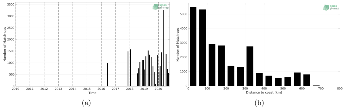
Figure 1: Number of match-ups between TSG (LEGOS-DM) and SMAP SSS L3 v5 - Monthly (RSS) SSS as a function of time (a) and as function of the distance to coast (b) over the Congo river plume Pi-MEP region and for the full satellite product period.
