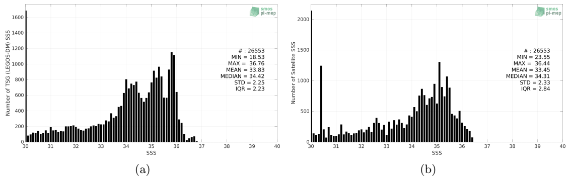
Figure 2: Histograms of SSS from TSG (LEGOS-DM) (a) and SMAP SSS L3 v5 - Monthly (RSS) (b) considering all match-up pairs per bins of 0.1 over the Congo river plume Pi-MEP region and for the full satellite product period.
