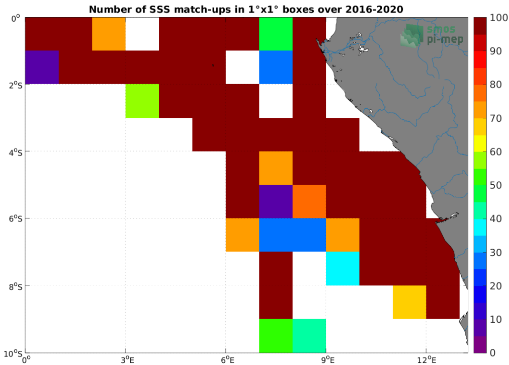
Figure 4: Number of SSS match-ups between TSG (LEGOS-DM) SSS and the SMAP SSS L3 v5 - Monthly (RSS) SSS product for the Congo river plume Pi-MEP region over 1^\circ \times 1^\circ boxes and for the full satellite product period.
