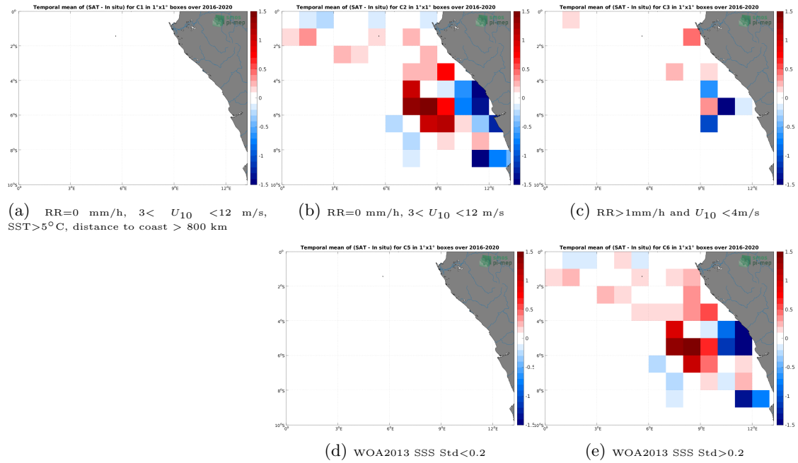
Figure 12: Temporal mean gridded over spatial boxes of size 1^\circ \times 1^\circ of \Delta SSS (SMAP SSS L3 v5 - Monthly (RSS) - TSG (LEGOS-DM)) for 5 different subdatasets corresponding to:RR=0 mm/h, 3 < U_{10} < 12 m/s, SST > 5^\circ C , distance to coast > 800 km (a), RR=0 mm/h, 3 < U_{10} < 12 m/s (b), RR >1 mm/h and U_{10} < 4 m/s (c), WOA2013 SSS Std <0.2 (d), WOA2013 SSS Std >0.2 (e).
