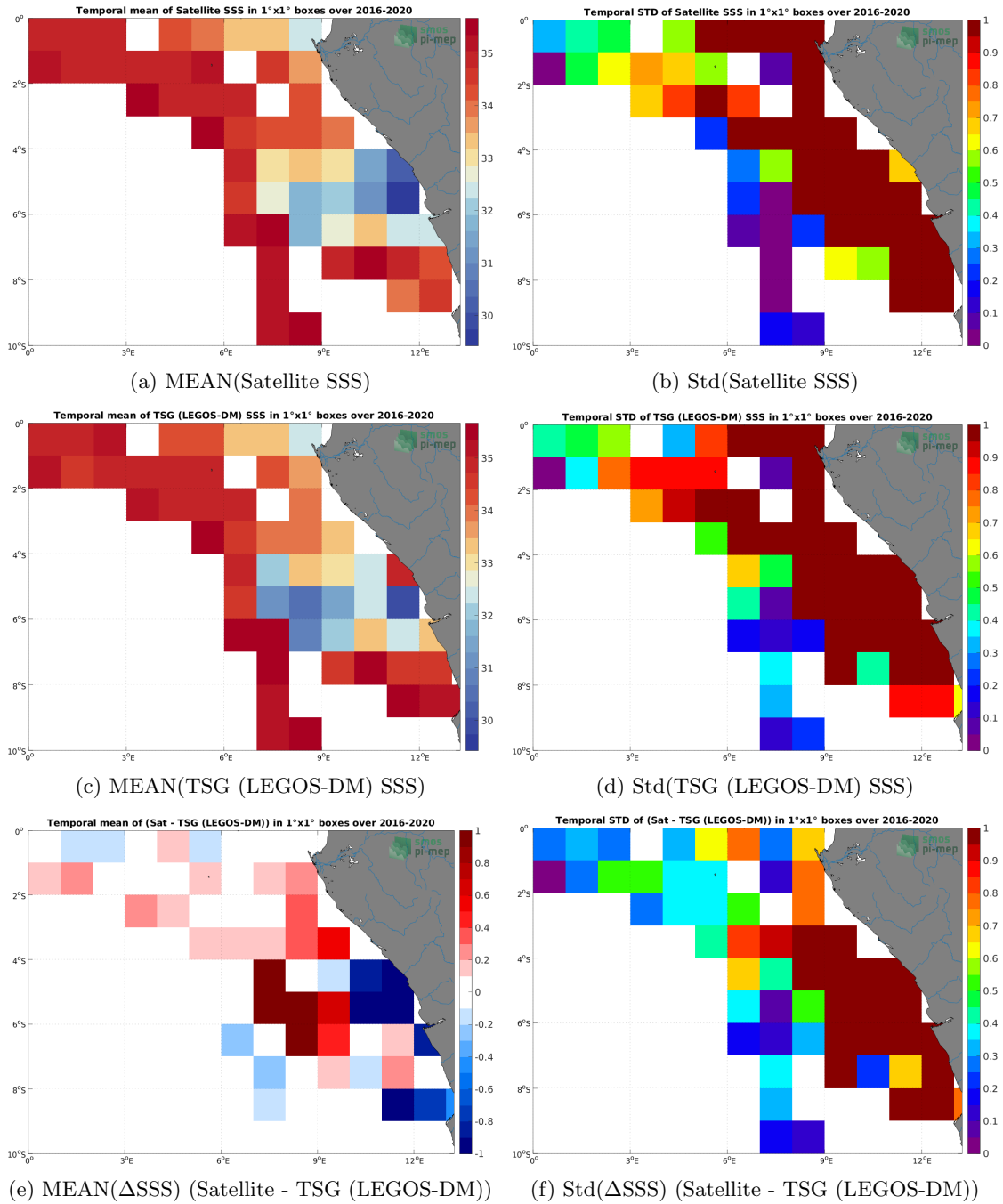
Figure 6: Temporal mean (left) and Std (right) of SSS from SMAP SSS L3 v5 - Monthly (RSS) (top), TSG (LEGOS-DM) (middle), and of \Delta SSS (Satellite - TSG (LEGOS-DM)). Only match-up pairs are used to generate these maps.
