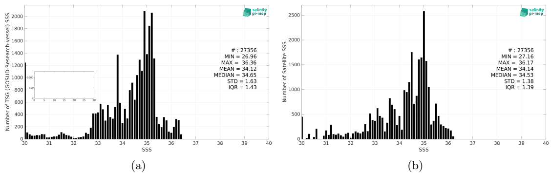
Figure 2: Histograms of SSS from TSG (GOSUD-Research-vessel) (a) and SMAP SSS L3 v5 - Monthly (RSS) (b) considering all match-up pairs per bins of 0.1 over the Congo river plume Pi-MEP region and for the full satellite product period.
