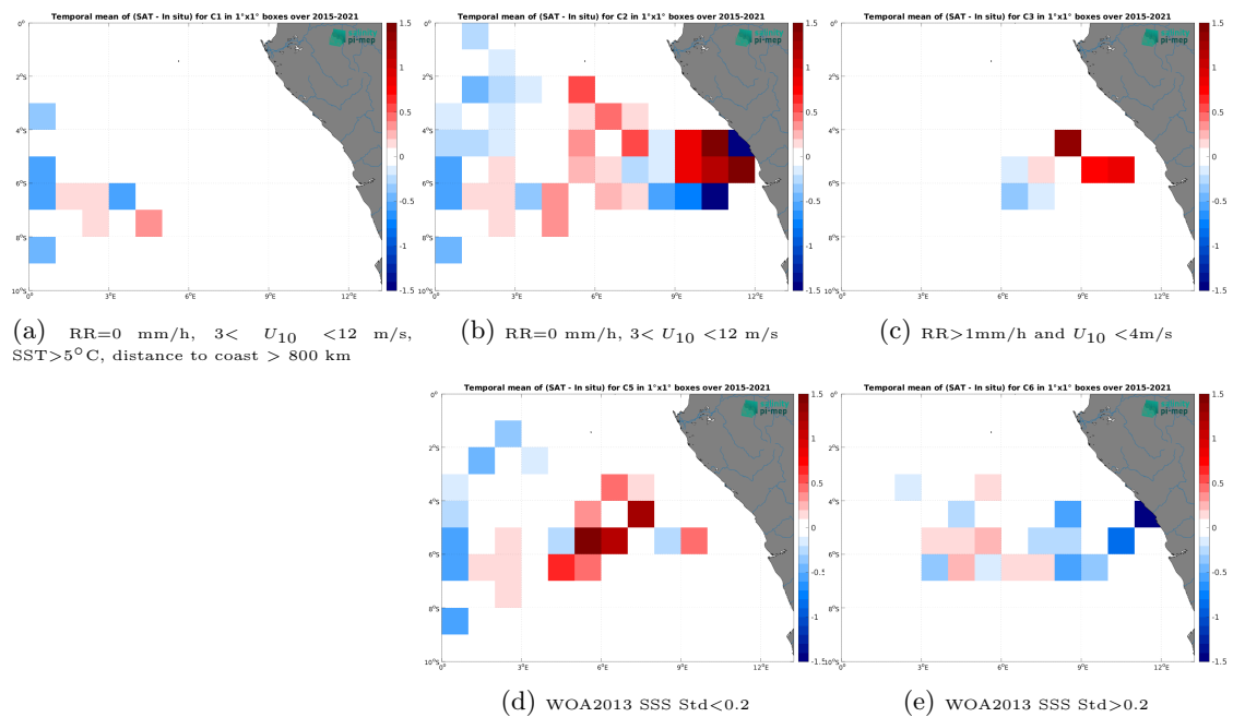
Figure 12: Temporal mean gridded over spatial boxes of size 1^\circ \times 1^\circ of \Delta SSS (SMAP SSS L3 v5 - Monthly (RSS) - TSG (GOSUD-Research-vessel)) for 5 different subdatasets corresponding to:RR=0 mm/h, 3 < U_{10} < 12 m/s, SST>5°C, distance to coast > 800 km (a), RR=0 mm/h, 3 < U_{10} < 12 m/s (b), RR>1mm/h and U_{10} < 4 m/s (c), WOA2013 SSS Std<0.2 (d), WOA2013 SSS Std>0.2 (e).
