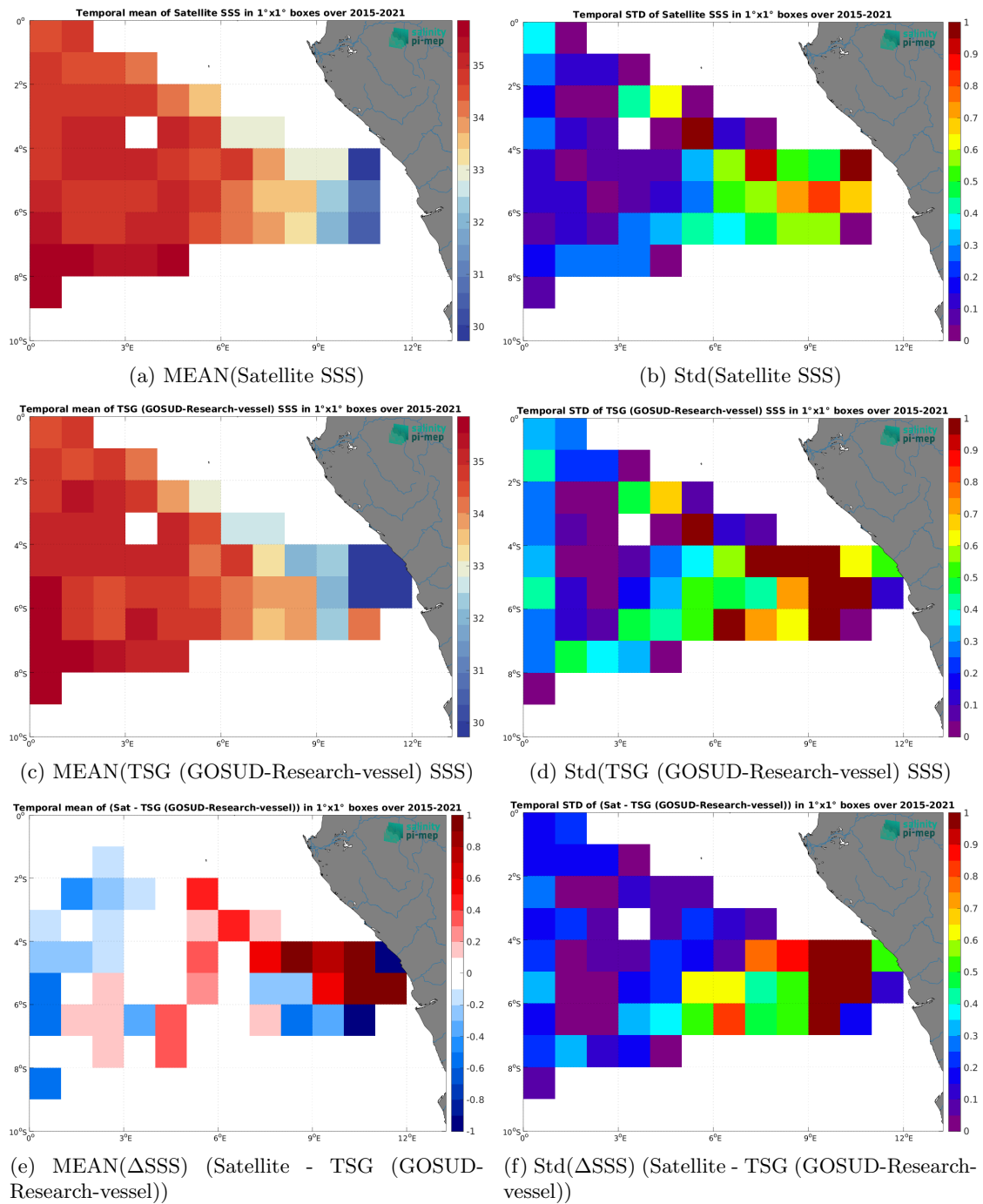
Figure 6: Temporal mean (left) and Std (right) of SSS from SMAP SSS L3 v5 - Monthly (RSS) (top), TSG (GOSUD-Research-vessel) (middle), and of \Delta SSS (Satellite - TSG (GOSUD-Research-vessel)). Only match-up pairs are used to generate these maps.
