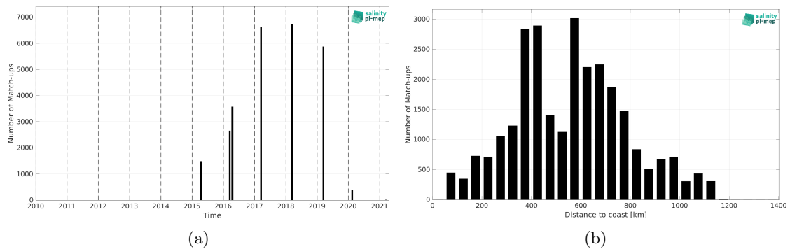
Figure 1: Number of match-ups between TSG (GOSUD-Research-vessel) and SMAP SSS L3 v5 - Monthly (RSS) SSS as a function of time (a) and as function of the distance to coast (b) over the Congo river plume Pi-MEP region and for the full satellite product period.
