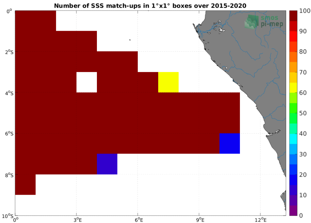
Figure 4: Number of SSS match-ups between TSG (GOSUD-Research-vessel) SSS and the SMAP SSS L3 v5 - Monthly (RSS) SSS product for the Congo river plume Pi-MEP region over 1^\circ \times 1^\circ boxes and for the full satellite product period.
