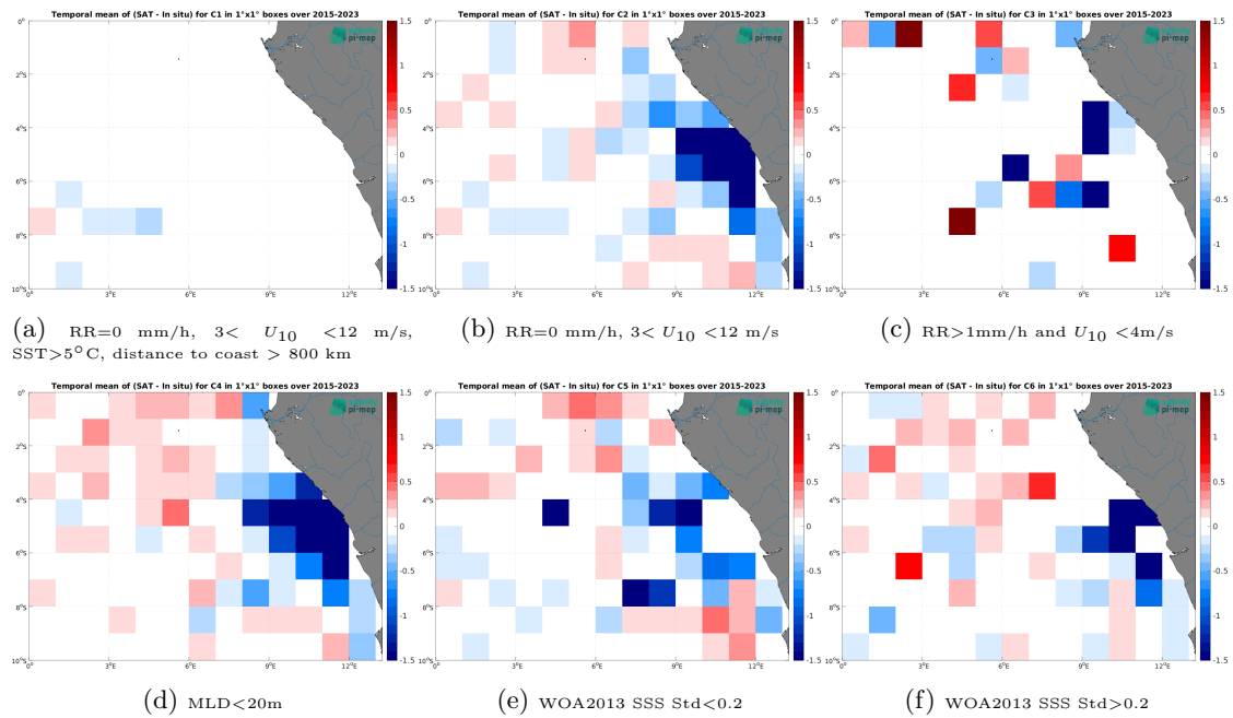
Figure 12: Temporal mean gridded over spatial boxes of size 1^\circ \times 1^\circ of \Delta SSS (SMAP SSS L3 v5 - Monthly (RSS) - Argo) for 6 different subdatasets corresponding to:RR=0 mm/h, 3 < U_{10} < 12 m/s, SST >5^\circ\text{C} , distance to coast > 800 km (a), RR=0 mm/h, 3 < U_{10} < 12 m/s (b), RR >1 mm/h and U_{10} < 4 m/s (c),MLD <20 m (d),WOA2013 SSS Std <0.2 (e),WOA2013 SSS Std >0.2 (f).
