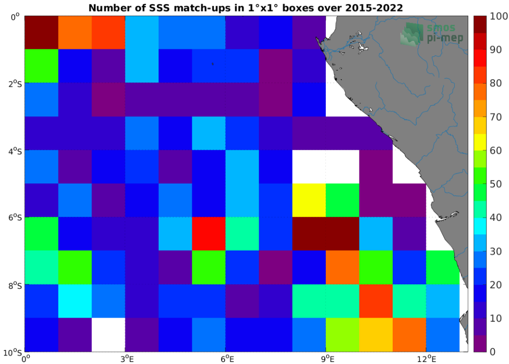
Figure 4: Number of SSS match-ups between Argo SSS and the SMAP SSS L3 v5 - Monthly (RSS) SSS product for the Congo river plume Pi-MEP region over 1^{\circ} \times 1^{\circ} boxes and for the full satellite product period.
