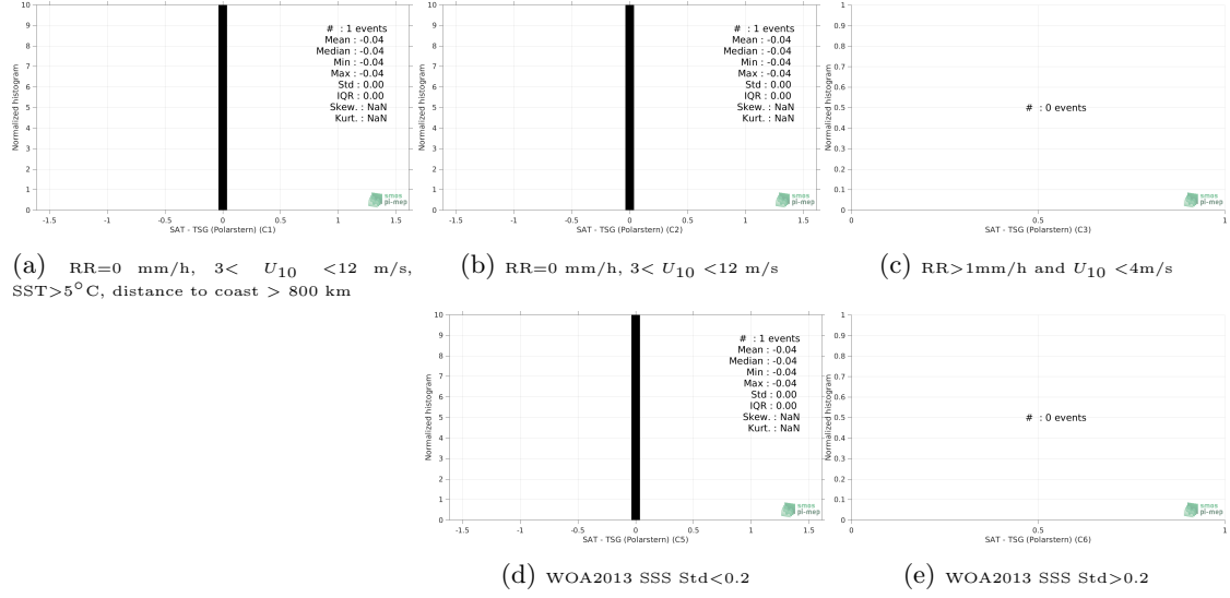
Figure 13: Normalized histogram of \Delta\text{SSS} (SMAP SSS L3 v4 - 8-Day running (RSS) - TSG (Polarstern)) for 5 different subdatasets corresponding to: RR=0 mm/h, 3 < U_{10} < 12 m/s, SST > 5^\circ\text{C} , distance to coast > 800 km (a), RR=0 mm/h, 3 < U_{10} < 12 m/s (b), RR > 1\text{mm/h} and U_{10} < 4\text{m/s} (c), WOA2013 SSS Std < 0.2 (d), WOA2013 SSS Std > 0.2 (e).
