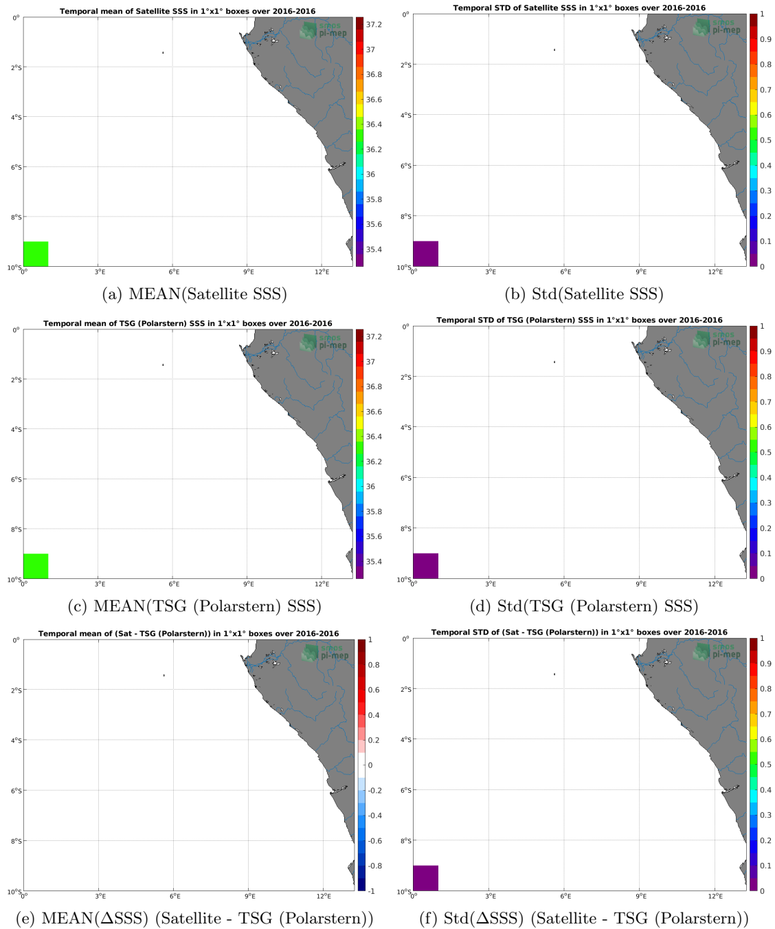
Figure 6: Temporal mean (left) and Std (right) of SSS from SMAP SSS L3 v4 - 8-Day running (RSS) (top), TSG (Polarstern) (middle), and of \Delta SSS (Satellite - TSG (Polarstern)). Only match-up pairs are used to generate these maps.
