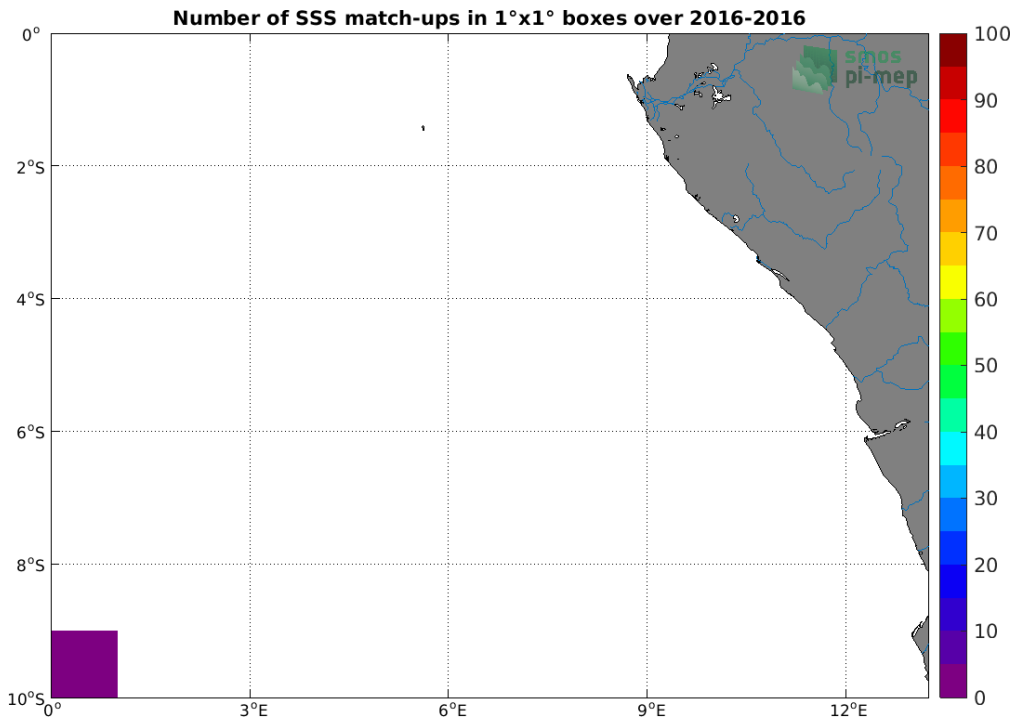
Figure 4: Number of SSS match-ups between TSG (Polarstern) SSS and the SMAP SSS L3 v4 - 8-Day running (RSS) SSS product for the Congo river plume Pi-MEP region over 1°x1° boxes and for the full satellite product period.
