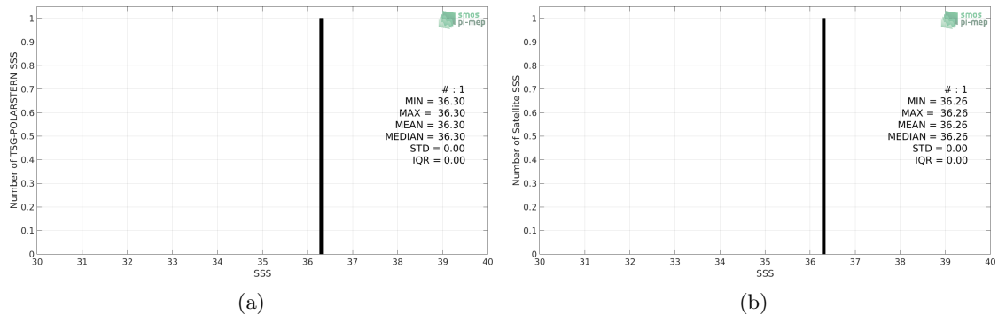
Figure 2: Histograms of SSS from TSG-POLARSTERN (a) and SMAP-L3-RSS-V4-8DAY-RUNNING (b) considering all match-up pairs per bins of 0.1 over the Congo river plume Pi-MEP region and for the full satellite product period.
