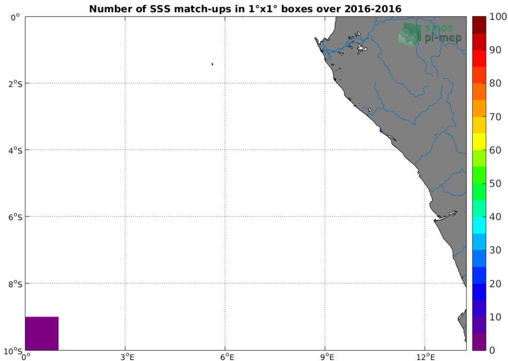
Figure 4: Number of SSS match-ups between TSG-POLARSTERN SSS and the SMAP-L3-RSS-V4-8DAY-RUNNING SSS product for the Congo river plume Pi-MEP region over 1^{\circ} \times 1^{\circ} boxes and for the full satellite product period.
