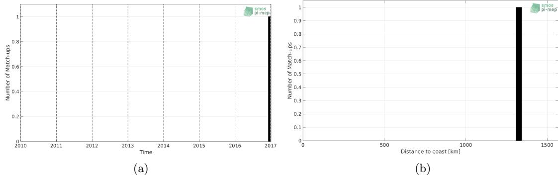
Figure 1: Number of match-ups between TSG-POLARSTERN and SMAP-L3-RSS-V4-8DAY-RUNNING SSS as a function of time (a) and as function of the distance to coast (b) over the Congo river plume Pi-MEP region and for the full satellite product period.
