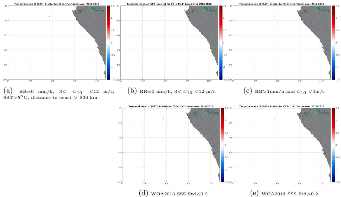
Figure 12: Temporal mean gridded over spatial boxes of size 1^{\circ}\times 1^{\circ} of \Delta\text{SSS} (SMAP-L3-RSS-V4-8DAY-RUNNING - TSG-POLARSTERN) for 5 different subdatasets corresponding to:RR=0 mm/h, 3 < U_{10} < 12 m/s, SST >5^{\circ}\text{C} , distance to coast > 800 km (a), RR=0 mm/h, 3 < U_{10} < 12 m/s (b), RR >1 mm/h and U_{10} < 4 m/s (c), WOA2013 SSS Std <0.2 (d), WOA2013 SSS Std >0.2 (e).
