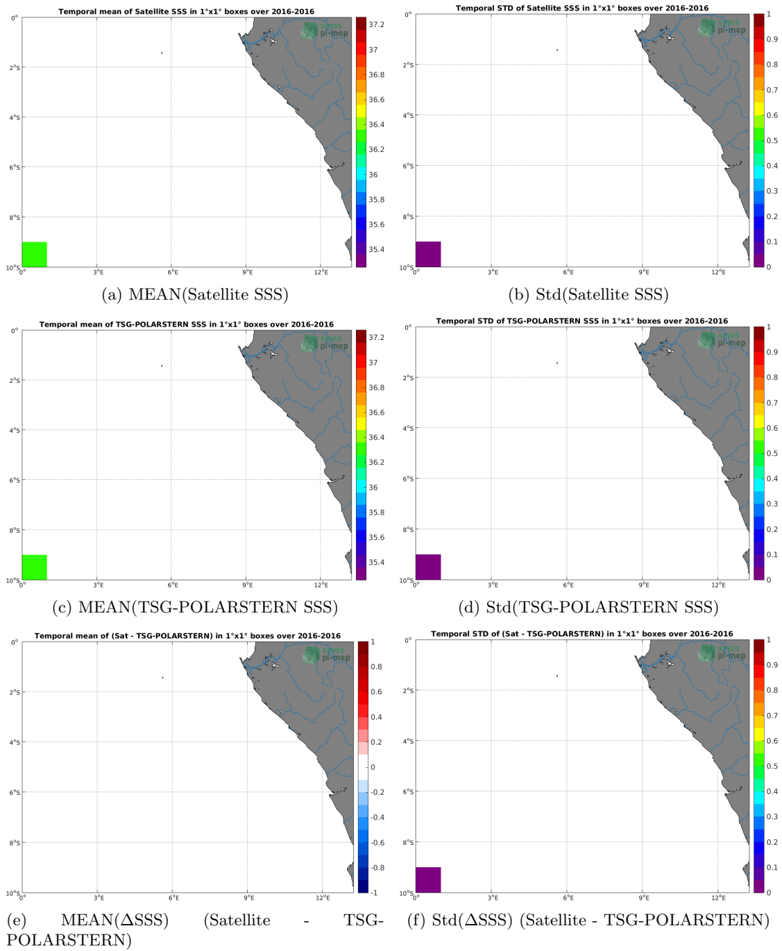
Figure 6: Temporal mean (left) and Std (right) of SSS from SMAP-L3-RSS-V4-8DAY-RUNNING (top), TSG-POLARSTERN (middle), and of \Delta SSS (Satellite - TSG-POLARSTERN). Only match-up pairs are used to generate these maps.
