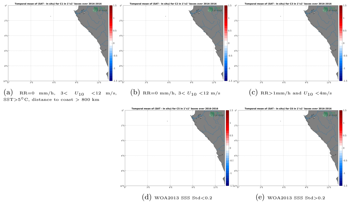
Figure 12: Temporal mean gridded over spatial boxes of size 1^\circ \times 1^\circ of \Delta SSS (SMAP-L3-RSS-V4-8DAY-RUNNING - TSG-POLARSTERN) for 5 different subdatasets corresponding to:RR=0 mm/h, 3 < U_{10} < 12 m/s, SST > 5^\circ\text{C} , distance to coast > 800 km (a), RR=0 mm/h, 3 < U_{10} < 12 m/s (b), RR > 1 mm/h and U_{10} < 4 m/s (c), WOA2013 SSS Std < 0.2 (d), WOA2013 SSS Std > 0.2 (e).
