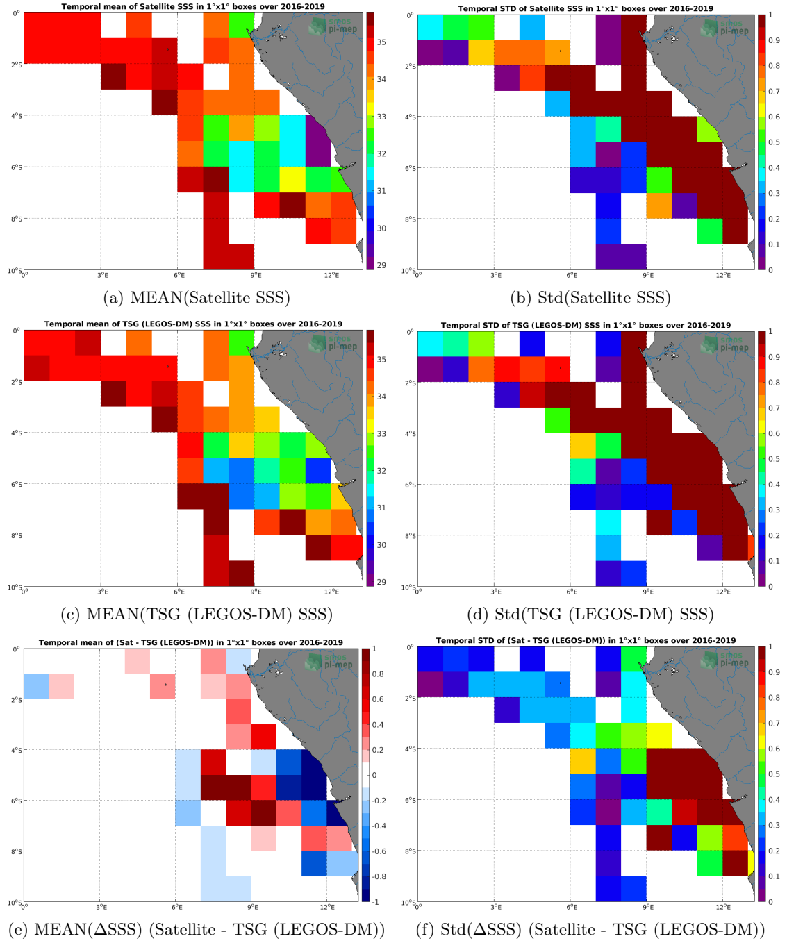
Figure 6: Temporal mean (left) and Std (right) of SSS from SMAP SSS L3 v4 - 8-Day running (RSS) (top), TSG (LEGOS-DM) (middle), and of \Delta SSS (Satellite - TSG (LEGOS-DM)). Only match-up pairs are used to generate these maps.
