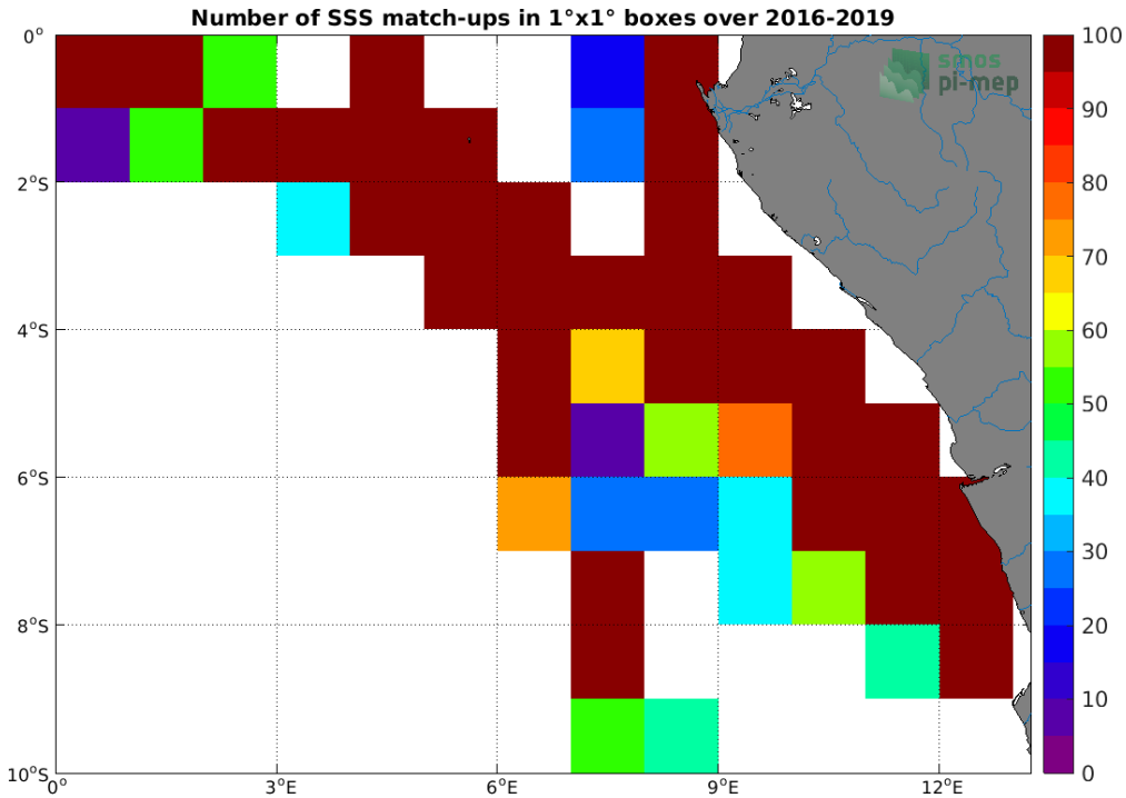
Figure 4: Number of SSS match-ups between TSG (LEGOS-DM) SSS and the SMAP SSS L3 v4 - 8-Day running (RSS) SSS product for the Congo river plume Pi-MEP region over 1°x1° boxes and for the full satellite product period.
