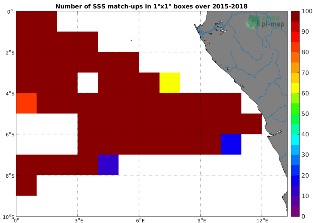
Figure 4: Number of SSS match-ups between TSG-GOSUD-Research-vessel SSS and the SMAP-L3-RSS-V4-8DAY-RUNNING SSS product for the Congo river plume Pi-MEP region over 1°x1° boxes and for the full satellite product period.
