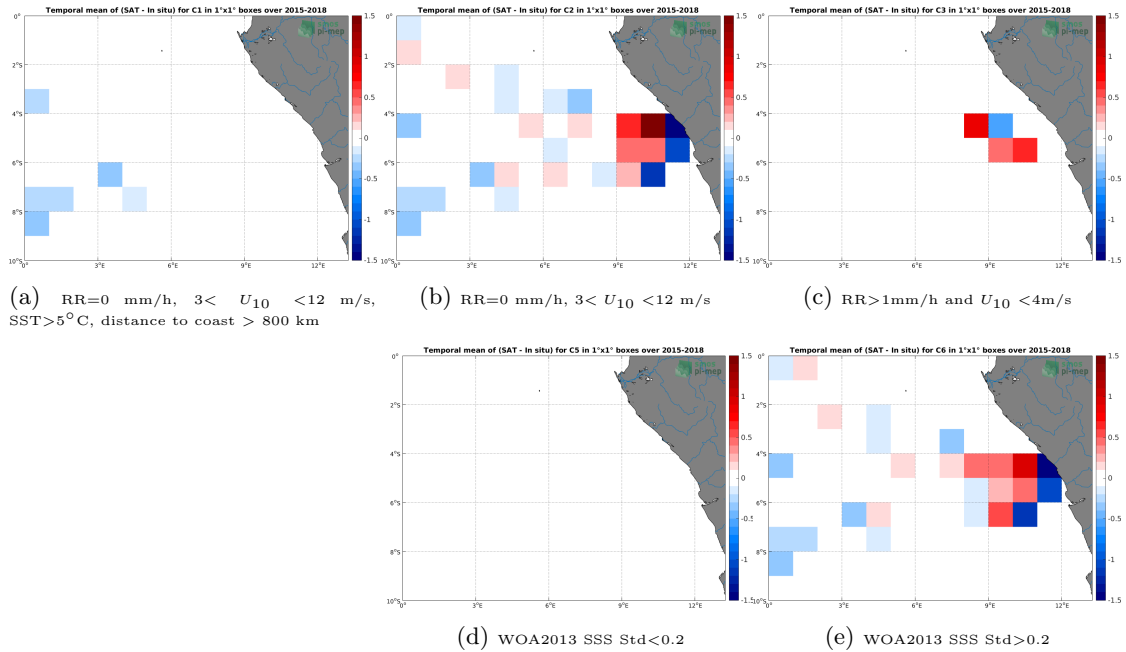
Figure 12: Temporal mean gridded over spatial boxes of size 1^\circ \times 1^\circ of \Delta SSS (SMAP-L3-RSS-V4-8DAY-RUNNING - TSG-GOSUD-Research-vessel) for 5 different subdatasets corresponding to: RR=0 mm/h, 3 < U_{10} < 12 m/s, SST > 5°C, distance to coast > 800 km (a), RR=0 mm/h, 3 < U_{10} < 12 m/s (b), RR > 1mm/h and U_{10} < 4 m/s (c), WOA2013 SSS Std < 0.2 (d), WOA2013 SSS Std > 0.2 (e).
