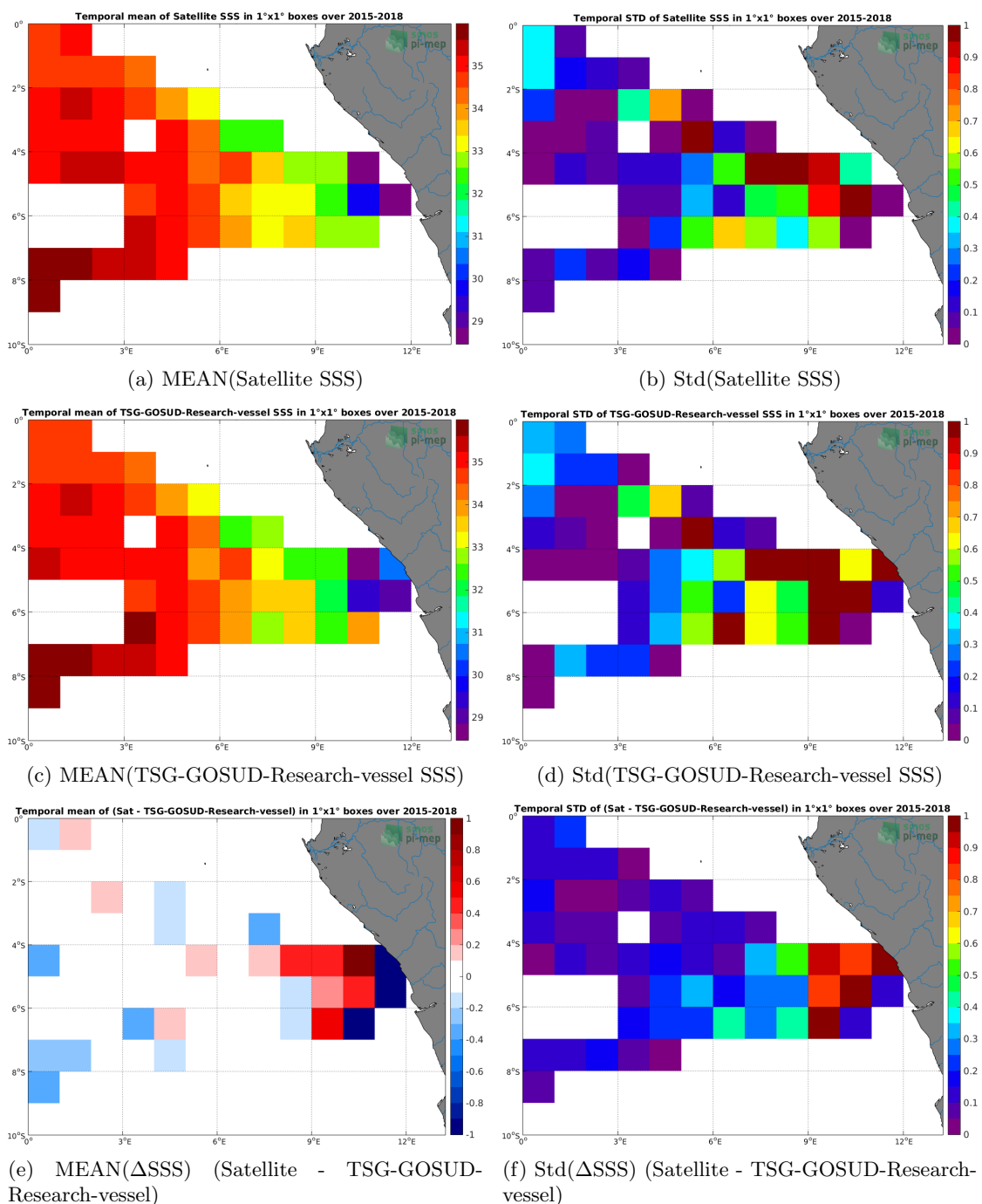
Figure 6: Temporal mean (left) and Std (right) of SSS from SMAP-L3-RSS-V4-8DAY-RUNNING (top), TSG-GOSUD-Research-vessel (middle), and of \Delta SSS (Satellite - TSG-GOSUD-Research-vessel). Only match-up pairs are used to generate these maps.
