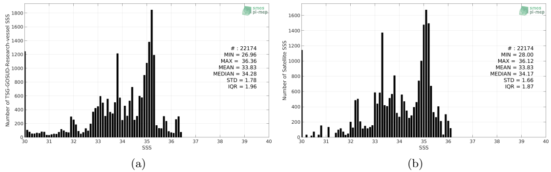
Figure 2: Histograms of SSS from TSG-GOSUD-Research-vessel (a) and SMAP-L3-RSS-V4-8DAY-RUNNING (b) considering all match-up pairs per bins of 0.1 over the Congo river plume Pi-MEP region and for the full satellite product period.
