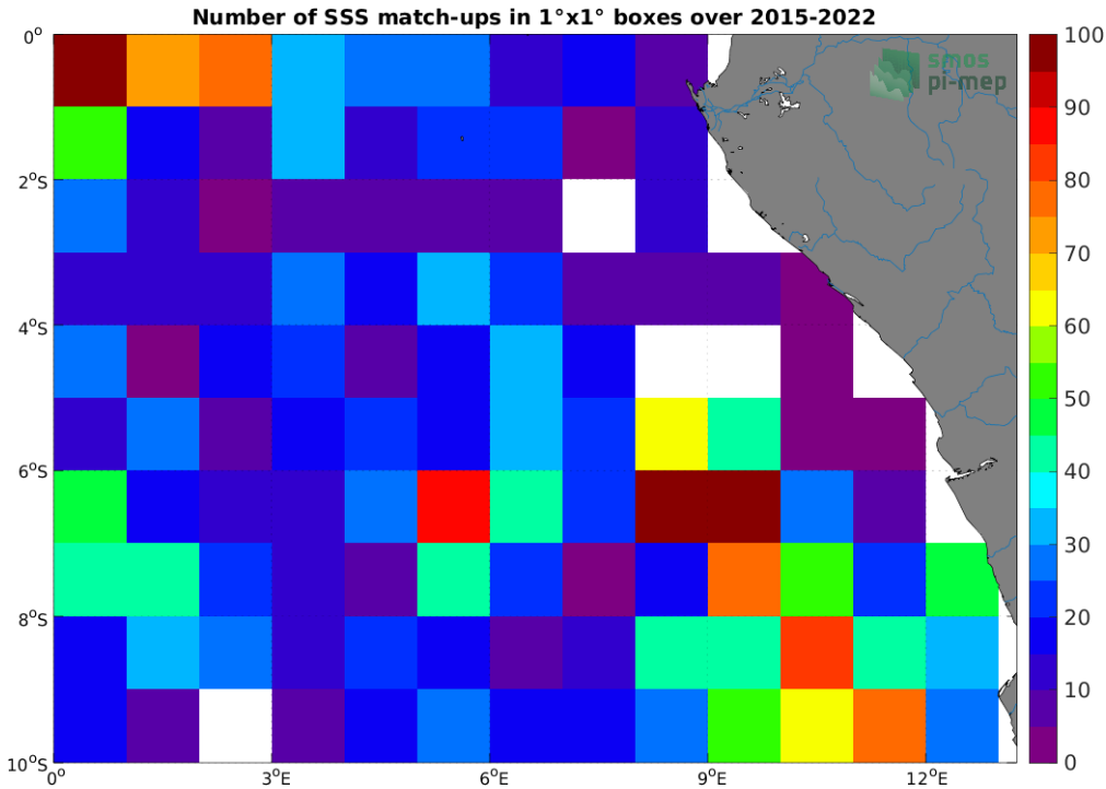
Figure 4: Number of SSS match-ups between Argo SSS and the SMAP SSS L3 v4 - 8-Day running (RSS) SSS product for the Congo river plume Pi-MEP region over 1°x1° boxes and for the full satellite product period.
