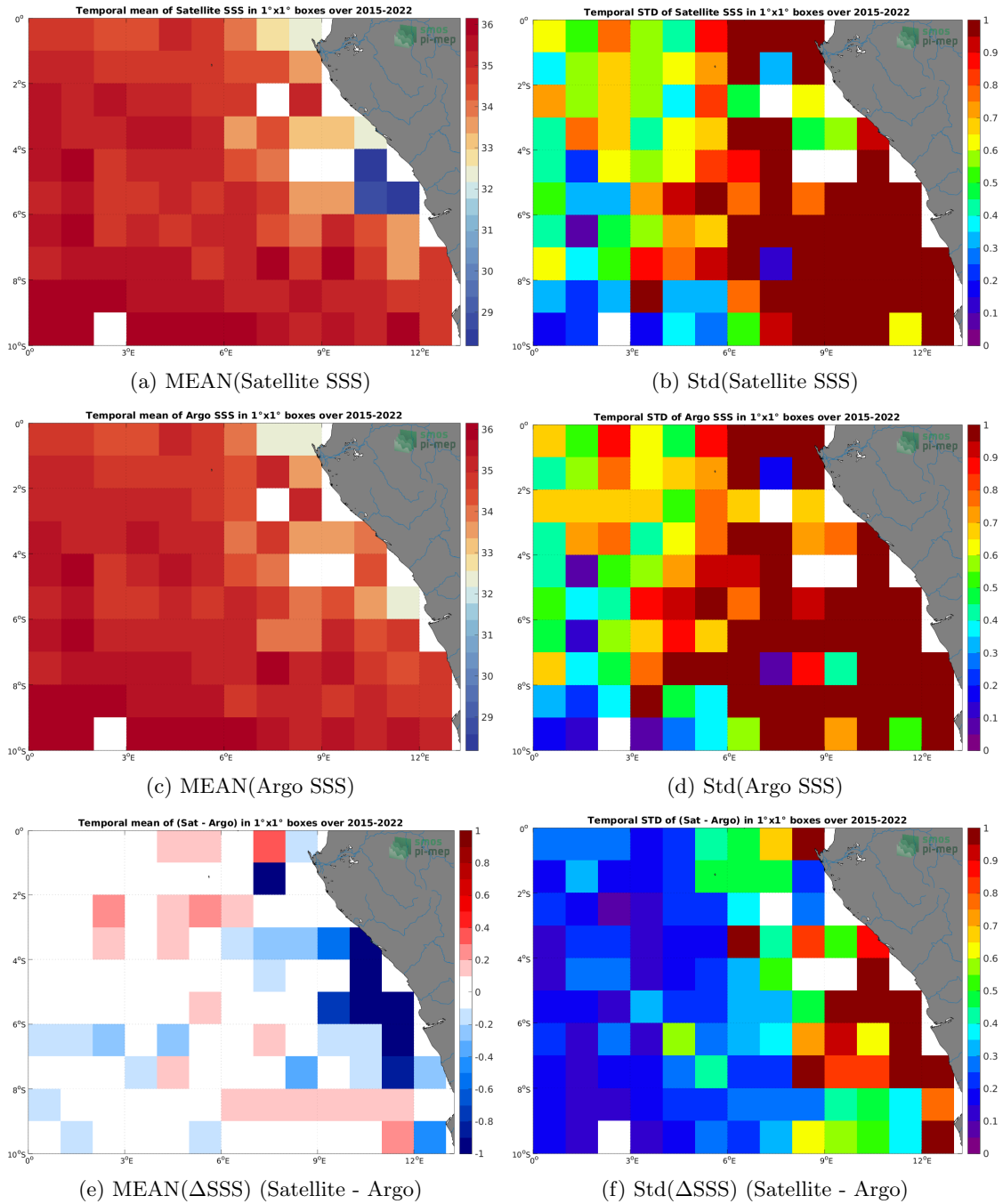
Figure 6: Temporal mean (left) and Std (right) of SSS from SMAP SSS L3 v4 - 8-Day running (RSS) (top), Argo (middle), and of \Delta SSS (Satellite - Argo). Only match-up pairs are used to generate these maps.
