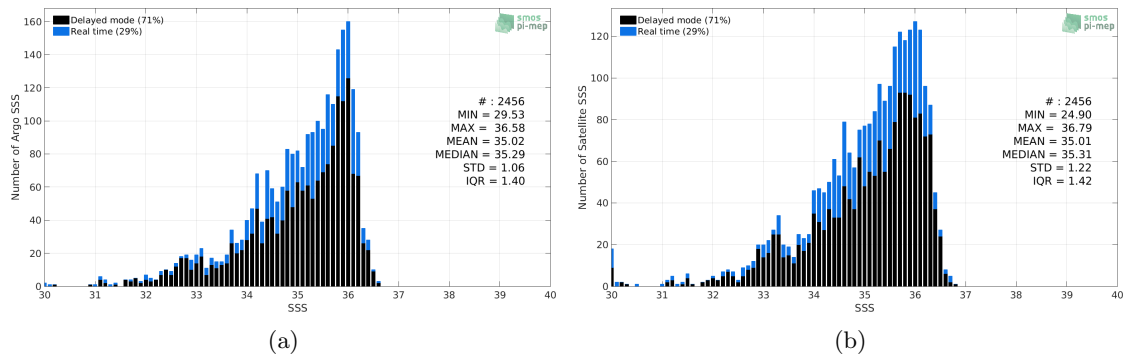
Figure 2: Histograms of SSS from Argo (a) and SMAP-L3-RSS-V4-8DAY-RUNNING (b) considering all match-up pairs per bins of 0.1 over the Congo river plume Pi-MEP region and for the full satellite product period.
