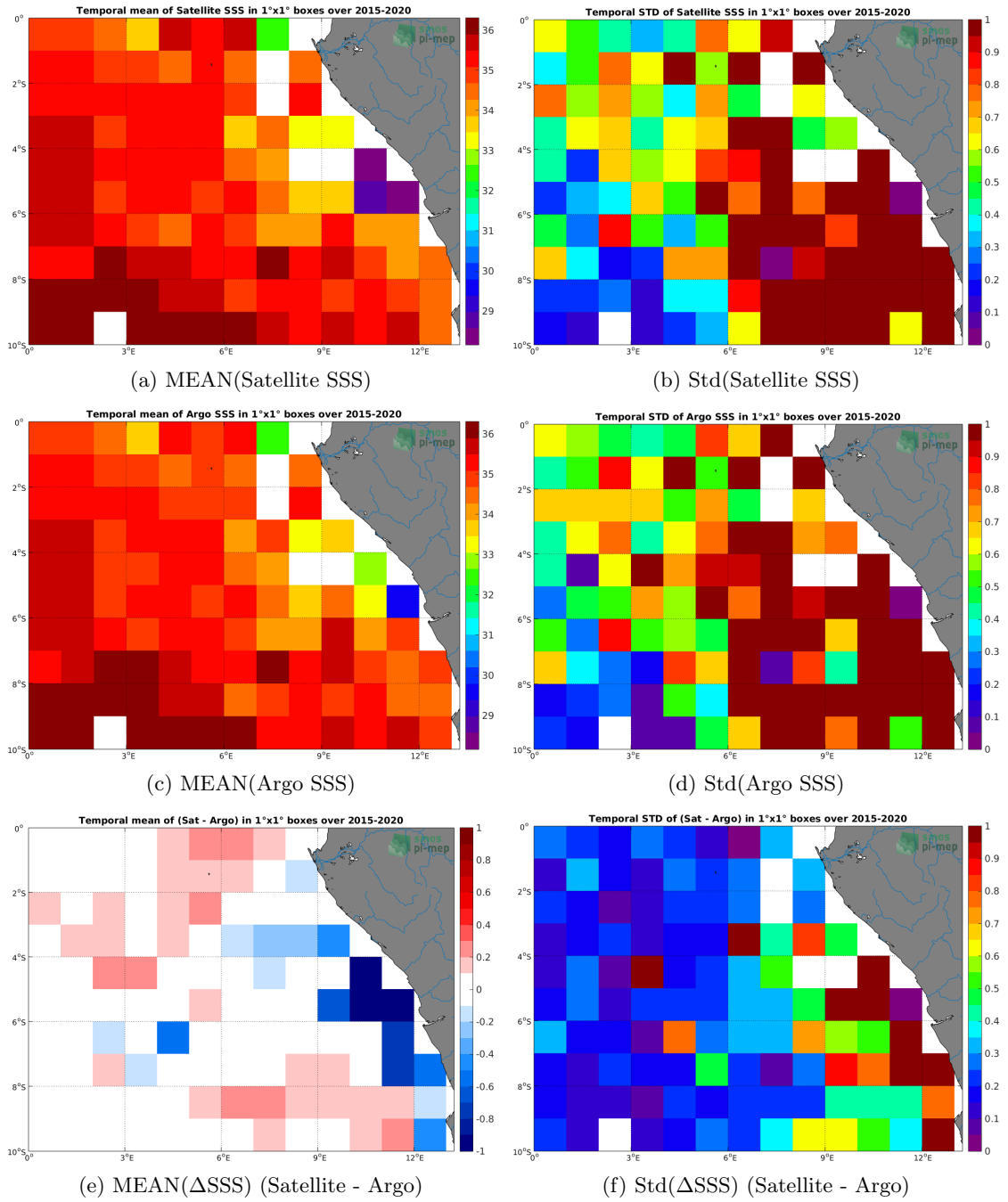
Figure 6: Temporal mean (left) and Std (right) of SSS from SMAP-L3-RSS-V4-8DAY-RUNNING (top), Argo (middle), and of \Delta SSS (Satellite - Argo). Only match-up pairs are used to generate these maps.
