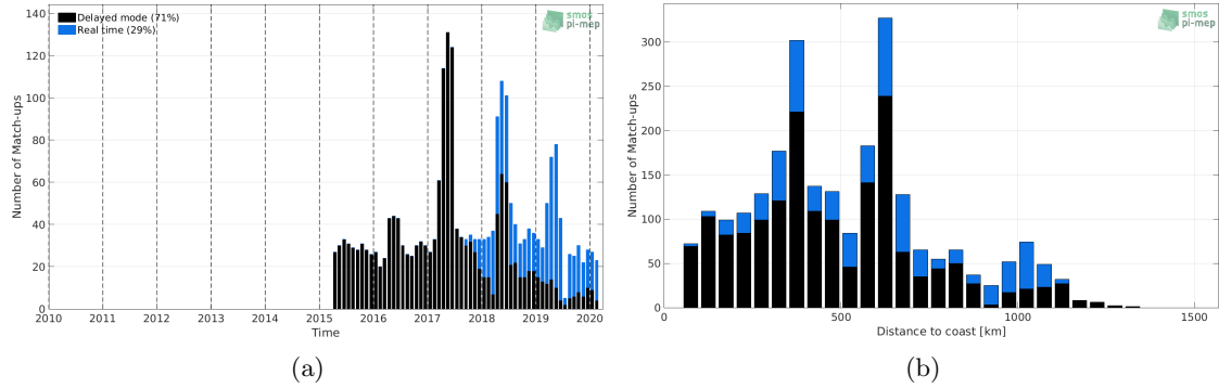
Figure 1: Number of match-ups between Argo and SMAP-L3-RSS-V4-8DAY-RUNNING SSS as a function of time (a) and as function of the distance to coast (b) over the Congo river plume Pi-MEP region and for the full satellite product period.
