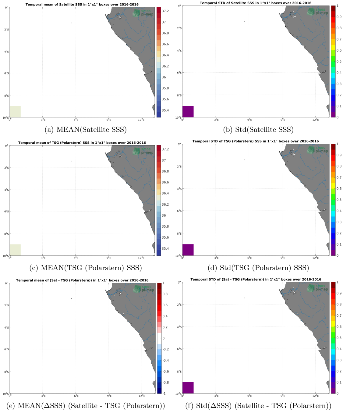
Figure 6: Temporal mean (left) and Std (right) of SSS from SMAP SSS L3 v4 - Monthly (RSS) (top), TSG (Polarstern) (middle), and of \Delta SSS (Satellite - TSG (Polarstern)). Only match-up pairs are used to generate these maps.
