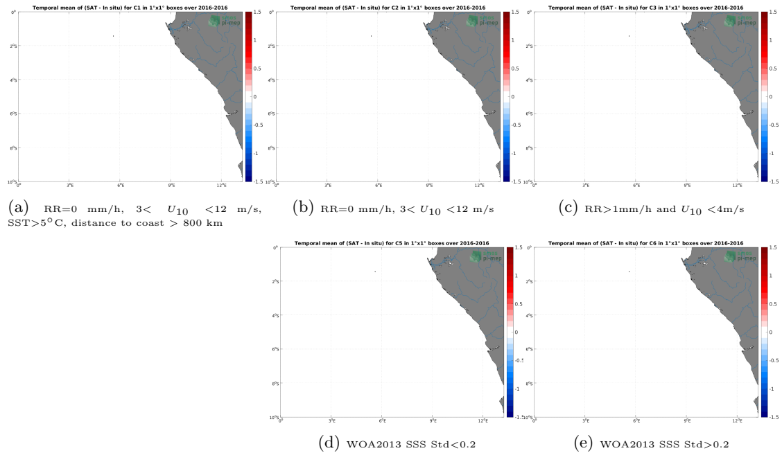
Figure 12: Temporal mean gridded over spatial boxes of size 1^{\circ}\times 1^{\circ} of \Delta\text{SSS} (SMAP SSS L3 v4 - Monthly (RSS) - TSG (Polarstern)) for 5 different subdatasets corresponding to:RR=0 mm/h, 3 < U_{10} < 12 m/s, SST >5^{\circ}\text{C} , distance to coast > 800 km (a), RR=0 mm/h, 3 < U_{10} < 12 m/s (b), RR >1 mm/h and U_{10} < 4 m/s (c), WOA2013 SSS Std <0.2 (d), WOA2013 SSS Std >0.2 (e).
