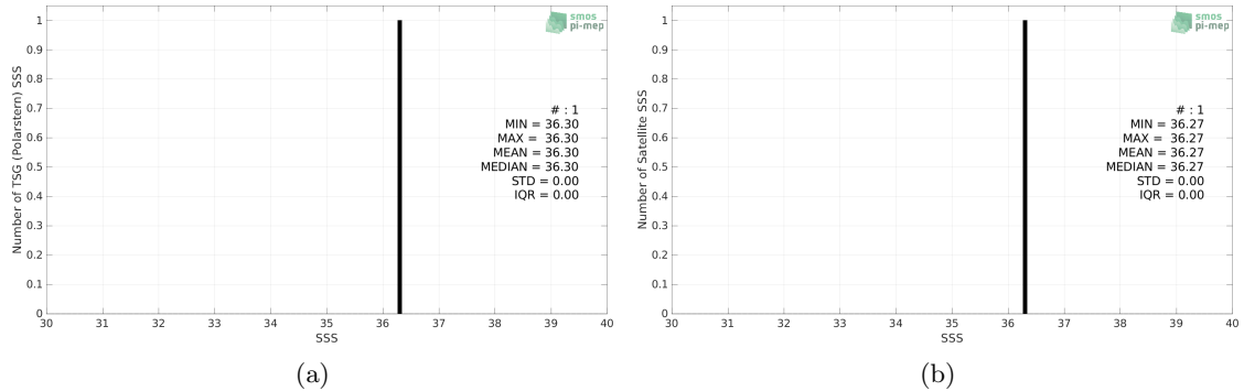
Figure 2: Histograms of SSS from TSG (Polarstern) (a) and SMAP SSS L3 v4 - Monthly (RSS) (b) considering all match-up pairs per bins of 0.1 over the Congo river plume Pi-MEP region and for the full satellite product period.
