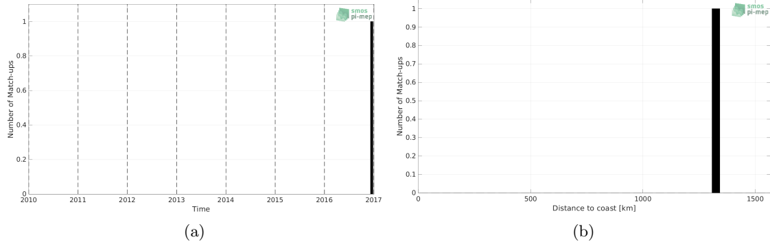
Figure 1: Number of match-ups between TSG (Polarstern) and SMAP SSS L3 v4 - Monthly (RSS) SSS as a function of time (a) and as function of the distance to coast (b) over the Congo river plume Pi-MEP region and for the full satellite product period.
