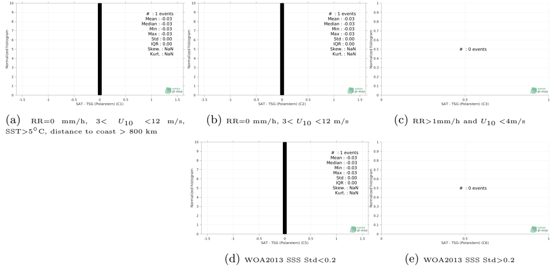
Figure 13: Normalized histogram of \Delta\text{SSS} (SMAP SSS L3 v4 - Monthly (RSS) - TSG (Polarstern)) for 5 different subdatasets corresponding to: RR=0 mm/h, 3 < U_{10} < 12 m/s, SST > 5^\circ\text{C} , distance to coast > 800 km (a), RR=0 mm/h, 3 < U_{10} < 12 m/s (b), RR > 1\text{mm/h} and U_{10} < 4\text{m/s} (c), WOA2013 SSS Std < 0.2 (d), WOA2013 SSS Std > 0.2 (e).
