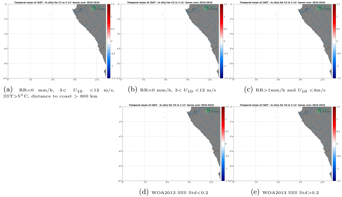
Figure 12: Temporal mean gridded over spatial boxes of size 1^{\circ}\times 1^{\circ} of \Delta\text{SSS} (SMAP-L3-RSS-V4-MONTHLY - TSG-POLARSTERN) for 5 different subdatasets corresponding to:RR=0 mm/h, 3 < U_{10} < 12 m/s, SST >5^{\circ}\text{C} , distance to coast > 800 km (a), RR=0 mm/h, 3 < U_{10} < 12 m/s (b), RR >1 mm/h and U_{10} < 4 m/s (c), WOA2013 SSS Std <0.2 (d), WOA2013 SSS Std >0.2 (e).
