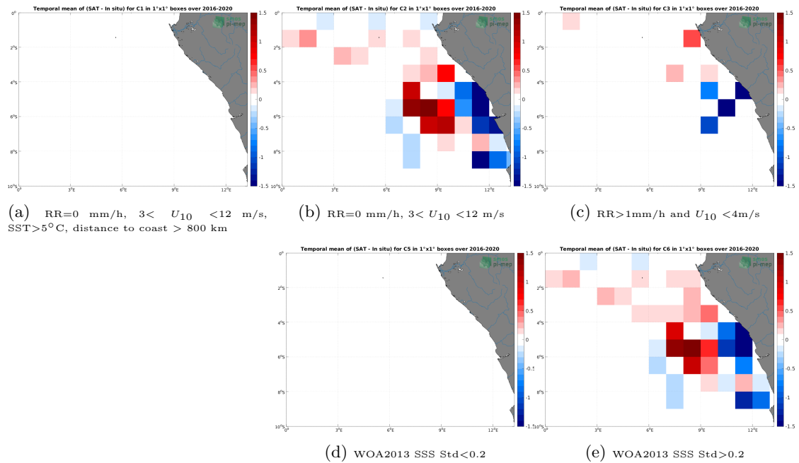
Figure 12: Temporal mean gridded over spatial boxes of size 1^\circ \times 1^\circ of \Delta SSS (SMAP SSS L3 v4 - Monthly (RSS) - TSG (LEGOS-DM)) for 5 different subdatasets corresponding to:RR=0 mm/h, 3 < U_{10} < 12 m/s, SST > 5^\circ\text{C} , distance to coast > 800 km (a), RR=0 mm/h, 3 < U_{10} < 12 m/s (b), RR > 1 mm/h and U_{10} < 4 m/s (c), WOA2013 SSS Std < 0.2 (d), WOA2013 SSS Std > 0.2 (e).
