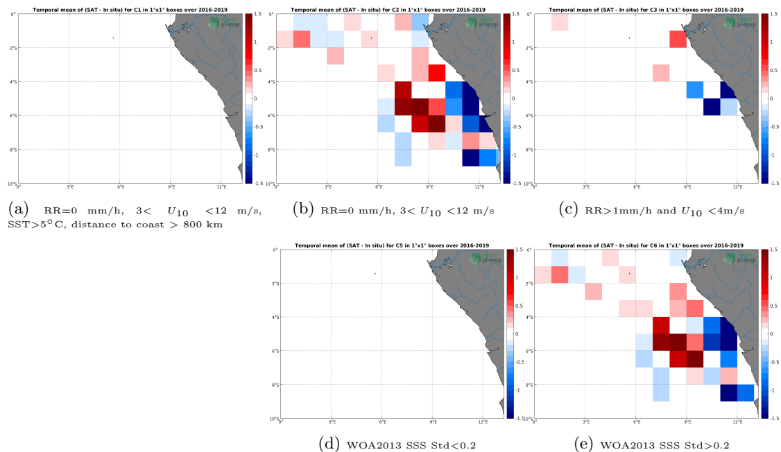
Figure 12: Temporal mean gridded over spatial boxes of size 1^\circ \times 1^\circ of \Delta\text{SSS} (SMAP SSS L3 v4 - Monthly (RSS) - TSG (LEGOS-DM)) for 5 different subdatasets corresponding to:RR=0 mm/h, 3 < U_{10} < 12 m/s, SST > 5^\circ\text{C} , distance to coast > 800 km (a), RR=0 mm/h, 3 < U_{10} < 12 m/s (b), RR > 1 mm/h and U_{10} < 4 m/s (c), WOA2013 SSS Std < 0.2 (d), WOA2013 SSS Std > 0.2 (e).
