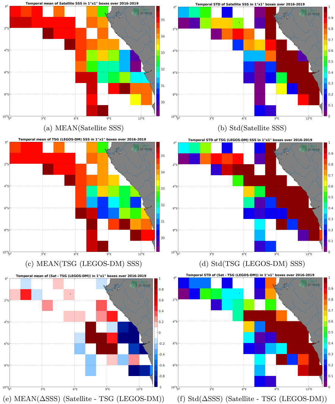
Figure 6: Temporal mean (left) and Std (right) of SSS from SMAP SSS L3 v4 - Monthly (RSS) (top), TSG (LEGOS-DM) (middle), and of \Delta SSS (Satellite - TSG (LEGOS-DM)). Only match-up pairs are used to generate these maps.
