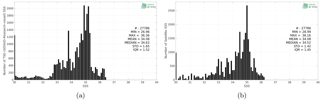
Figure 2: Histograms of SSS from TSG (GOSUD-Research-vessel) (a) and SMAP SSS L3 v4 - Monthly (RSS) (b) considering all match-up pairs per bins of 0.1 over the Congo river plume Pi-MEP region and for the full satellite product period.
