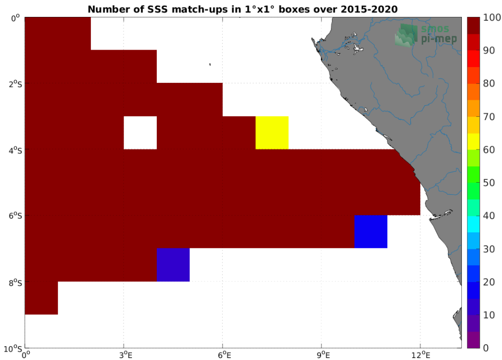
Figure 4: Number of SSS match-ups between TSG (GOSUD-Research-vessel) SSS and the SMAP SSS L3 v4 - Monthly (RSS) SSS product for the Congo river plume Pi-MEP region over 1^{\circ} \times 1^{\circ} boxes and for the full satellite product period.
